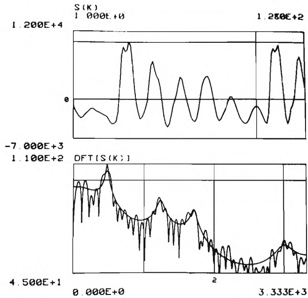
Figure 4-1: Example frame used as s(k) a) 128 samples of the vowel /ə/, sampled at 6667. Hz b) Spectrum of /ə/ and a 10 pole LPC fit to that spectrum
