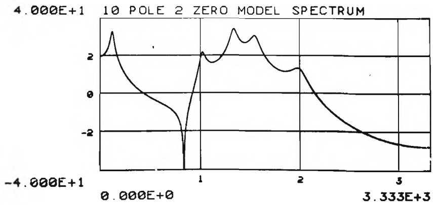
Figure 4-7: 10 Pole, 2 Zero Model Spectrum to be identified
