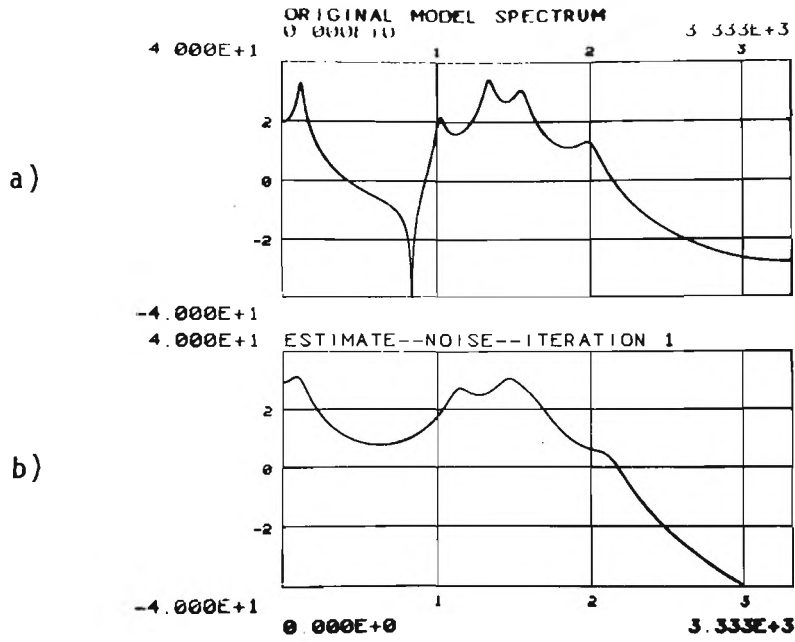
Figure 4-16: Noise Excitation a) Model spectrum b) Estimate of model spectrum after 1 iteration
