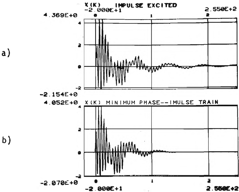
Figure 4-12: Impulse Train Excitation a) Output of model with an impulse input b) Modified system output after cepstral modifications to remove periodicity and simulate a minimum phase signal.
