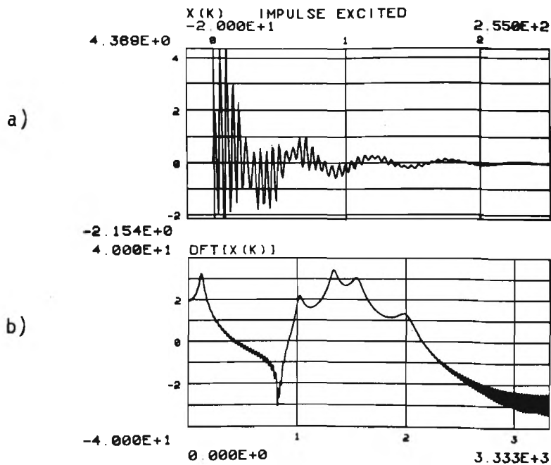
Figure 4-8: Impulse Excitation a) Output of model b) Spectrum of part a)
