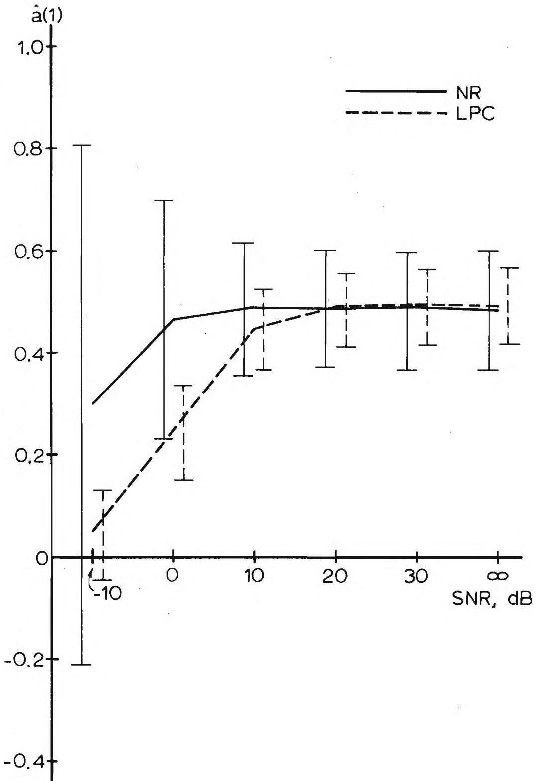
Figure 4-23: NR and LPC estimates of a(1) in AR+N tests, shown with \pm \sigma limits
