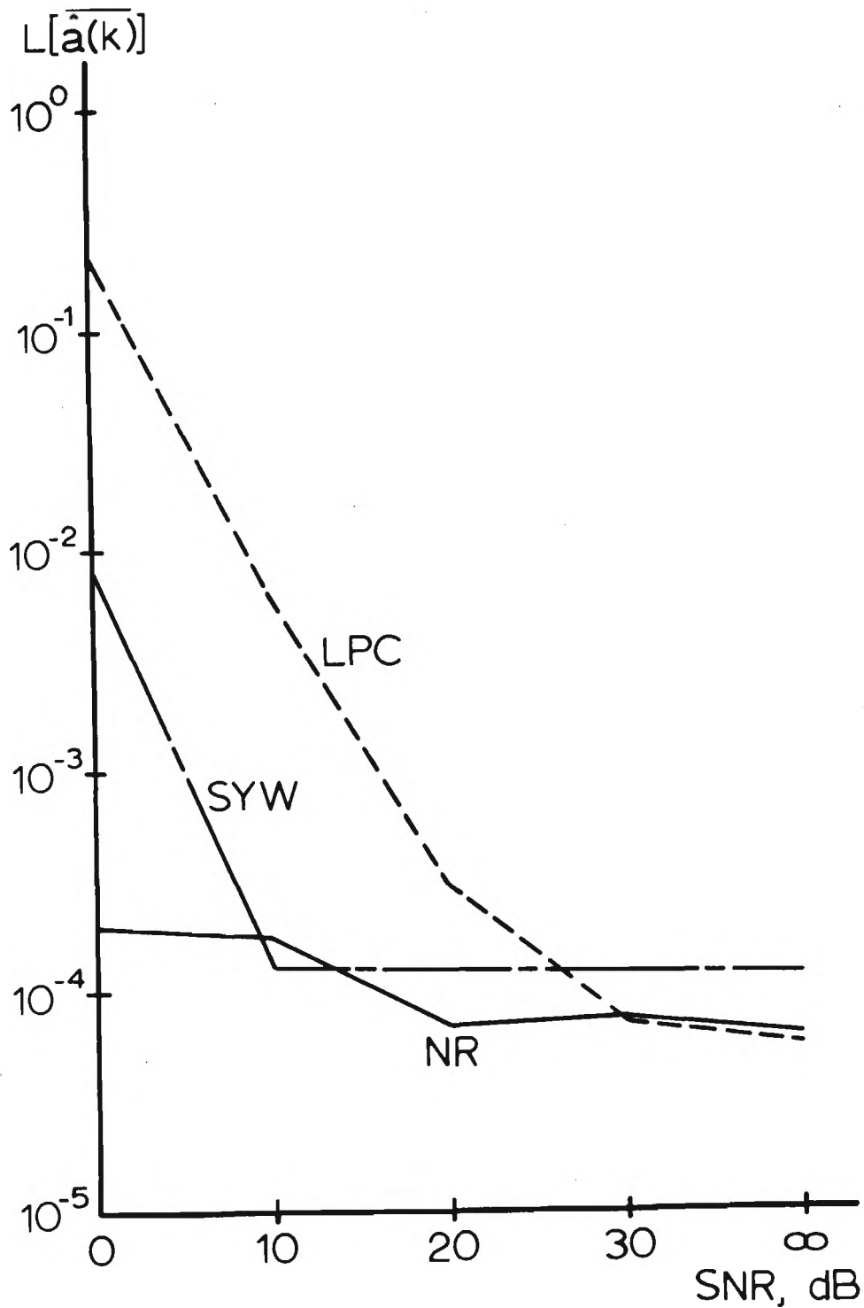
Figure 4-28: Distance measures for three estimates of the AR(4) model coefficients a) L[\hat{a}(k)]
