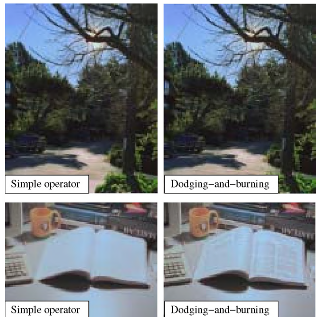
Figure 8: The simple operator of Equation 3 brings out sufficient detail in the top image (dynamic range is 6 zones), although applying dodging-and-burning does not introduce artifacts. For the bottom image (dynamic range is 15 zones) dodging-and-burning is required to make the book’s text visible.
