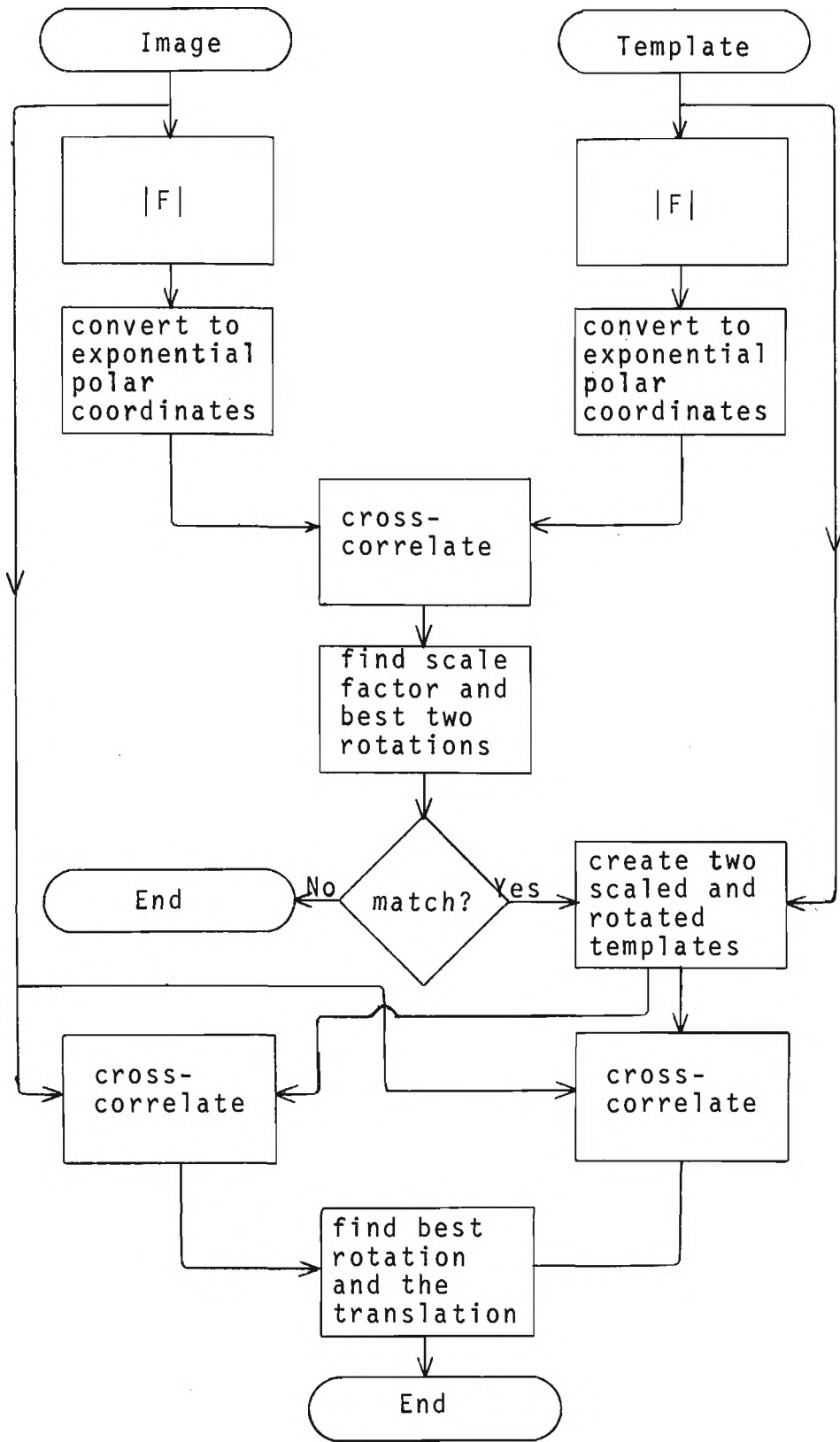
Figure 3 Two-dimensional generalized correlation. Magnitude method.
