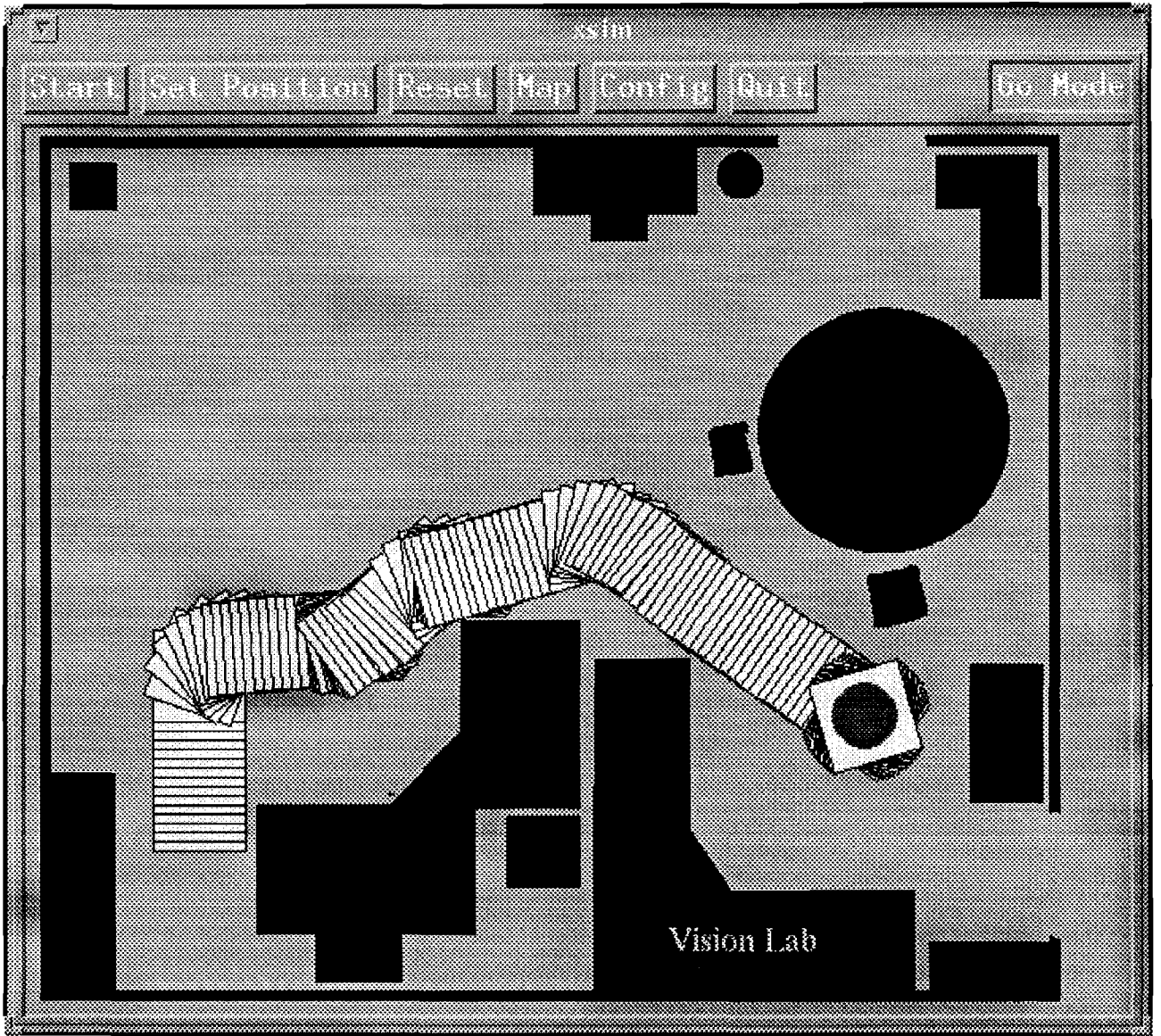
Figure 19: The trajectory of the robot from the initial to the goal point.
