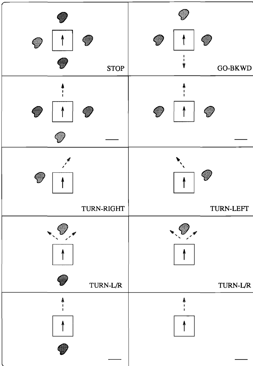
Figure 15: The reaction control when the system state = FORWARD .
