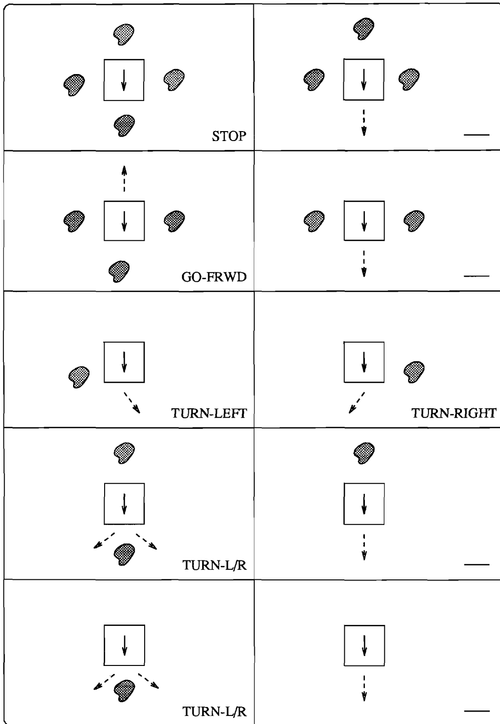
Figure 16: The reaction control when the system state = BACKWARD .
