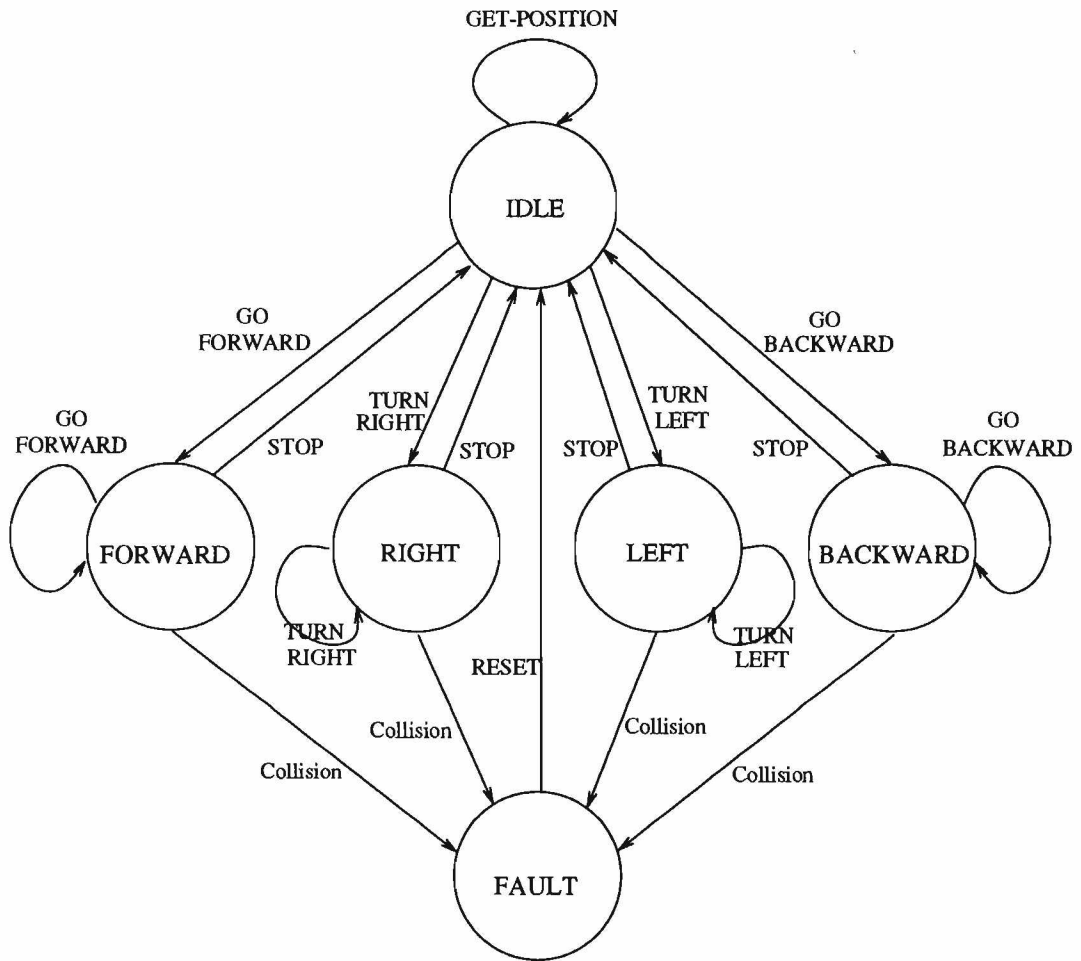
Figure 13: The relation between the system states and the commands.
