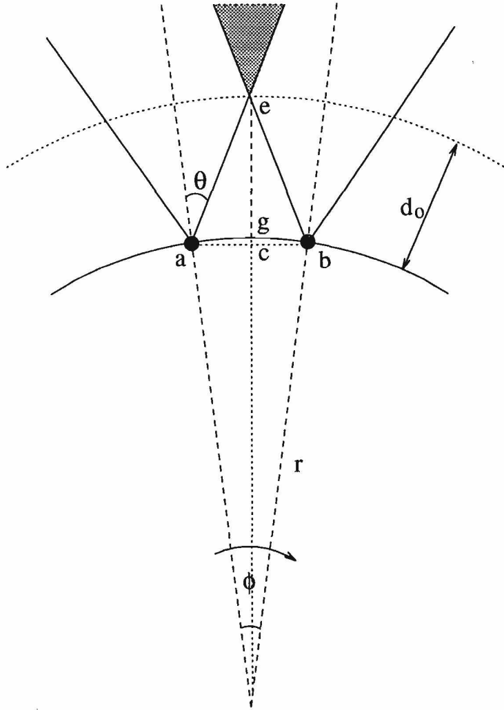
Figure 10: Rotating the robot \phi degrees.
