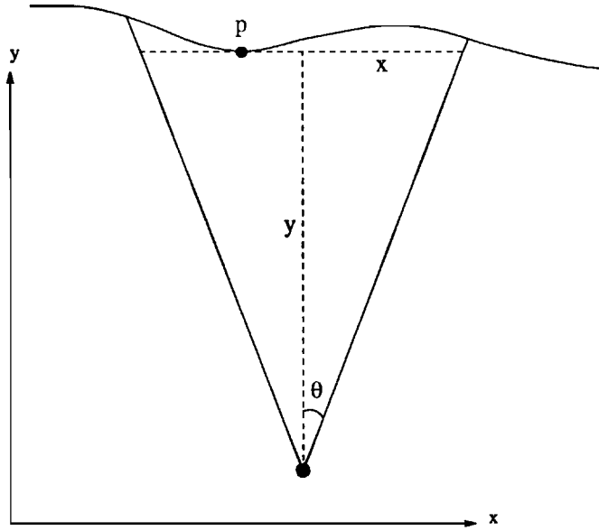
Figure 4: The simplified sonar model.
