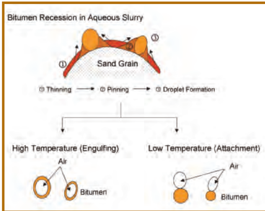
Figure 4-6. Bitumen liberation and aeration in water-based extraction process.
