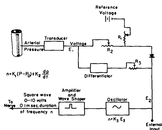
FIG. 1. Diagram of an electronic analog of the carotid sinus and the equation which describes its function.
