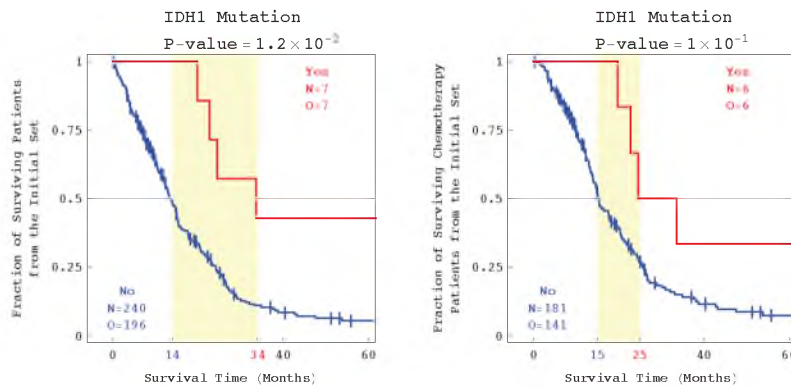
Figure S11 (left). KM survival analysis of the initial set of 251 patients classified by a mutation in the gene IDH1 .
