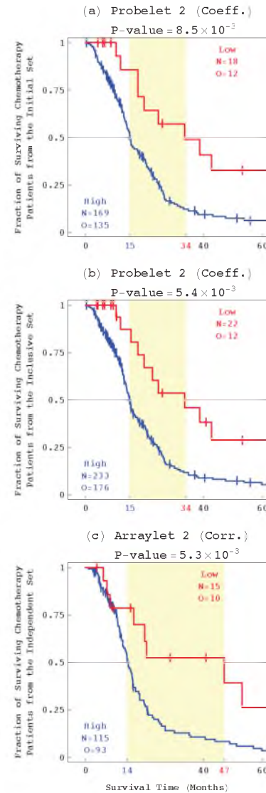
Figure S10. Kaplan-Meier (KM) survival analyses of only the chemotherapy patients from the three sets classified by GSVD.
