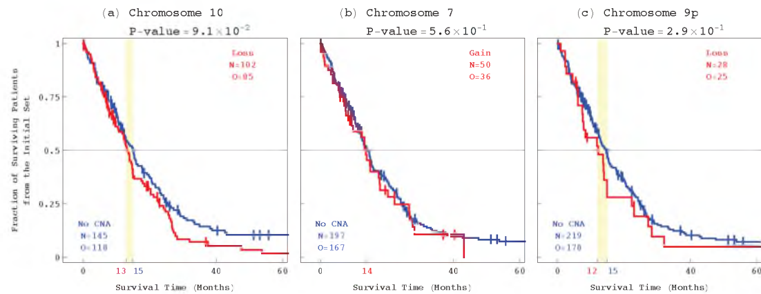
Figure S13. KM survival analyses of the initial set of 251 patients classified by GBM-associated chromosome number changes. (a) Analysis of the 247 patients with TCGA annotations in the initial set of 251 patients, classified by number changes in chromosome 10, shows almost overlapping Kaplan-Meier (KM) [36] curves with a KM median survival time difference of \sim 2 months, and a corresponding log-rank test P -value \sim 10^{-1} , meaning that chromosome 10 loss, frequently observed in GBM, is a poor predictor of GBM patients' survival. (b) KM survival analysis of the 247 patients classified by number changes in chromosome 7 shows almost overlapping KM curves with a KM median survival time difference of < \text{one month} , and a corresponding log-rank test P -value > 5 \times 10^{-1} , meaning that chromosome 7 gain is a poor predictor of GBM survival. (c) KM survival analysis of the 247 patients classified by number changes in chromosome 9p shows a KM median survival time difference of \sim 3 months, and a log-rank test P -value > 10^{-1} , meaning that chromosome 9p loss is a poor predictor of GBM survival.
