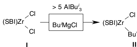
Scheme 1. Preparation of complex II .
