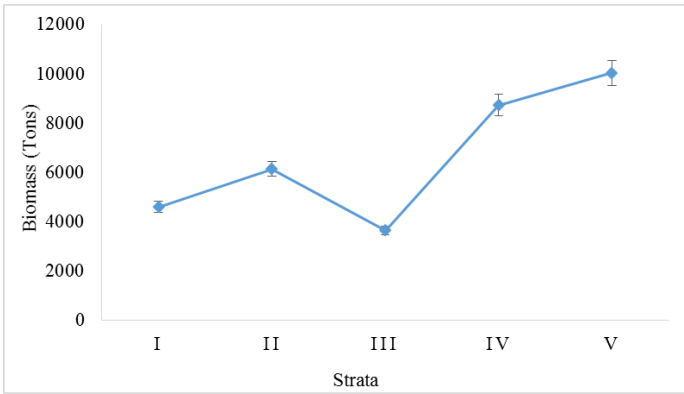
Figure 2. Biomass (tone) in different stratum at the northern coast of the Oman Sea.
