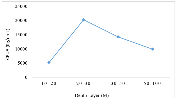
Figure 5. Catch per unit area (kg/ nm 2 ) in different depth layer at the Northern coast of the Oman Sea.
