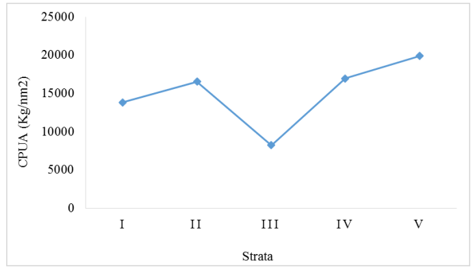
Figure 4. Catch per unit area (kg/ nm 2 ) in different stratum at the Northern coast of the Oman Sea.
