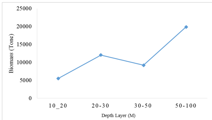
Figure 3. Biomass (tone) in different depth layer at the Northern coast of the Oman Sea.
