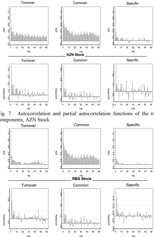
Fig. 8. Autocorrelation and partial autocorrelation functions of the two components, RBS Stock.
