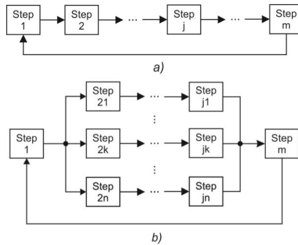
Fig. 3 Sequential control system with: a) single branch, b) parallel branches
