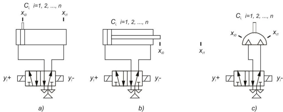
Fig. 1 Pneumatic system with two end positions with: a) Symmetric actuator, b) Asymmetric actuator, c) Semi-rotary drive
