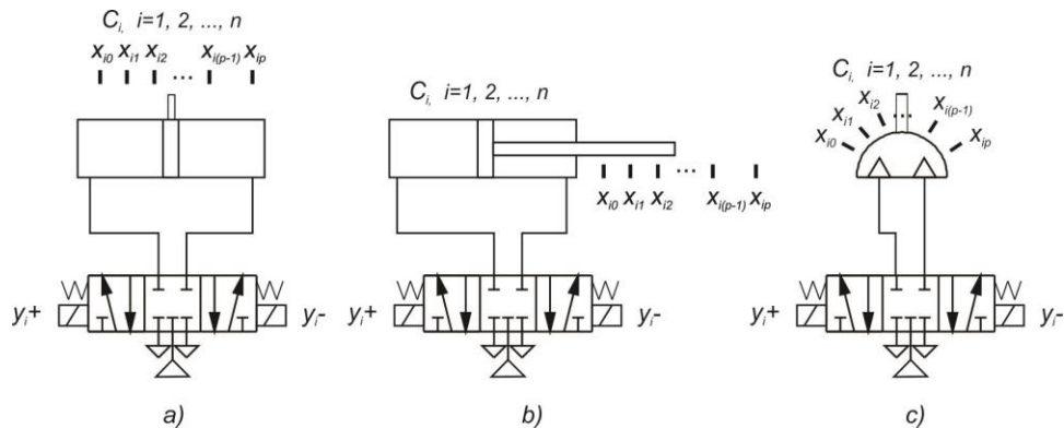
Fig. 2 Pneumatic system with more than two end positions with: a) Symmetric actuator, b) Asymmetric actuator, c) Semi-rotary drive
