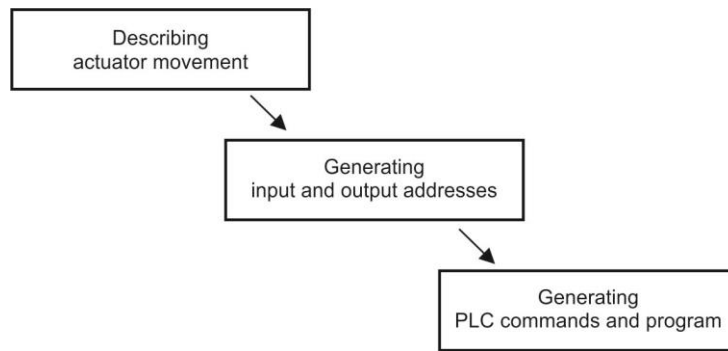
Fig. 4 Block scheme of automatic PLC programming of the sequential control of pneumatic actuators
