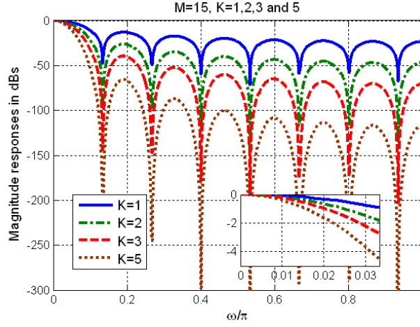
Fig. 3 Overall comb magnitude responses and passband zoom, for different values of K
