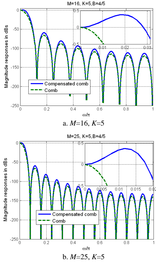
Fig. 5 Magnitude responses of comb and compensated comb in [7]
