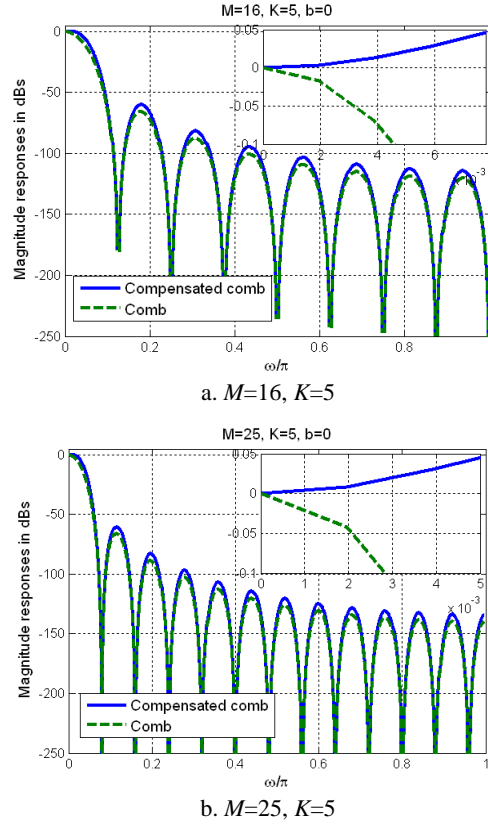
Fig. 6 Magnitude responses of comb and compensated comb in [8]
