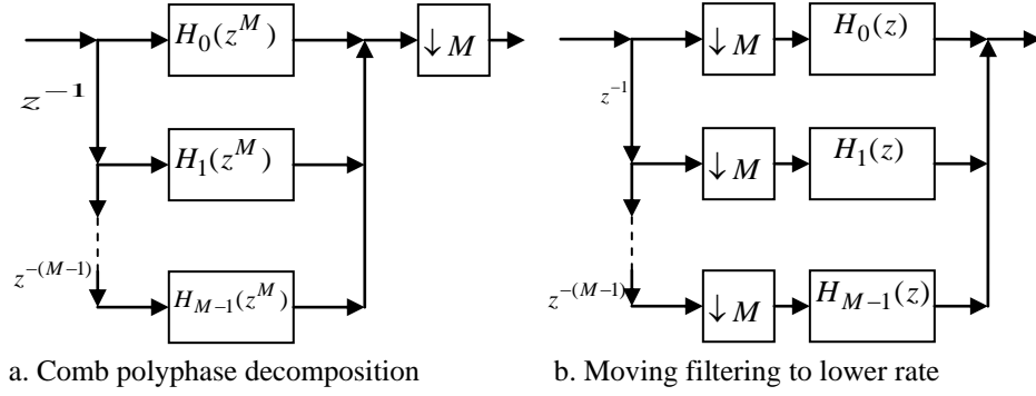
Fig. 2 Polyphase decomposition
