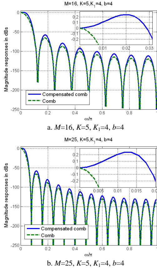
Fig. 8 Magnitude responses of comb and compensated comb in [10]
