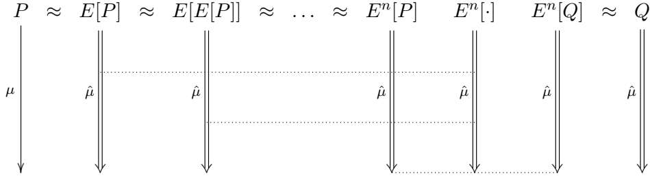
Figure 4: Proof of Theorem 3.5, building a a transition of E^n[Q] where Q does not move
