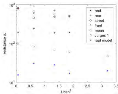
Figure 5. Res_{facet} averaged over different facets as a function of U_{can}^2 . The mean of Res_{facet} is the average over rear, ground and front surfaces. From low to high U_{can}^2 corresponds to H/W = 2, 1/5, 1/11, 1 and 1/2 respectively.
