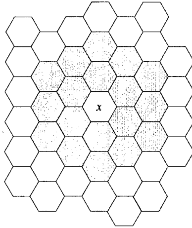
Figure 2.2: Reuse distance
