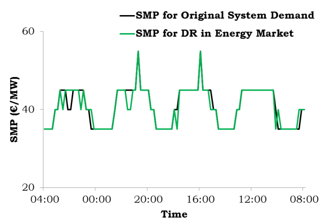
Fig. 4. Electricity price with and without DR for a peak load of 7500 MW
