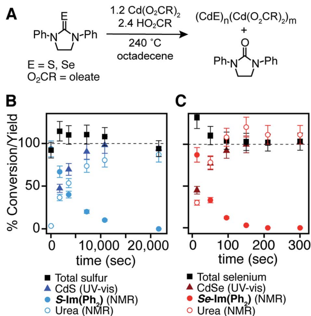
Fig. 1 (A) Synthesis of cadmium chalcogenide nanocrystals from (B) S -Im( \text{Ph}_2 ) and (C) Se -Im( \text{Ph}_2 ). Comparison of mass balance and kinetics as measured by UV-vis absorption and ^1\text{H} NMR spectroscopies. Error bars correspond to 10% error in NMR measurement.
