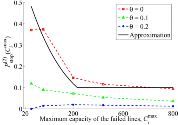
Fig. 6. Simulation results of P_{\text{stop}}^{(2)}(C_i^{\text{max}}) for r = 0.7, e = 0.1 and three values of \theta . The solid line is the parametric approximated function when \theta = 0 .
