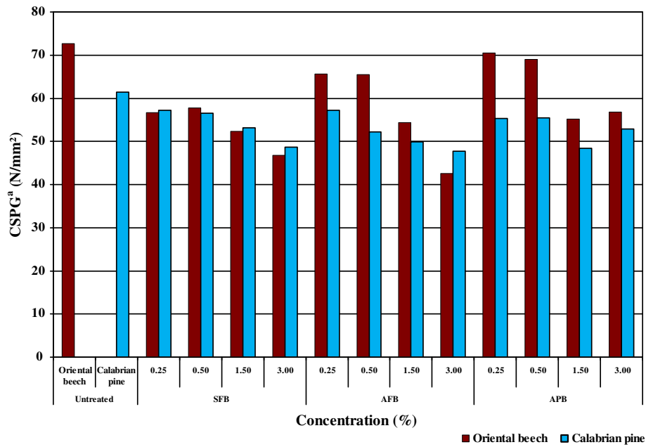
Fig. 1. The CSPG of Oriental beech and Scots pine impregnated with borates.
