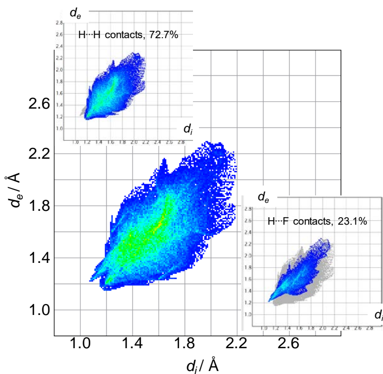
Figure 6 The 2D-fingerprint plots of [\text{Cs}(\text{G4})_2]^+ in [\text{Cs}(\text{G4})_2][\text{SF}_5] . The two insets highlight the H...H and H...F contacts. The symbols, d_e and d_i , are the distances from the surface to the nearest nucleus, external and internal, respectively.
