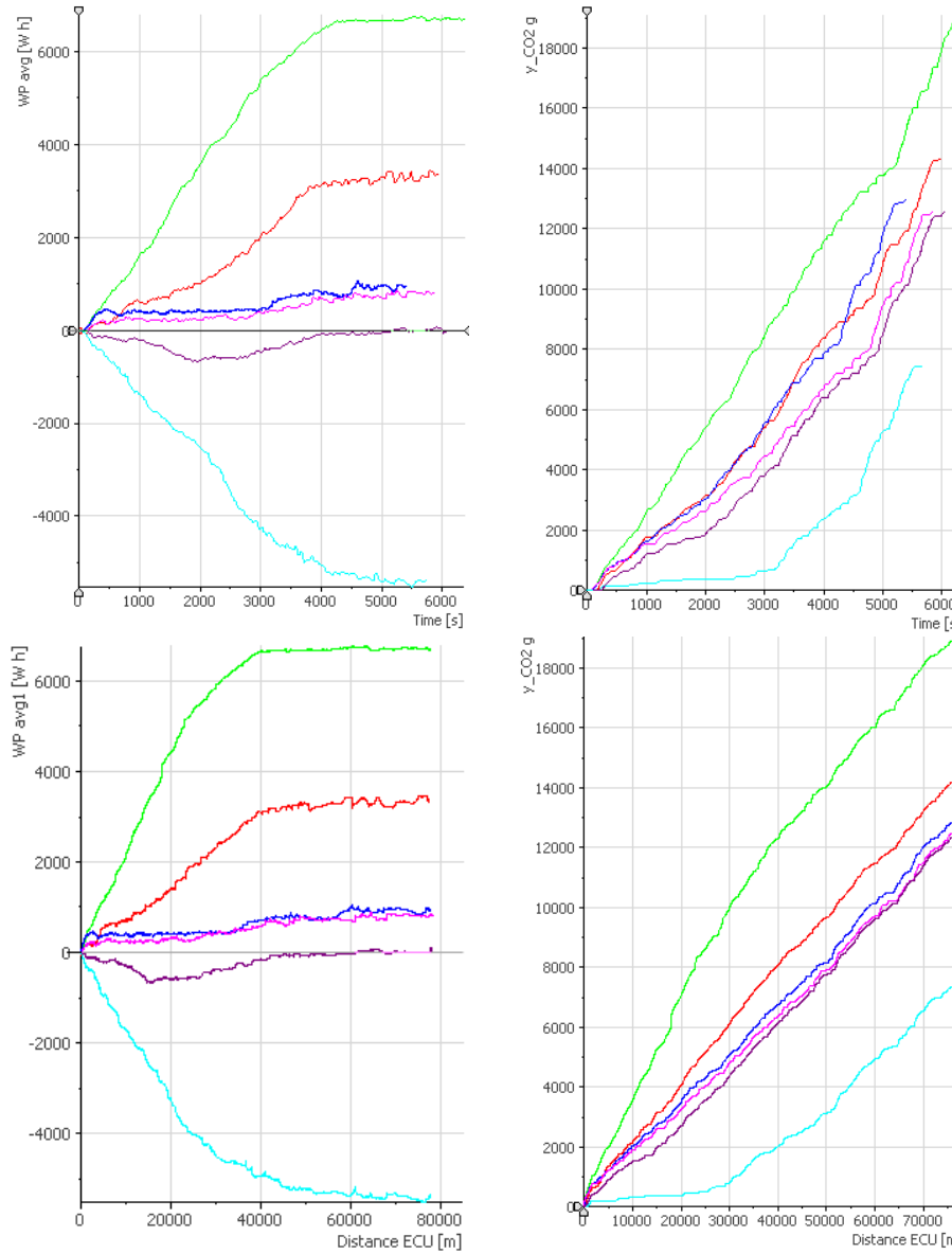
Figure 12: Driving Modes impact on CO2 grams and Wh (over time and over distance)
