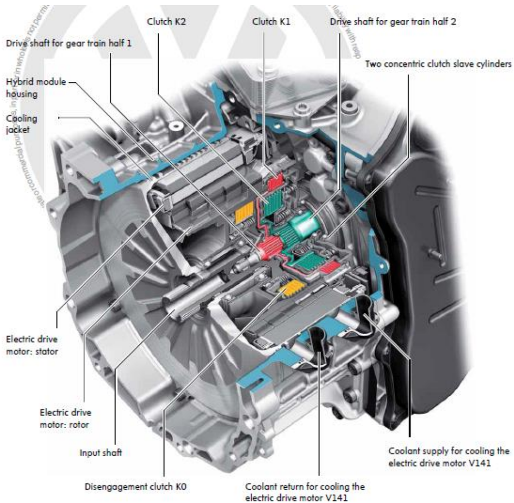
Figure 3: Hybrid module design overview (Picture from http://qualityservicemanual.com/725/volkswagen-audi-skoda-self-study-programme-sspservice-training-collection )
