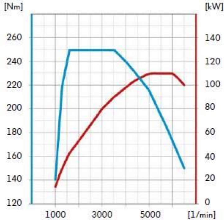
Figure 1: ICE Torque and power diagram. (Picture from https://www.alientech-tools.com/golf-gte-hybrid/ )
