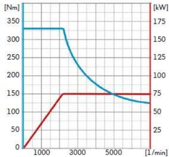
Figure 2: Electrical motor configuration; torque and power diagram (Picture from https://www.alienech-tools.com/golf-gte-hybrid/ )
