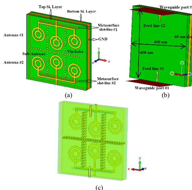
Fig.1. Proposed on-chip array antenna prototype.
