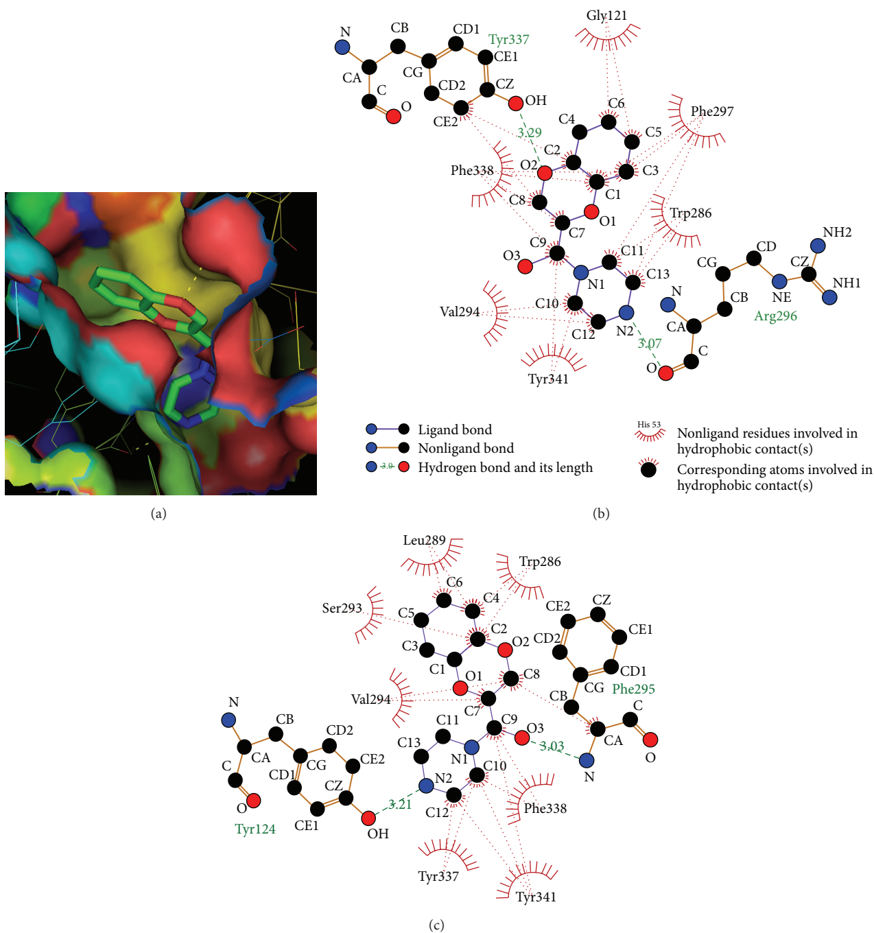
FIGURE 3: (a) Catalytic site docking of 1-(1,4-benzodioxane-2-carbonyl) piperazine (K)[Pymol view]. (b) Catalytic site docking of 1-(1,4-benzodioxane-2-carbonyl) piperazine (K). (c) Peripheral anionic site docking of 1-(1,4-benzodioxane-2-carbonyl) piperazine (K).
