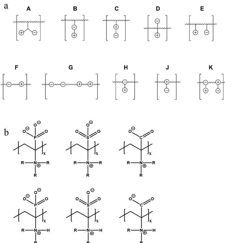
Figure 2. (a) Different arrangements of the functional groups in polyelectrolytic chains, reprinted from [101], and (b) commonly employed zwitterionic repeating units in polymeric materials.
