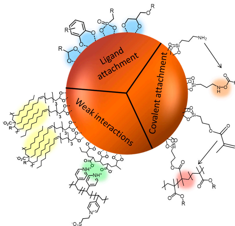
Figure 4. Schematic representation of applied immobilization techniques for polyzwitterions at the surface of magnetic nanoparticles (MNPs).
