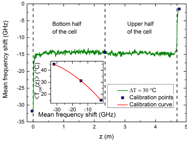
Fig. 7. The time-averaged frequency shift as a function of the vertical distance z from the bottom conducting plate ( \Delta T = 30^\circ\text{C} , Ra = 3.27 \times 10^{11} ) measured in a vertical 1 m from the cell sidewall. The vertical dashed black lines indicate the location of the cell centre and the positions of the plates. The inset represents a calibration curve used for transformation of the time-averaged frequency shift to the time-averaged temperature \langle T(z) \rangle . The red curve is second order polynomial fit of the three selected data points shown as blue squares. The temperature \langle T_{cal}(z) \rangle of the middle point was measured by the lower Pt100 probe, the other two points were measured by sensors placed in plates.
