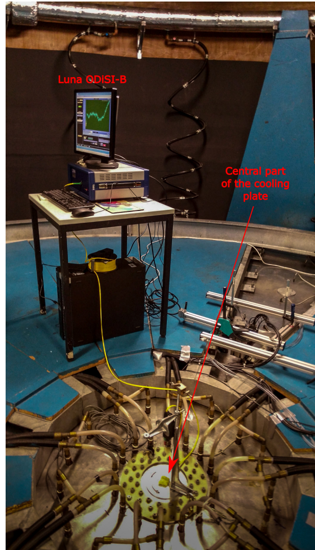
Fig. 4. The arrangement of Luna ODiSI-B in the space above the top plate. Optical fibre here enters the cell in the centre of the plate. The pipelines belong to the water cooling system of the plate.
