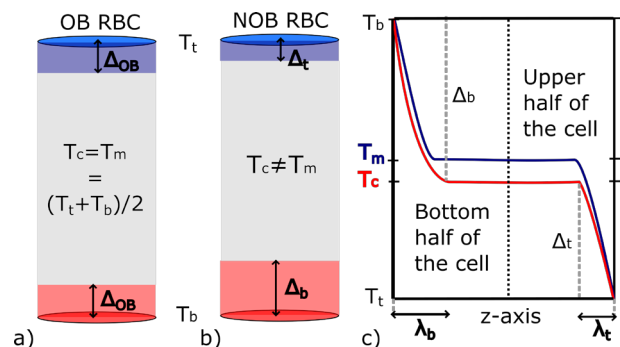
Fig. 1. Schematic illustration of the thermal boundary layers and vertical temperature profiles in RBC: a) Thermal boundary layers in OB RBC where the temperature drops ( \Delta_{OB} ) on the top and bottom boundary layers are equal. The turbulent core temperature T_c equals the mean temperature T_m . b) Thermal boundary layers in NOB RBC, where the temperature drops on the top ( \Delta_t = T_c - T_t ) and bottom ( \Delta_b = T_b - T_c ) layers are asymmetric. The turbulent core temperature T_c differs from the mean temperature T_m . c) The vertical temperature profile in the OB (blue) and NOB (red) RBC. \lambda_t and \lambda_b represents the thickness of the top and bottom boundary layers.
