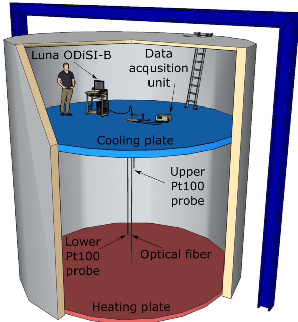
Fig. 3. Schematic illustration of Luna ODiSI-B and Pt100 probes installation in the axis of BOI. Luna ODiSI-B system and data acquisition unit for Pt100 probes were placed on an upper side of the top plate. The optical fibre passes through a hole in the plate and is fixed to the bottom plate. Both Pt100 probes were suspended on the feed cables passing through the hole in the top plate together with the fibre. The upper Pt100 probe serves only for measurement of temperatures profiles across the top boundary layer, whereas the lower Pt100 probe serves for measurement both across the bottom layer and in the turbulent core.
