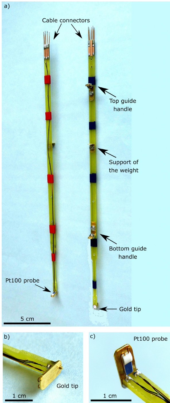
Fig. 5. Lower Pt100 probe for the reference temperature profiles measurements designed at ISI. a) The probe is shown from the front and back side. b) Detail view on of the gold tip which serves as the electrical indicator of mechanical contact of the probe with the bottom plate. Opposite to the tip, the small electrode made of the copper sheet is installed on the surface of the bottom plate to secure the electrical connection. c) Detail view of the Pt100 sensor fastened to the brass plate.
