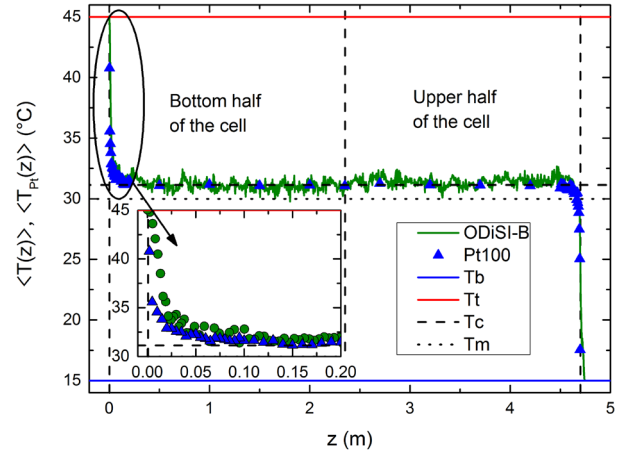
Fig. 8. Comparison of the time-averaged temperatures measured by Luna ODISI-B (green solid curve, filled green circles) and Pt100 probes (blue filled triangles) as a function of distance z from the bottom plate ( \Delta T = 30^\circ\text{C} , Ra = 3.27 \times 10^{11} ). Both profiles were measured along the vertical in the radial position 1 m from the cell sidewall. The vertical dashed black lines indicate the location of the cell centre and the plates. The solid horizontal lines represent the time-averaged temperatures of the top ( T_t - blue line) and bottom ( T_b - red line) plates. The horizontal dotted black line corresponds to the time-averaged mean plate temperature T_m . The dashed black line represents the time-averaged turbulent core temperature T_c measured in the cell centre by Pt100 probe.
