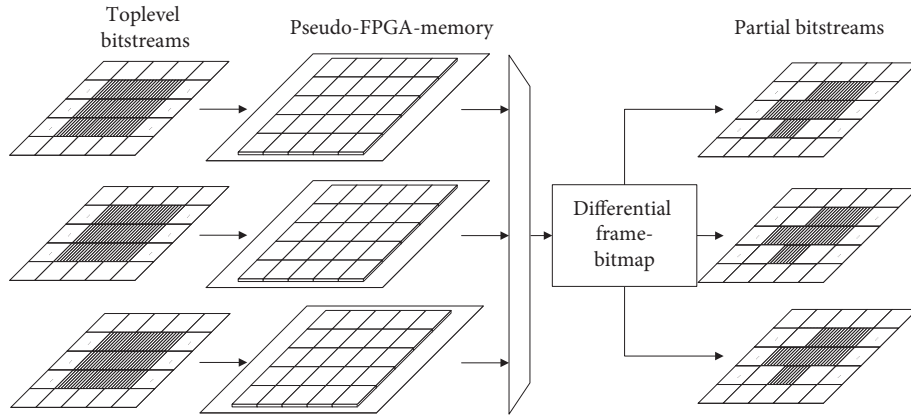
FIGURE 2: Functionality of the torCombitgen tool.
