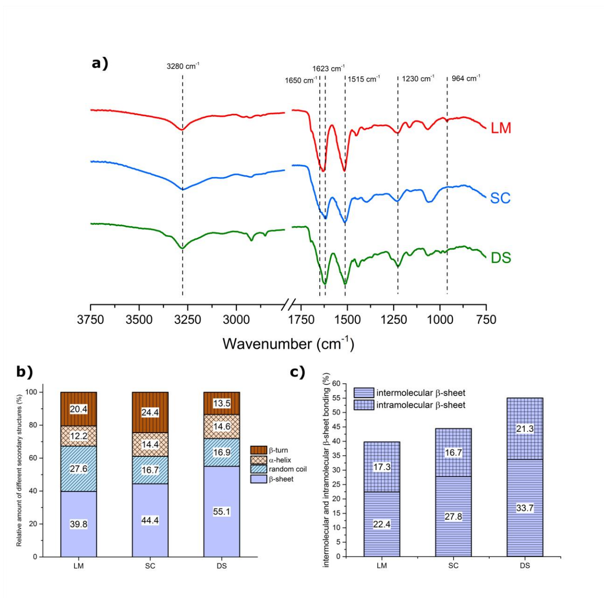
Figure 2. Molecular structure analyses. a) Samples FTIR spectra; b) FTIR secondary structure analysis on Amide I of different silks (based on related structure peak areas); c) Ratio of intermolecular and intramolecular bonds detected on different silks (based on related intermolecular and intramolecular \beta -sheet areas). LM: Linothele m. silk; SC: Bombyx m. silk; DS: degummed Bombyx m. silk.
