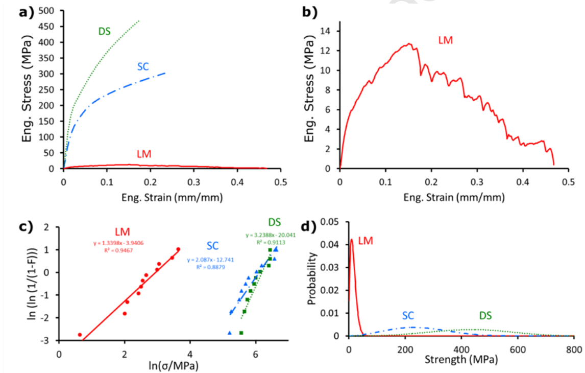
Figure 4. Mechanical behaviors of samples. a) the tested different silks; b) LM silk. c) Linear regression method used to compute the Weibull parameters and d) Weibull probability distribution of the strength of the tested silks. LM: Linothele m. silk; SC: Bombyx m. silk; DS: degummed Bombyx m. silk.
