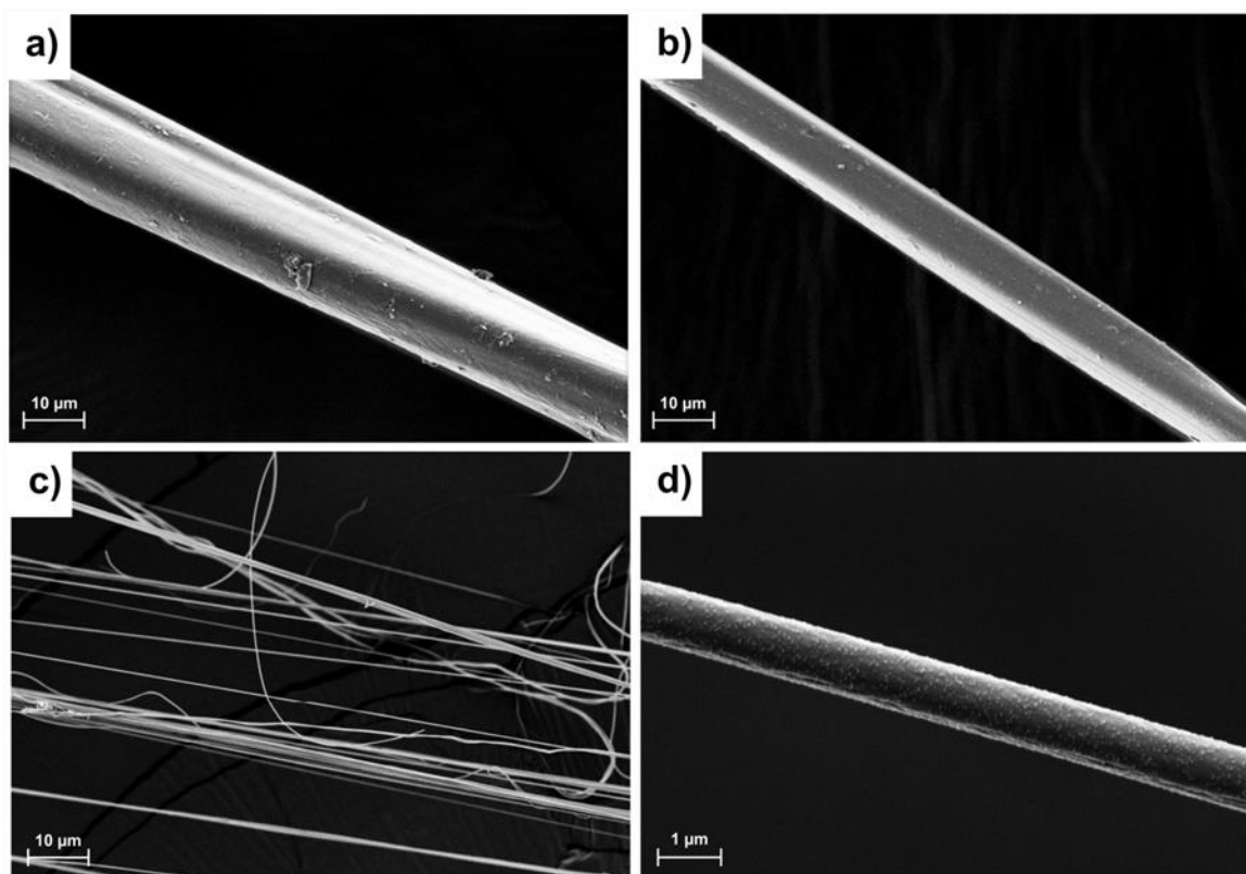
Figure 3. FE-SEM images of silk fibers. a) Silkworm cocoon silk from Bombyx mori before (SC) and b) after degumming (DS); c) and d) Linothele megatheloides spider silk (LM) in different magnifications. The scale bars in figure a, b and c are equivalent to 10 \mu\text{m} and the scale bar in figure d is equivalent to 1 \mu\text{m} .
