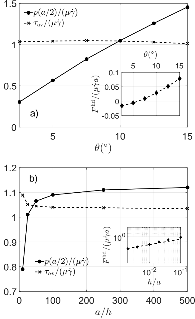
Figure 8: Total pressure force per unit area p = p^- - p^+ at the midpoint s = a/2 and length-averaged shear stress, \tau_{av} as a function of (a) wedge angle for a/h = 50 and (b) ratio a/h for \theta = 10^\circ . Inset of a): Edge force F^{hd}/(\mu\dot{\gamma}a) vs. \theta . Inset of b): Edge force F^{hd}/(\mu\dot{\gamma}a) vs. h/a (log-log). The dashed line in the inset corresponds to a power-law exponent of \sim 0.62 .
