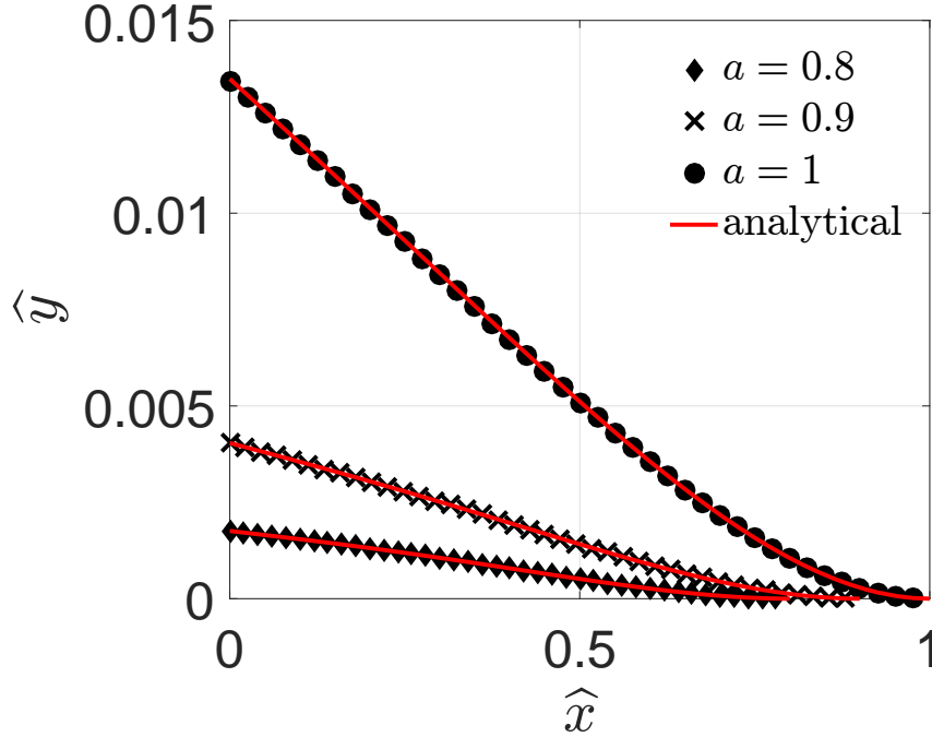
Figure 13: Out-of-plane displacement of the flap from simulations (markers) and analytical solutions (red lines) for three values of a , angle dependent load in case 2 (edge load plus distributed load) and \mu\dot{\gamma}/D = 1 . The results are in units of (D/(\mu\dot{\gamma}))^{1/3} .
