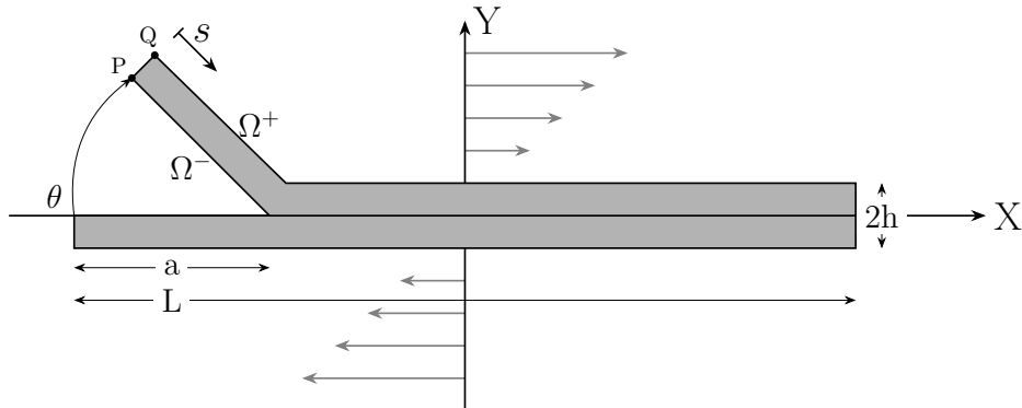
Figure 2: Simplified geometry used in the flow simulation.
