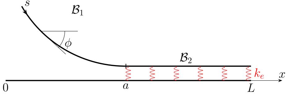
Figure 9: Schematic of the solid mechanics model.
