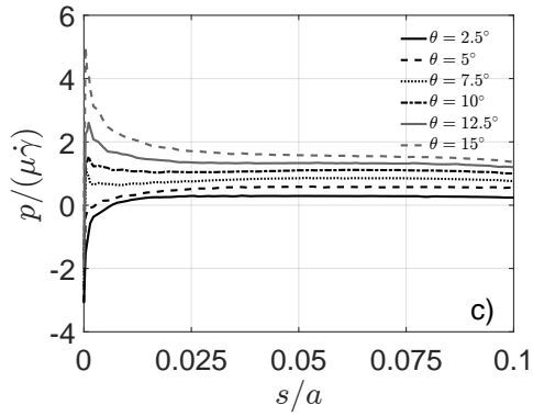
Figure 4: (a) and (b): Pressure distribution on the surfaces \Omega^+ and \Omega^- , respectively. The thickness of each layer is h = a/50 . (c) Total pressure p = p^- - p^+ in the region 0 \leq s/a \leq 0.1 near the edge of the flap.
