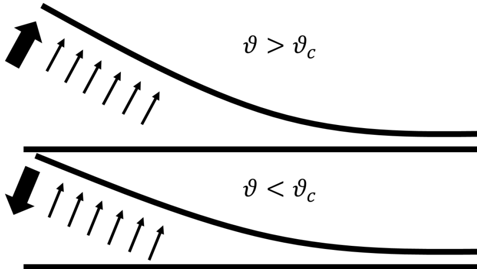
Figure 7: Schematic view of the hydrodynamic load distribution on the flap for angles larger and smaller than the critical angle \theta_c \simeq 7.5^\circ .
