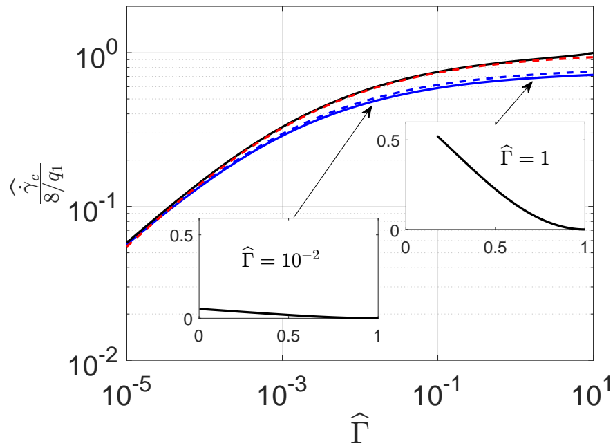
Figure 15: Non-dimensional shear rate as a function of the non-dimensional adhesion energy in the large displacement theory for different approximations of the wedge angle: tip angle (continuous blue line), local angle (dashed blue line) and secant angle (black line). The red line is the analytical solution for small displacements and secant angle approximation.
