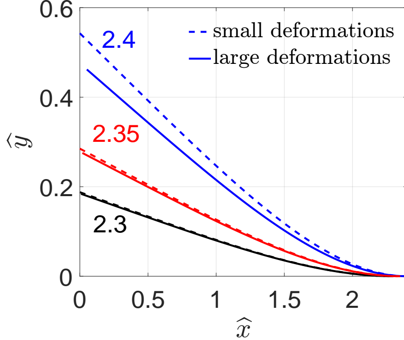
Figure 14: Flap shape comparing the linear (small displacement) and the non-linear (large displacement) formulation. The flap is plotted for different values of a and \mu\dot{\gamma}/D = 0.1 . The quantities in the plot are in (D/(\mu\dot{\gamma}))^{1/3} units).
