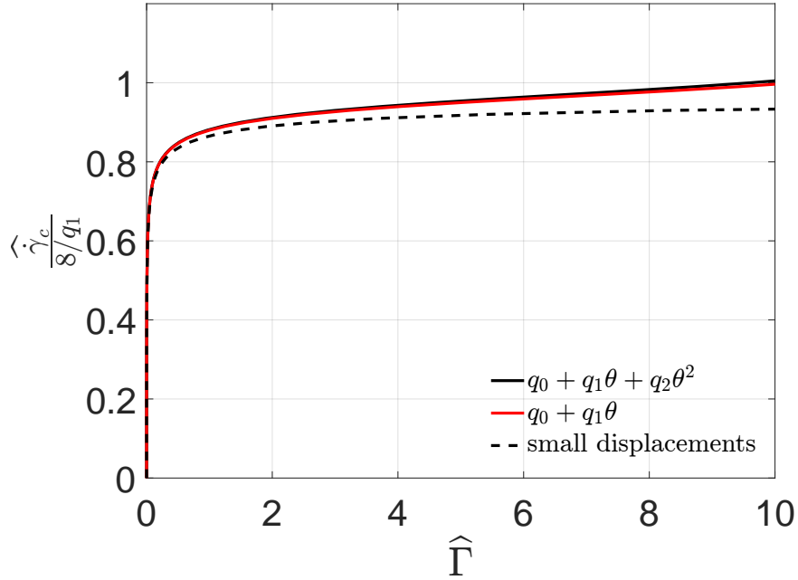
Figure 17: Relation between non-dimensional shear rate and non-dimensional adhesion energy, comparing the linear and non-linear loads.
