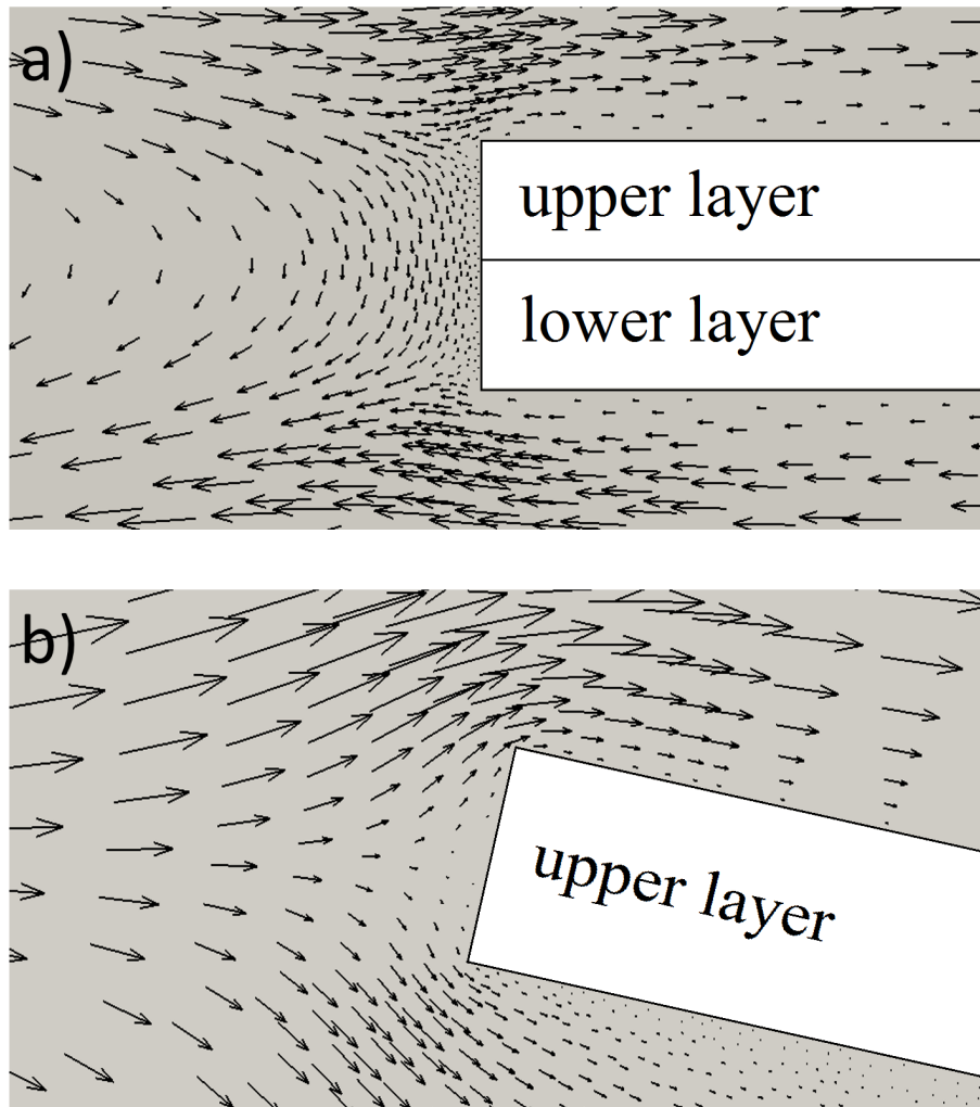
Figure 6: Velocity field near the edge for (a) \theta = 0^\circ and (b) \theta = 12.5^\circ .
