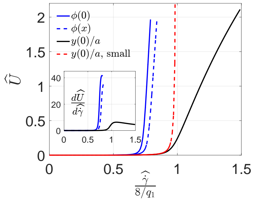
Figure 16: Non-dimensional bending energy vs. non-dimensional shear rate in the large displacement theory for different approximations of the wedge angle in the forcing term. The red dashed line correspond to the small-displacement theory, while the other lines are for the large-displacement theory. The inset shows the derivative of \widehat{U} with respect to \widehat{\dot{\gamma}} .
