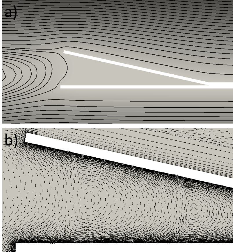
Figure 3: (a) Streamlines around the particle. (b) Detail of the recirculating eddies in the wedge below the flap.
