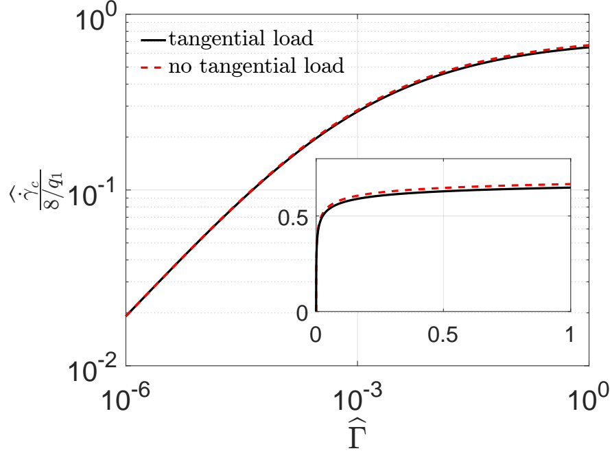
Figure 19: Non-dimensional shear rate against non-dimensional adhesion energy in the large displacement limit with tangential load \tau = 1.05\mu\dot{\gamma} (black line) and without tangential load (red dashed line) applied on the flap. The inset shows the same plot on a linear scale.
