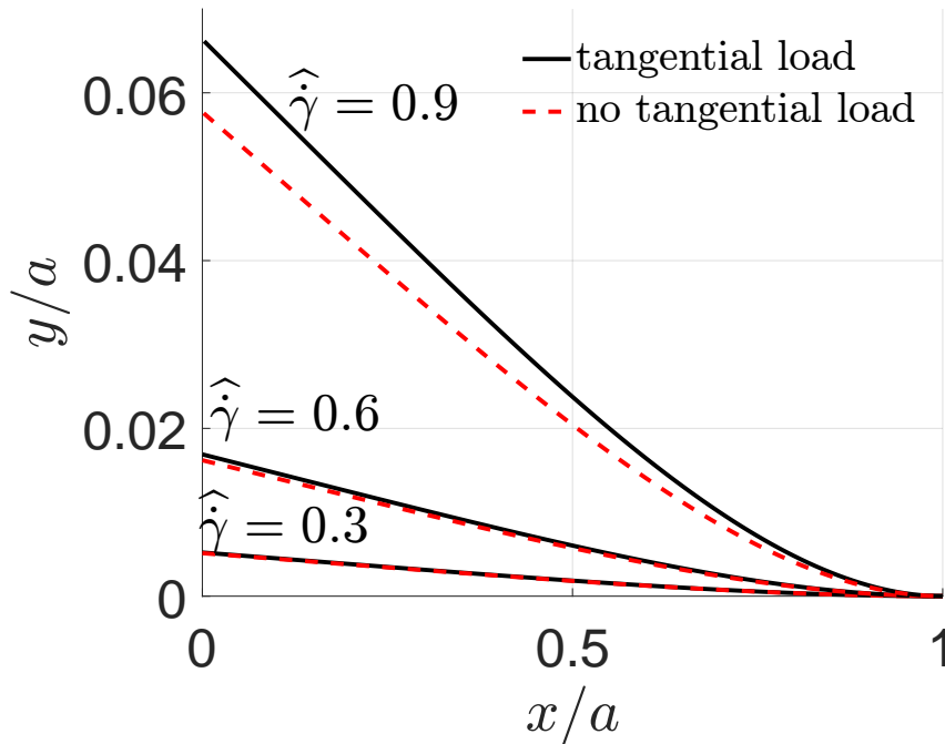
Figure 18: Flap shape in the large displacement limit with tangential load (black line) and without tangential load \tau = 1.05\mu\hat{\gamma} (red dashed line) for different values of \hat{\gamma} .
