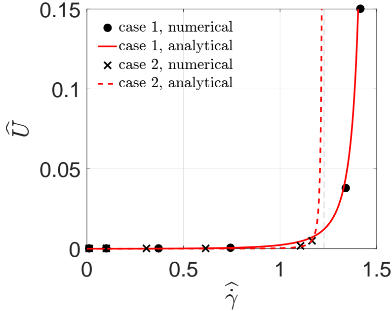
Figure 11: Non-dimensional bending energy as a function of the non dimensional shear rate. The markers represent the results from finite difference simulations. The red lines represent the analytical solutions.
