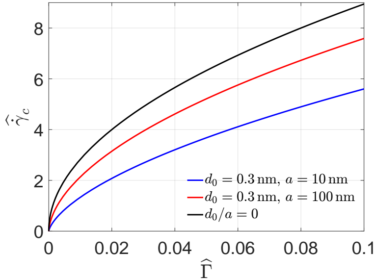
Figure 10: Non-dimensional shear rate \hat{\gamma}_c as a function of the non-dimensional adhesion energy \hat{\Gamma} for different values of the parameter d_0/a . An increase in the stiffness of the foundation (smaller d_0 ) corresponds to larger values of the critical shear rate
