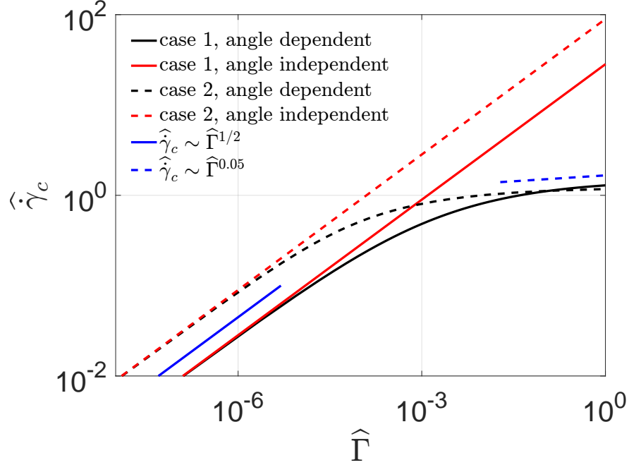
Figure 12: Non-dimensional shear rate as a function of the non-dimensional adhesion energy for different loads. The blue lines show the power-law trends for small values of \hat{\Gamma} (continuous line) and large values of \hat{\Gamma} (dashed line).
