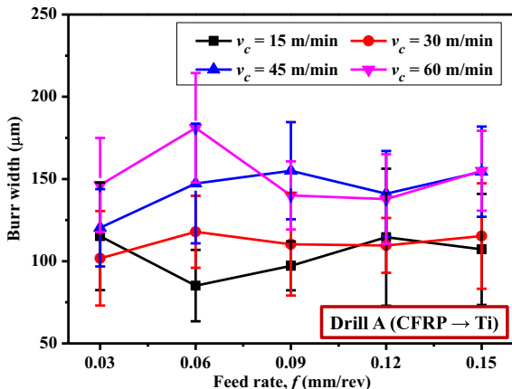
Fig. 32. Parametric effects on burr width when using drill A (CFRP → Ti cutting sequence).
