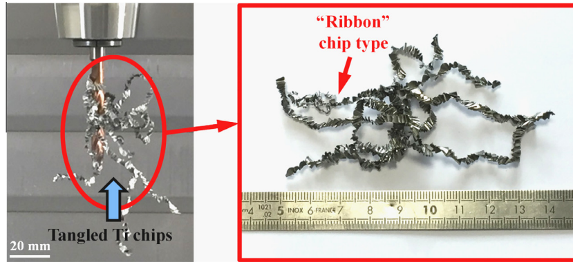
Fig. 14. Photographs showing the tangled Ti chips on drill body and resected “ribbon” type chips after drilling with drill B in the CFRP → Ti cutting sequence ( v_c = 30 m/min, f = 0.03 mm/rev).
