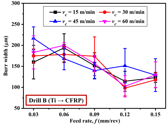
Fig. 34. Parametric effects on burr width when using drill B (Ti → CFRP cutting sequence).
