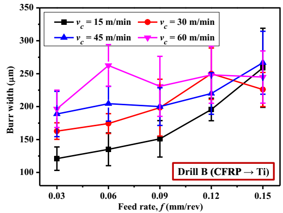
Fig. 33. Parametric effects on burr width when using drill B (CFRP → Ti cutting sequence).
