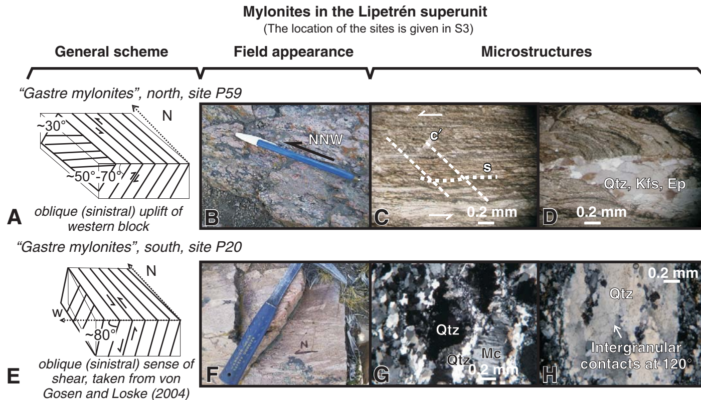
Figure 4. Mylonites in the Lipetrén superunit; their location can be found in Table S3 (see footnote 1). (A)–(D) General scheme, field appearance, and microstructures of the northern strip of mylonites east of Gastre town at site P59. (A) General scheme of the “Gastre mylonites” of von Gosen and Loske (2004) with a NNW-SSE strike, steeply dipping to the W-SW, and with an oblique (sinistral) sense of shear. (B) Thin foliation planes of NNW-SSE strike. (C) S-C’ structure defining a sinistral sense of shear; the S surfaces are defined by quartz, feldspars, micas, and opaque minerals, and they are crenulated by the C’ surfaces defined by micas. (D) Late quartz-feldspathic veins disrupting the mylonitic foliation. (E)–(H) General scheme, field appearance, and microstructures of the southern strip of mylonites east of Gastre town at site P20. (E) General scheme of the southern band of Gastre mylonites of site P20, with steeply dipping N-S foliation and a steeply plunging lineation; the dextral sense of shear is taken from von Gosen and Loske (2004). (F) Parallel foliation planes of N-S orientation. (G)–(H) Quartz and feldspar porphyroclasts surrounded by quartz and feldspar recrystallized subgrains with post-kinematic annealing. All photomicrographs were taken under crossed polars. Mineral abbreviations in all figures are after Kretz (1983). Qtz—quartz; Kfs—K-feldspar; Ep—epidote; Mc—microcline.
