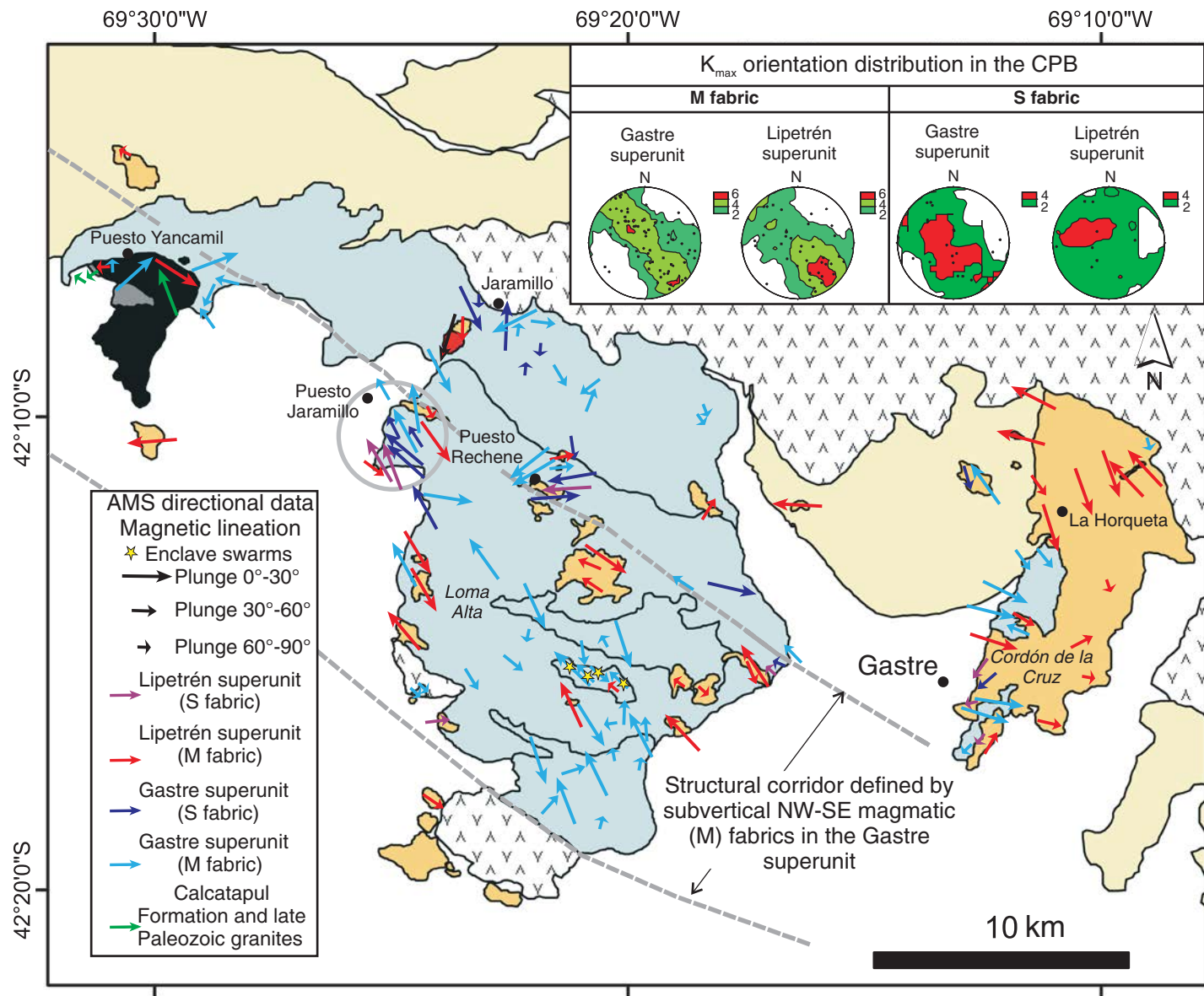
Figure 8. Map showing magnetic lineation ( K_{max} direction) in the Central Patagonian batholith (CPB). The dashed lines represent the Gastre corridor of magmatic fabrics, whose strike was defined only with those magnetic fabrics of high inclinations (from 60° to 90°). As in Figure 7, the circle shows the area where the fabrics of the Lipetrén superunit bear a different strike with respect to the magmatic and solid-state fabrics of the Gastre superunit. Inset shows K_{max} distribution of the magmatic (M) and low-temperature solid-state (S) fabrics (as described in the field) within the Gastre and Lipetrén superunits. The stereonets represent Kamb contoured equal-area lower-hemisphere stereographic projections made with the software Stereonet 9.9.5 (Allmendinger et al., 2013; Cardozo and Allmendinger 2013). The scale represents Kamb contours in standard deviation. Lithologic symbol explanations as in Figure 7. AMS—anisotropy of magnetic susceptibility.
