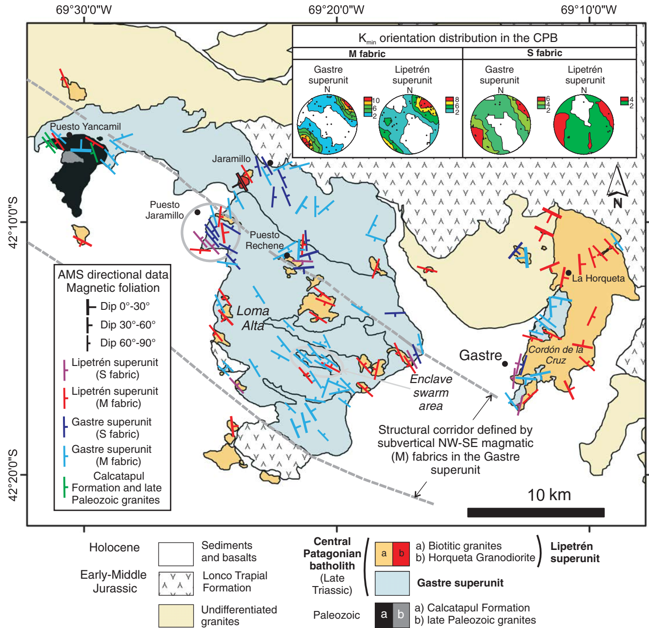
Figure 7. Map showing magnetic foliation planes ( K_{max} - K_{int} planes), defined as the plane perpendicular to K_{min} in the Central Patagonian batholith (CPB). The dashed lines represent the Gastre corridor of magmatic fabrics, whose strike was defined only with those magnetic fabrics of high inclinations (from 60° to 90°). The circle around Puesto Jaramillo encloses the area where the magmatic fabrics of the Lipetrén superunit are not parallel to the magmatic and solid-state fabrics of the Gastre superunit. In contrast, the solid-state fabrics of the Lipetrén superunit are parallel to the magmatic and solid-state fabrics of the Gastre superunit. Inset shows K_{min} distribution of the magmatic (M) and low-temperature solid-state (S) fabrics (as described in the field) within the Gastre and Lipetrén superunits. The stereonets represent Kamb contoured equal-area lower-hemisphere stereographic projections made with the software Stereonet 9.9.5 (Allmendinger et al., 2013; Cardozo and Allmendinger, 2013). The scale represents Kamb contours in standard deviation. AMS—anisotropy of magnetic susceptibility.
