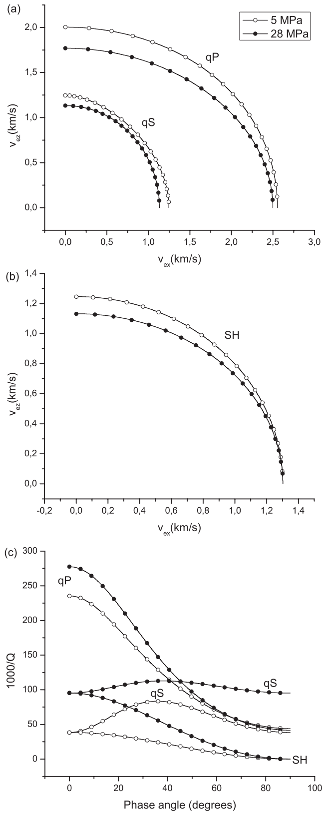
Figure 6. Energy velocity (a and b) and dissipation factor (c) versus angle for the normal (open circles) and overpressure (full circles) cases. Fractal variations of the fracture stiffnesses are modelled. The frequency is 25 Hz.
