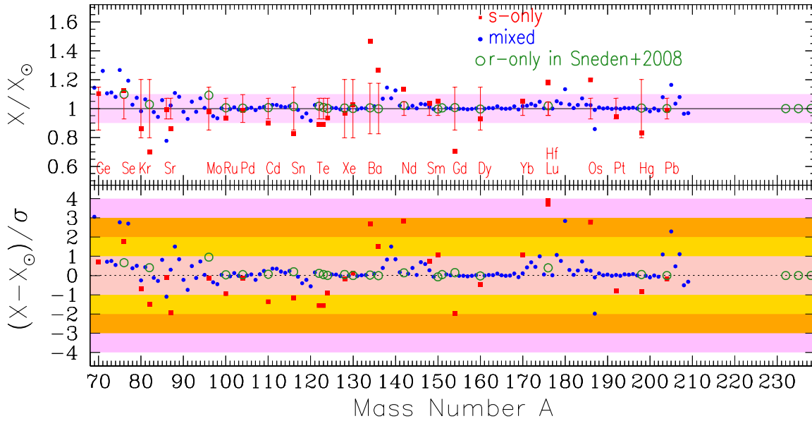
Figure 5. Results compared to uncertainties of pre-solar abundances. Top: Model over-abundances at the time of Solar system formation and elementary uncertainties \pm 1\sigma for the s- only isotopes (vertical red segments, centered at X/X_{\odot}=1 from Lodders et al. (2009) , the names of which are provided in the bottom of the panel; the shaded area indicates the range of \pm 10\% deviation from solar. Bottom: Overabundances (positive) or underabundances (negative) expressed in terms of the corresponding elementary uncertainties. Shaded areas indicate ranges of \pm 1\sigma , \pm 2\sigma , etc.
