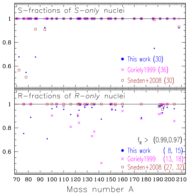
Figure 2. Top: Nuclei having an s-fraction f_s=1 in at least one of the lists of Goriely (1999) , Sneden et al. (2008) or ours. Bottom: Nuclei with r-fraction f_r = 1 in at least one of the cited studies. In parentheses: the number of such nuclei in each study. In the bottom panel: two numbers are given, for r-fractions f_r > 0.99 and > 0.97 , respectively; the Th and U isotopes are counted in, even if they do not appear in the figure.
