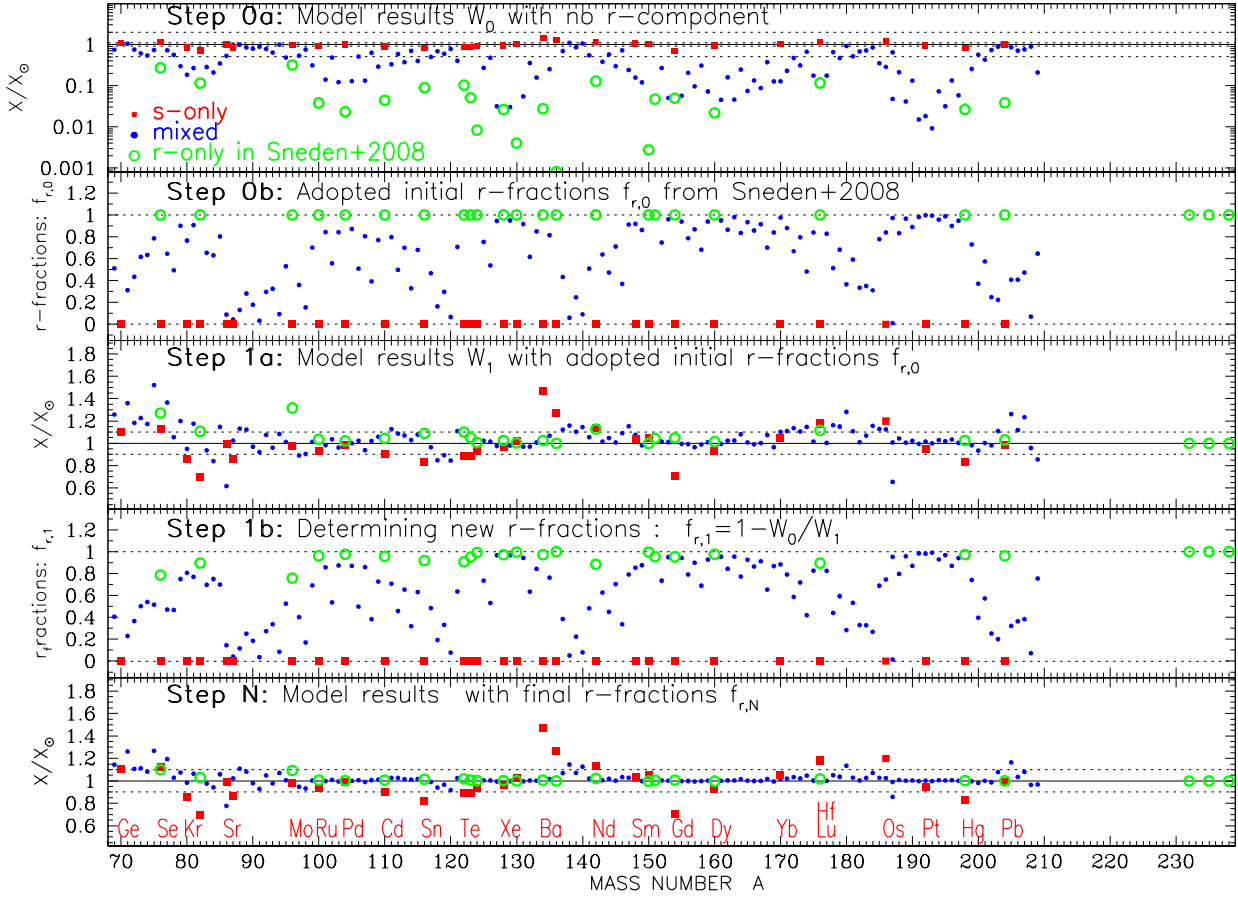
Figure 1. Top: Model results W_0 after Step 0, without r-component (see text); horizontal dashed lines indicate levels of \pm 10\% and a factor of 2 deviation from solar; 2 nd from top: Adopted initial r-fractions from Sneden et al. (2008); 3 rd from top: Results W_1 after Step 1, with r-component introduced from Sneden et al. (2008); horizontal dashed lines indicate levels of \pm 10\% deviation from solar; 4 th from top: Our r-component after Step 1 is obtained as r_1 = 1 - W_0/W_1 (where the corresponding s-component is obtained first as s_1 = W_0/W_1 ) and is introduced in the next iteration; Bottom: Same as the 3d panel, after the final ( N=17 here) iteration of our "bootstrap" method; horizontal dashed lines indicate levels of \pm 10\% deviation from solar. Note that the scale in the Y-axis changes in the different panels. The names of the elements with s- only isotopes are indicated in the bottom panel.
