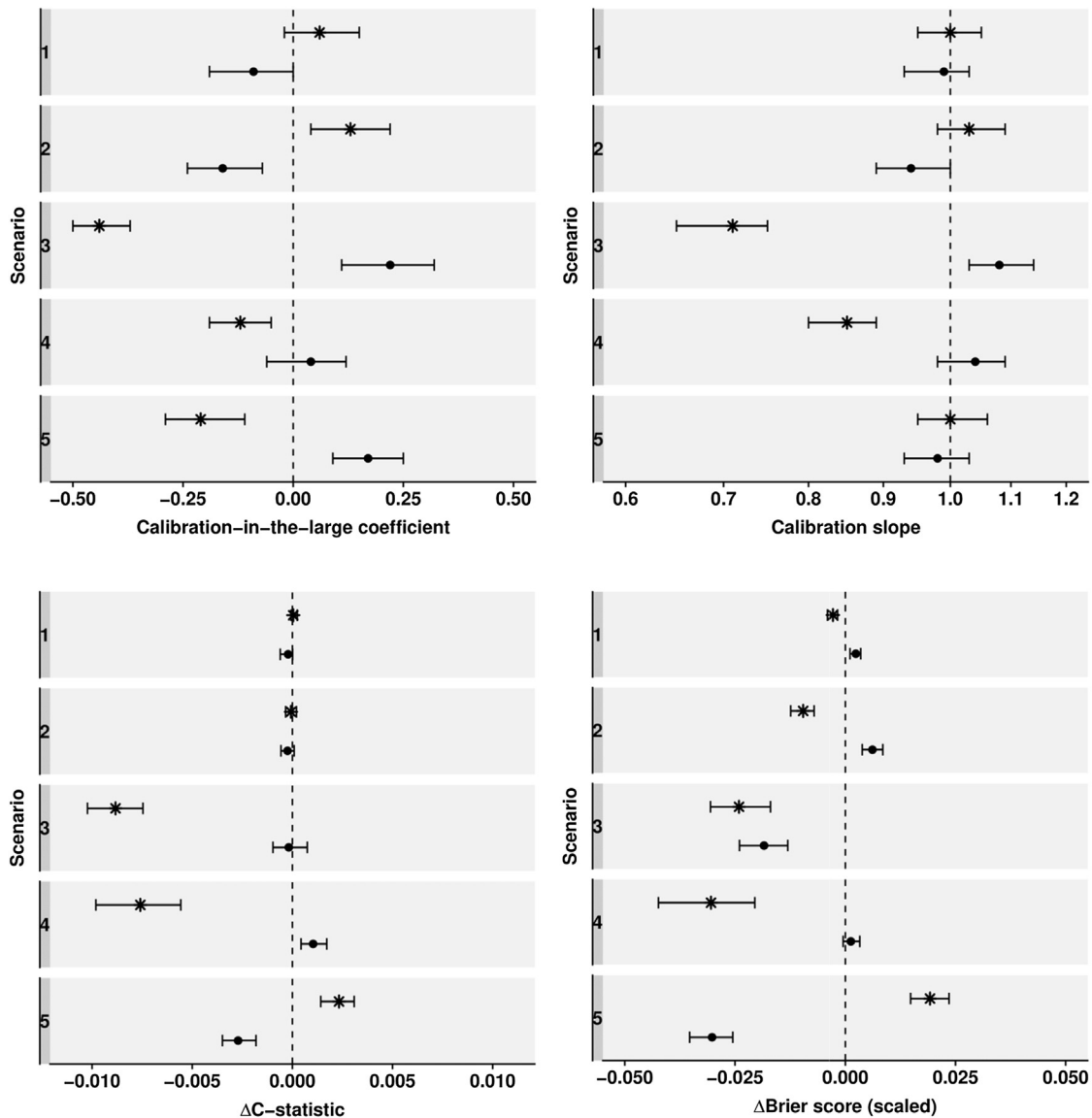
Fig. 2. Measures of predictive performance under predictor measurement heterogeneity of a model predicting the probability of having ovarian mass malignancy. The model is applied to the International Ovarian Tumor Analysis (IOTA) dataset, containing information on 5,914 nonpregnant women (1999–2012). Error bars represent the 95-percentile interval over 500 bootstrap samples. Error bars with an asterisk (*) indicate scenarios 1a–5a, meaning the model was derived using the preferred measurement and validated using the pragmatic measurement, scenarios with a point (●) indicate scenarios 1b–5b, meaning the model was derived using the pragmatic measurement and validated using the preferred measurement.
