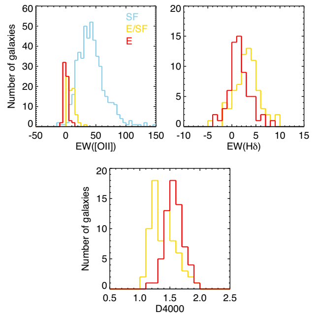
Figure 8. Distribution of spectral index measurements for galaxies with spectroscopic redshifts. Top left: \text{EW}(\text{OII}) for all galaxies colour-coded by their spectral type (‘E’ in red, ‘E/SF’ in orange, and ‘SF’ in blue). Top right and bottom: \text{EW}(\text{H}\delta) and \text{D4000} , respectively, for passive galaxies (‘E’ and ‘E/SF’).
