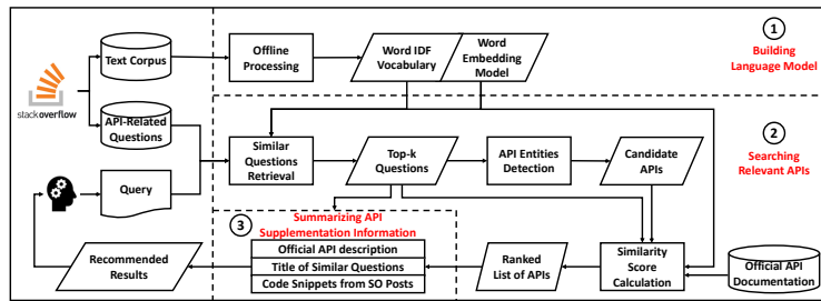
Figure 1: Overall framework of BIKER
