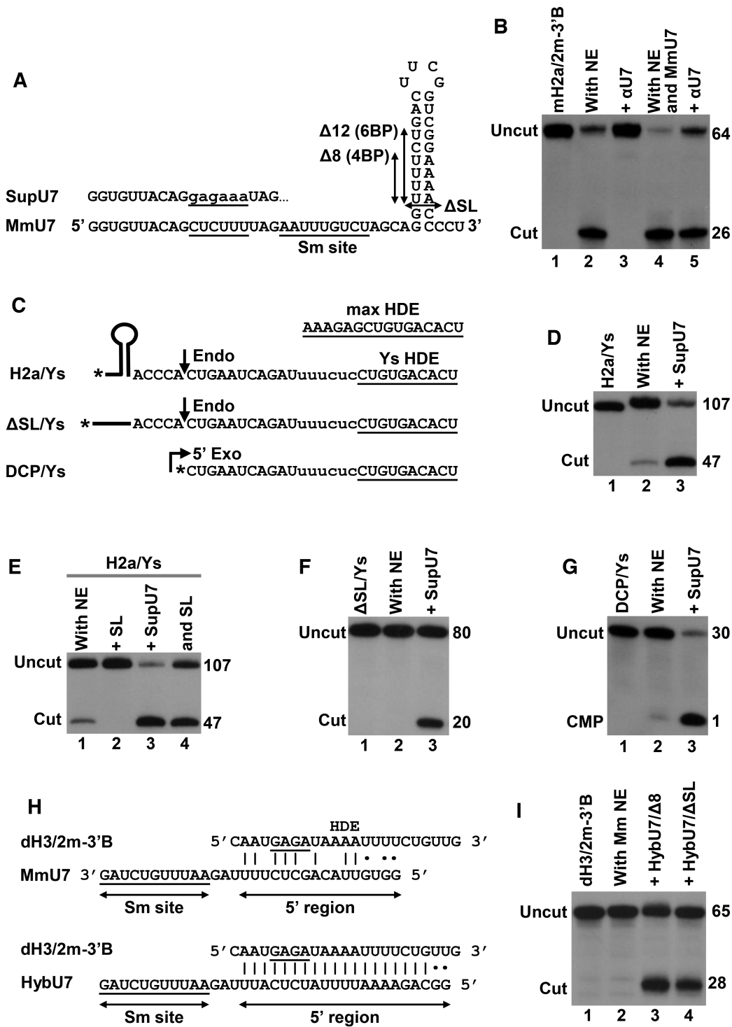
Figure 4. Altering substrate specificity of semi-recombinant holo U7 snRNP. (A) Sequence and structural organization of mouse U7 snRNA. The CU-CUUU pyrimidine core of mouse (Mm) U7 snRNA and the nucleotide substitution (lower case letters) in the suppressor U7 snRNA (SupU7) are underlined. Deletions within the 3' terminal stem-loop are indicated with double-headed arrows. (B) Processing of mH2a/2m-3'B pre-mRNA in a mouse nuclear extract (NE) alone or in the presence of an oligonucleotide blocking U7 snRNA ( \alpha U7) and/or recombinant core MmU7 snRNP. Lane 1 contains mH2a/2m-3'B pre-mRNA alone. (C) Changing six purines in an improved HDE of H2a histone pre-mRNA (max HDE) to six complementary pyrimidines (Ys, indicated with lower case letters) reduces the number of base pairs formed with endogenous U7 snRNA from 16 to 10 (underlined in the sequence). The three RNA substrates share the same mutated HDE but differ at 5' end, with H2a/Ys containing normal stem-loop, \Delta SL containing a 20-nucleotide unstructured region instead of the stem-loop, and DCP/Ys beginning immediately downstream of the cleavage site. Asterisks indicate the position of ^{32} P label. (D-G) Processing of the mutant RNA substrates shown in panel C in a mouse nuclear extract (NE) alone or in the presence of SupU7 snRNP. (H) Base pairing potential between Drosophila -specific dH3/2m-3'B pre-mRNA and MmU7 or HybU7 snRNAs. Watson-Crick and G-U base pairs are represented by vertical lines and dots, respectively. The purine core of Drosophila HDE is underlined. (I). Processing of dH3/2m-3'B pre-mRNA in a Mm NE alone or in the presence of indicated semi-recombinant U7 snRNPs.
