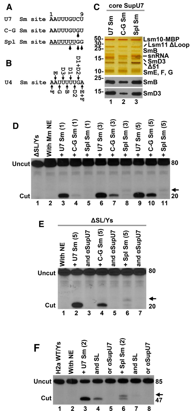
Figure 7. In vitro assembly of the U7-specific ring on a spliceosomal Sm site. (A) Nucleotide sequence of the U7-specific Sm site (top sequence) and changes made to generate C-G and spliceosomal-type (Spl) Sm sites (bottom sequences). Mutated nucleotides are indicated with the arrows. (B) Interaction between the spliceosomal Sm proteins and individual nucleotides of the Sm site in U4 snRNA (50). (C) Proteins of the U7-specific Sm ring bound to the U7, C-G and Spl Sm sites visualized by silver staining (top) and Western blotting (bottom). (D) Processing of \Delta SL/Ys pre-mRNA in a mouse nuclear extract in the presence of 1, 3 and 5 \mu l of peak fraction containing indicated core U7 snRNPs. The arrow denotes the unusual cleavage product generated by SupU7 snRNP containing Spl Sm site. (E, F) Processing of \Delta SL/Ys (panel E) and H2a WT/Ys (panel F) pre-mRNAs in a mouse nuclear extract in the presence of 5 or 2 \mu l of indicated core SupU7 snRNPs and processing competitors (SL or \alpha SupU7).
