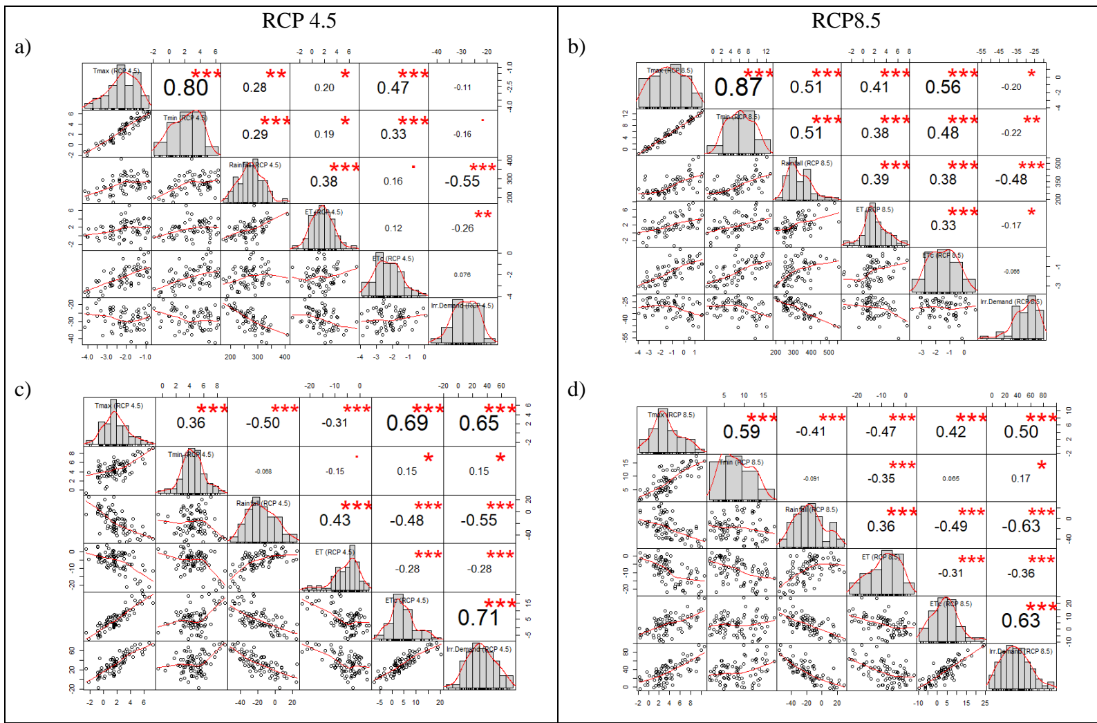
Figure 4-9. Kendall's tau correlation matrix among different variables for the REMO model; (a) and (b) for the dry season, and (c) and (d) for the wet season with p-values 1, * 0.05, **0.01, ***0.001, and ***0.
