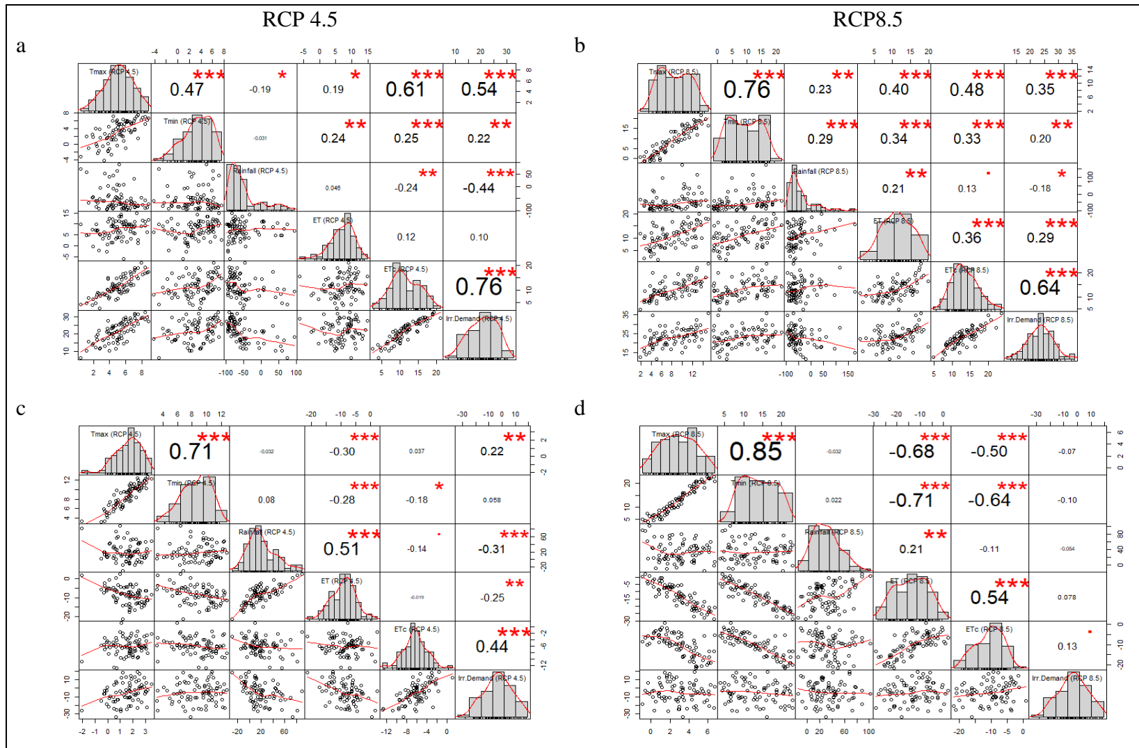
Figure 4-8. Kendall's tau correlation matrices among different variables for the RCA4 model; (a) and (b) for the dry season, and (c) and (d) for the wet season with p-values 1, * 0.05, **0.01, ***0.001, and ***0.
