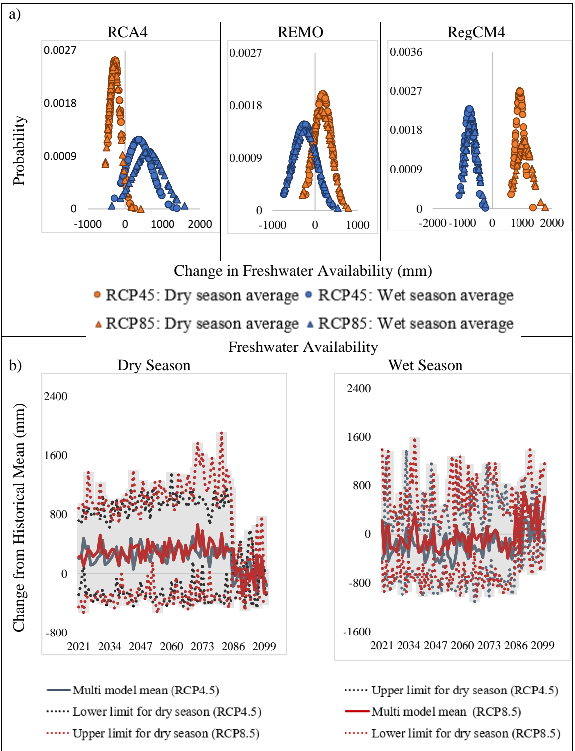
Figure 4-14. Plots showing the probability density function of freshwater availability in (a) and the uncertainty of freshwater availability for regional climate models in (b).
