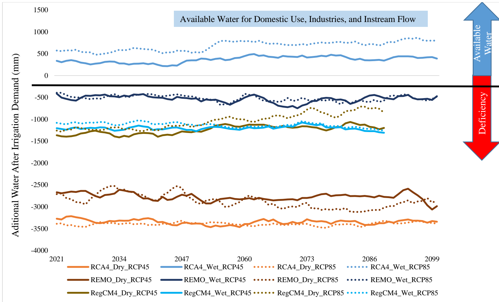
Figure 4-15. Climatic impact on freshwater availability (FWA) after fulfilling the irrigation requirement. Here, FWA is the multi-decadal mean of [(Rainfall-Evapotranspiration) - irrigation demand].
