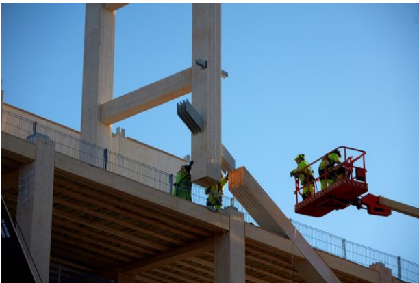
Figure 5: Large steel plate and dowel connections of the Mjøstårnet building. Image: Jens Haugen/Anti.
