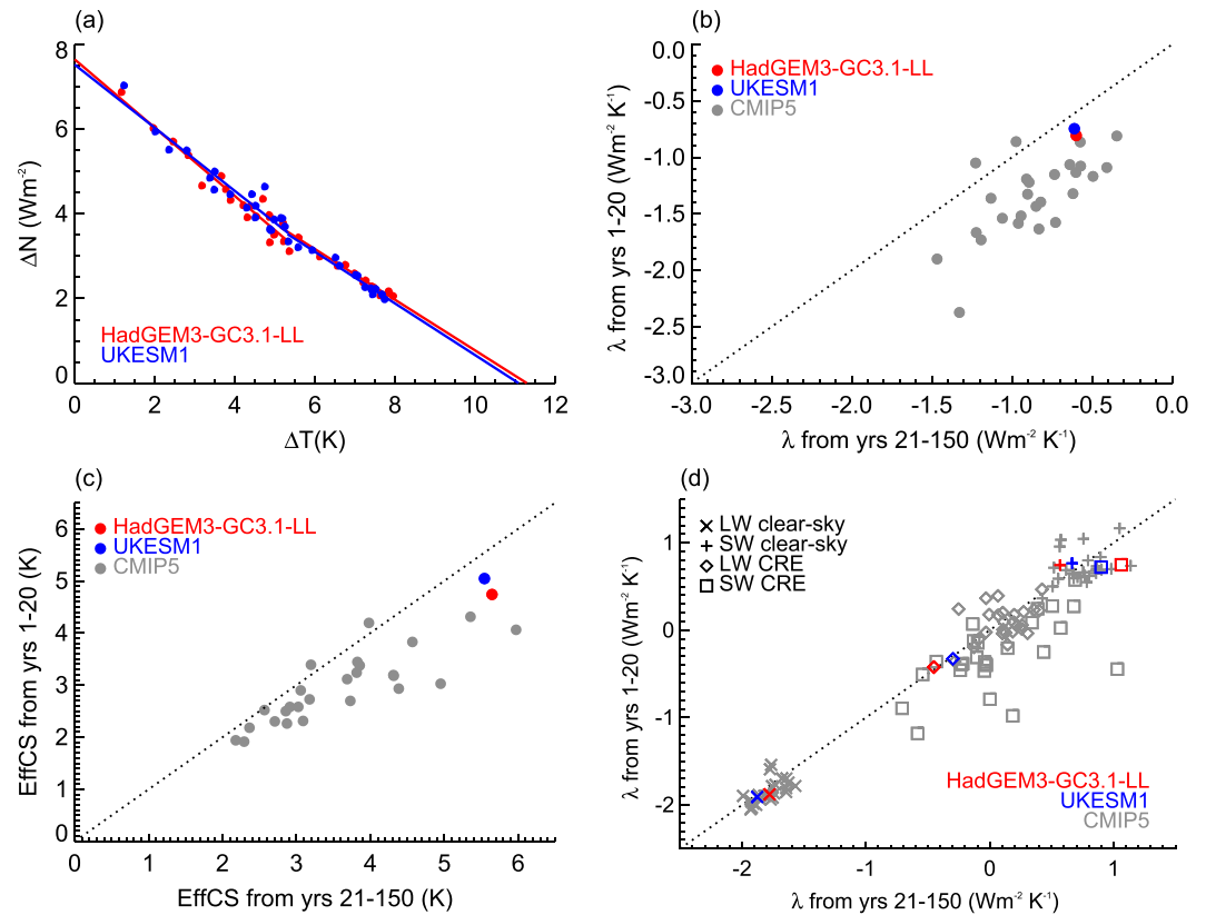
Figure 6. (a) Gregory plot separated at year 20, that is, a linear regression fit for years 1–20 and 21–150, for HadGEM3-GC3.1-LL and UKESM1 abrupt-4xCO 2 simulations. (b) Comparison of the feedback parameter derived the two time periods across models. (c) Comparison of the EffCS derived from the two time periods. (d) Comparison of the feedback parameter components derived the two time periods across models.
