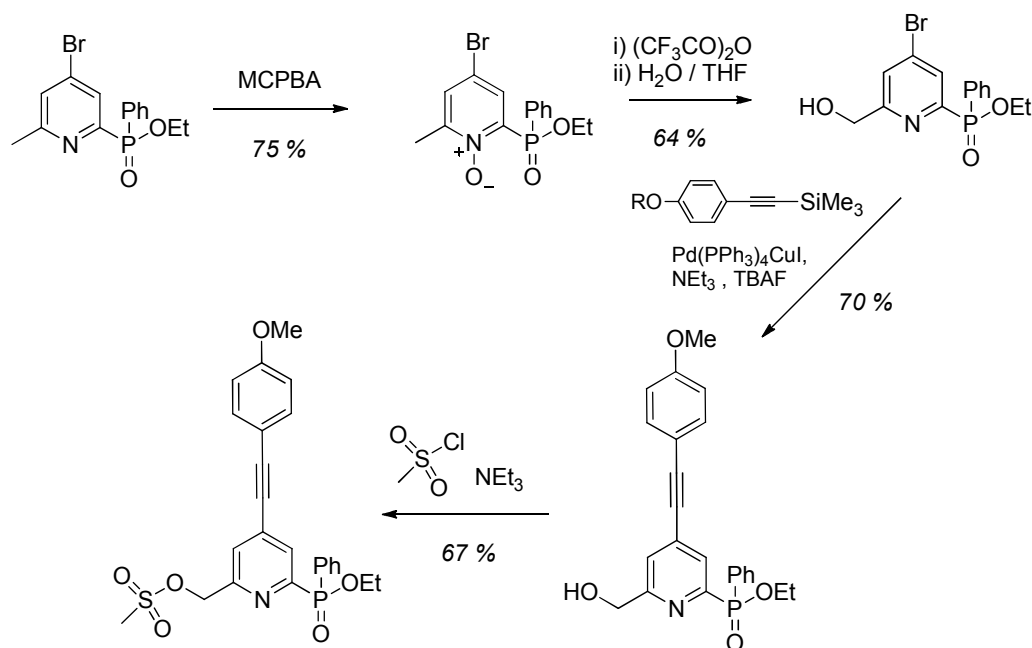
Scheme 5.10
