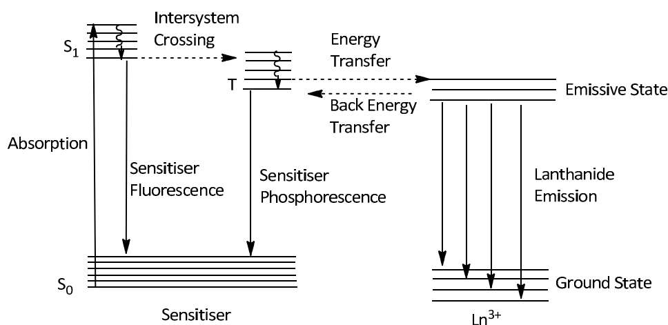
Figure 1.6 Jablonski diagram showing the processes of sensitised emission.
