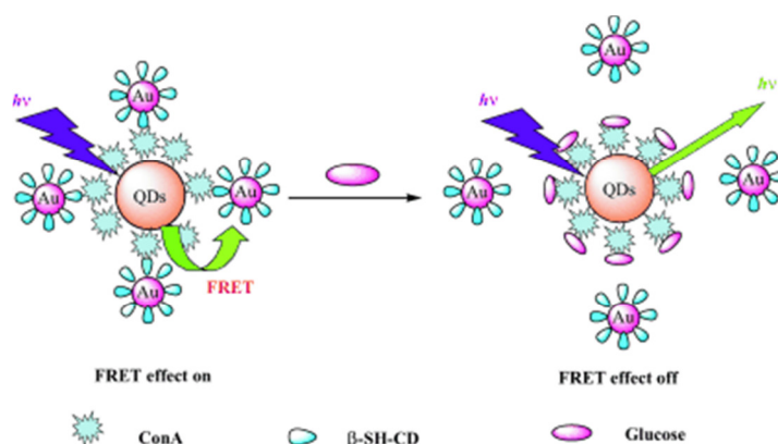
Figure 1.12 Schematic illustration of FRET between a QD and a gold nanoparticle which is inhibited by the presence of glucose.
