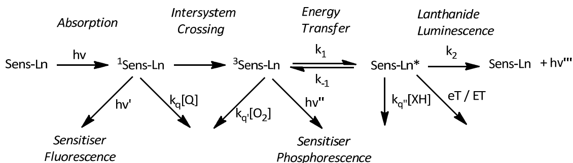
Scheme 1.1
