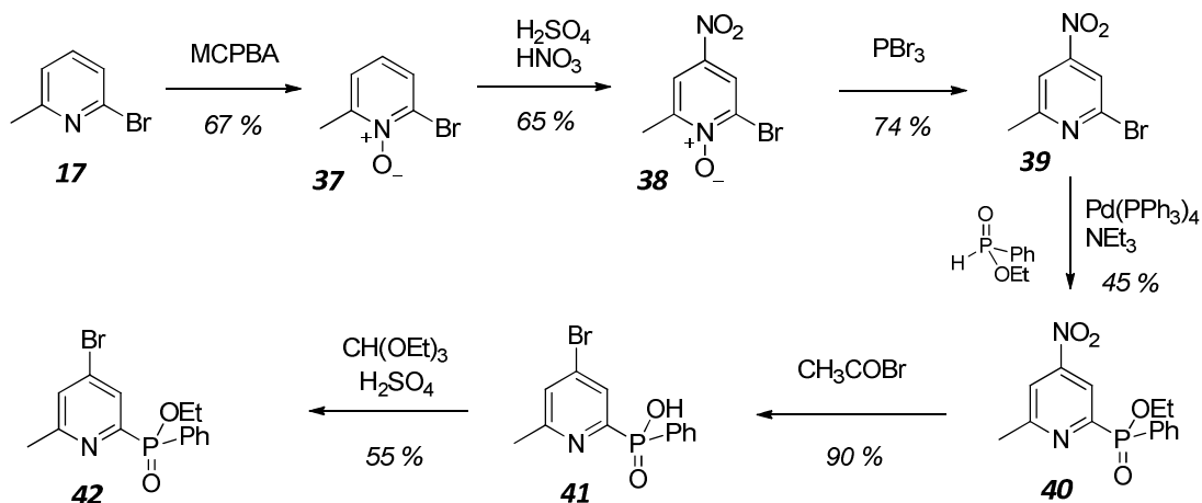
Scheme 5.4
