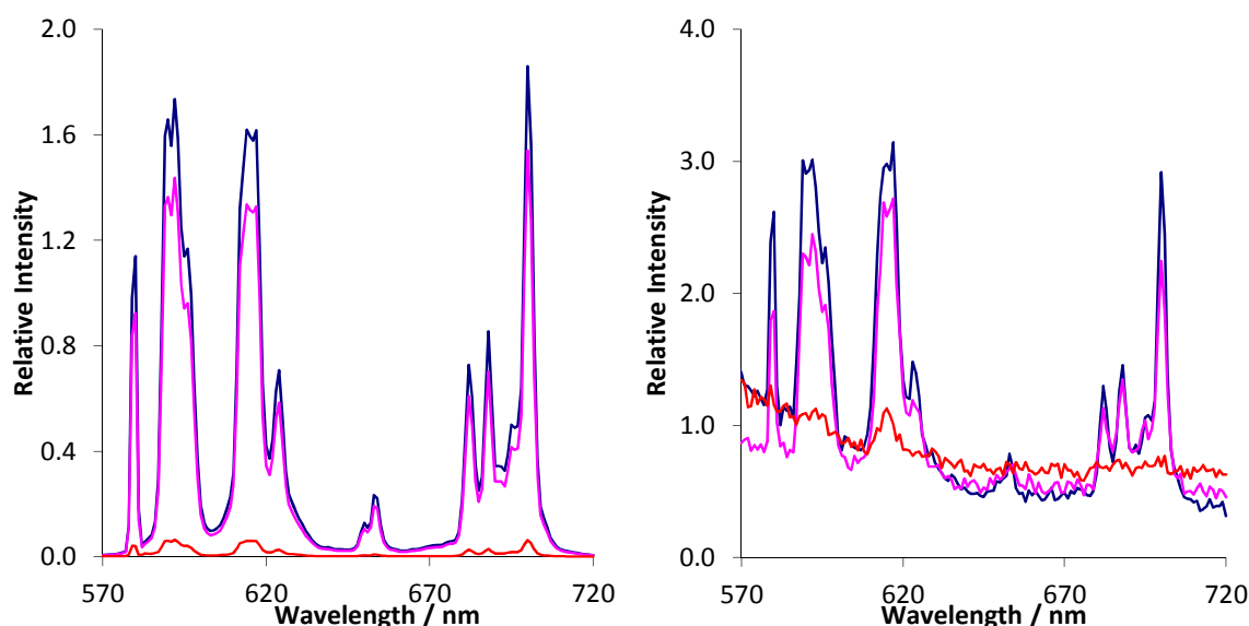
Figure 6.1 Emission spectra for [\text{Eu}\cdot\text{L}^1(\text{H}_2\text{O})] in the presence of 0 mM (blue), 0.1 mM (purple) and 10 mM (orange) \text{MnCl}_2 , following excitation at left ) 328 nm and right ) 398 nm ( \text{H}_2\text{O} , 100 \mu\text{M} complex, 0.1 M HEPES, 0.1 M NaCl, pH 7.4, 295 K).
