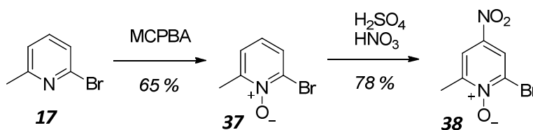
Scheme 5.2
