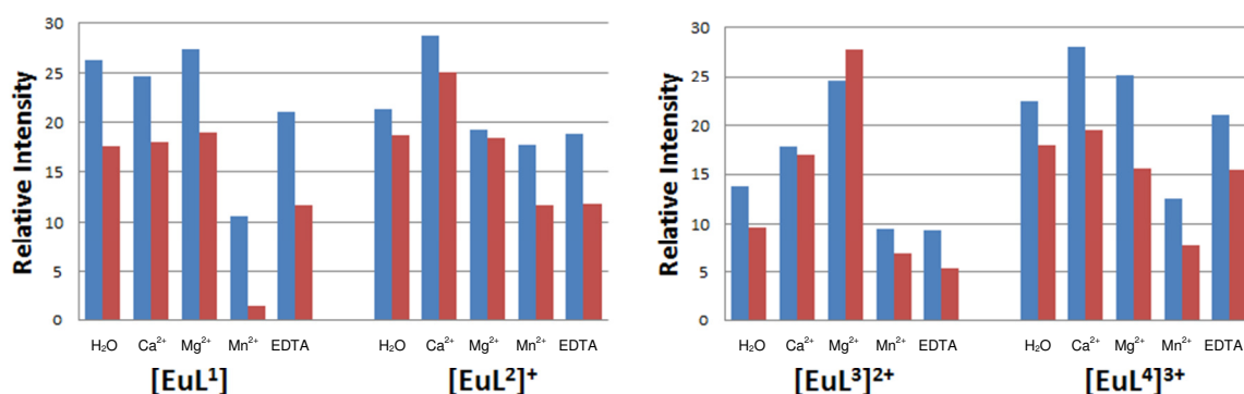
Figure 2.9 Changes in \text{Eu}^{3+} emission intensity after 15 min (blue) or 18h (red) in the presence of the stated additives (10nM complex, 20mM additive, \lambda_{\text{ex}} = 335 nm, \lambda_{\text{em}} = 620 nm).
