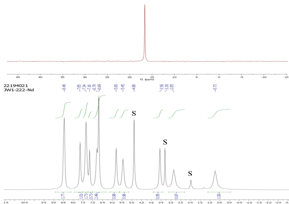
Figure 4.6 ^1\text{H} -( lower ) and ^{31}\text{P} -( upper ) NMR spectra for [\text{Nd}\cdot\text{L}^9] ( \text{CD}_3\text{OD} , 400 MHz, 295 K, pD 5.8). Residual solvent peaks are labelled S.
