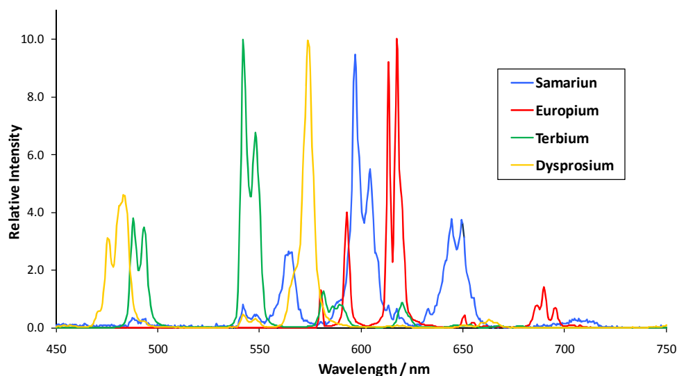
Figure 4.12 Emission spectra of the four emissive complexes in the [\text{Ln}\cdot\text{L}^9] series ( \text{H}_2\text{O} , \lambda_{\text{ex}} = 274\text{ nm} , pH 5.8). Spectra have been scaled so that the maximum intensity is equal in each case.
