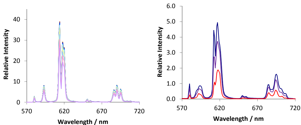
Figure 6.9 Luminescence titrations for [\text{Eu}\cdot\text{L}^{12}] (left) and [\text{Eu}\cdot\text{L}^{13}(\text{H}_2\text{O})]^+ (right) with increasing urate concentrations ( \text{H}_2\text{O} : \text{CH}_3\text{OH} , 3 : 1, 8 \mu\text{M} complex, 0 – 300 \mu\text{M} urate, 0.1 M HEPES, 0.1 M NaCl, pH 7.4, 295 K). For [\text{Eu}\cdot\text{L}^{13}(\text{H}_2\text{O})]^+ , only the emission spectra at 0 (blue), 15 (purple) and 300 \mu\text{M} (red) are shown.
