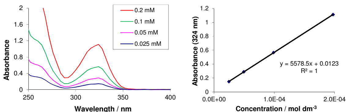
Figure 2.5 left ) Absorption of 2-methyl-3-azaxanthone at four concentrations (MeOH, 295 K) and right ) absorbance at \lambda_{\text{max}} as a function of concentration, allow calculation of the molar extinction coefficient.
