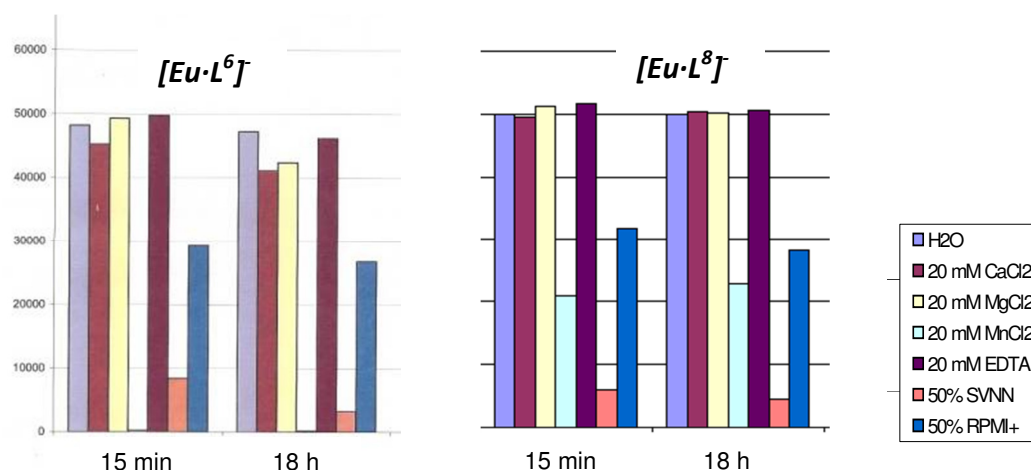
Figure 3.6 Stability data for [\text{Eu}\cdot\text{L}^6]^- (left) and [\text{Eu}\cdot\text{L}^8]^- (right) in HEPES buffer or at two time points, 15 min and 18 h (10nM complex, \lambda_{\text{ex}} = 335 \text{ nm} , \lambda_{\text{em}} = 620 \text{ nm} ).
