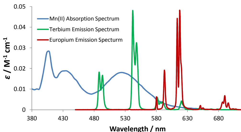
Figure 6.5 Molar extinction coefficient for \text{MnCl}_2 (blue) as a function of wavelength ( \text{H}_2\text{O} , pH 7.4, 295 K). The emission spectra for [\text{Tb}\cdot\text{L}^9] (green) and [\text{Eu}\cdot\text{L}^9] (red) are shown to allow analysis of the spectral overlap integral.
