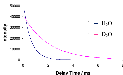
Figure 2.7 Emission decay curves of [\text{Eu}\cdot\text{L}^1(\text{H}_2\text{O})] in \text{H}_2\text{O} and \text{D}_2\text{O} , allowing calculation of k and \tau .
