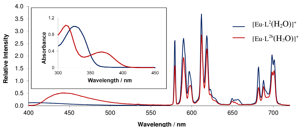
Figure 2.12 Comparison of the absorption (insert) and emission spectra of [\text{Eu}\cdot\text{L}^2(\text{H}_2\text{O})]^+ ( \lambda_{\text{ex}} = 328 \text{ nm} ) and [\text{Eu}\cdot\text{L}^{2b}(\text{H}_2\text{O})]^+ ( \lambda_{\text{ex}} = 368 \text{ nm} ) ( \text{H}_2\text{O} , pH 5.8, 295 K).
