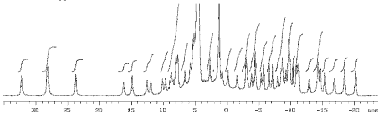
Figure 2.2 ^1\text{H-NMR} analysis of [\text{Eu}\cdot\text{L}^1(\text{H}_2\text{O})] (400 MHz, \text{D}_2\text{O} , pD 5.8).
