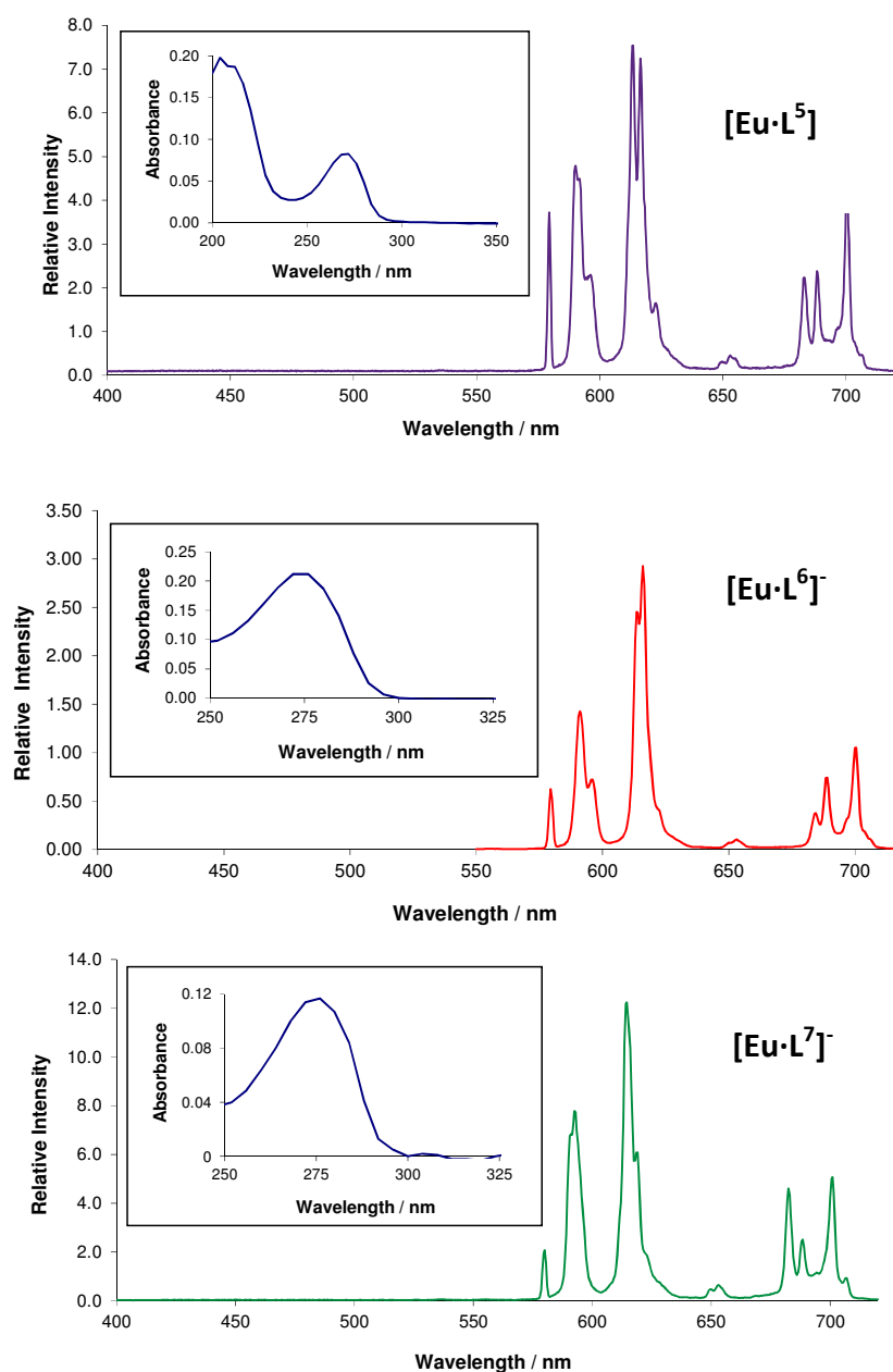
Figure 3.2 Absorption ( insert ) and emission spectra for the three complexes, [Eu·L 5 ], [Eu·L 6 ] - and [Eu·L 7 ] - . All spectra recorded in H 2 O ( \lambda_{\text{ex}} = 275 nm, 20 \mu\text{M} , pH 5.8, 295 K).
