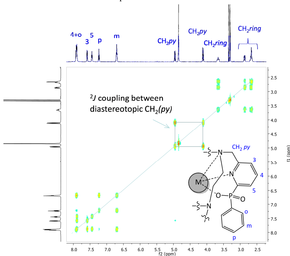
Figure 4.8 ^1\text{H} -COSY spectrum of [\text{Y}\cdot\text{L}^9] ( \text{CD}_3\text{OD} , 500 MHz, pD 5.8).
