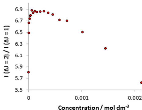
Figure 5.17 Integrated intensity ratio of \Delta J = 2 : \Delta J = 1 as a function of [HSA] (10 \mu\text{M} complex, \text{H}_2\text{O} : \text{CH}_3\text{OH} , 3 : 1, pH 7.4, 295 K).
