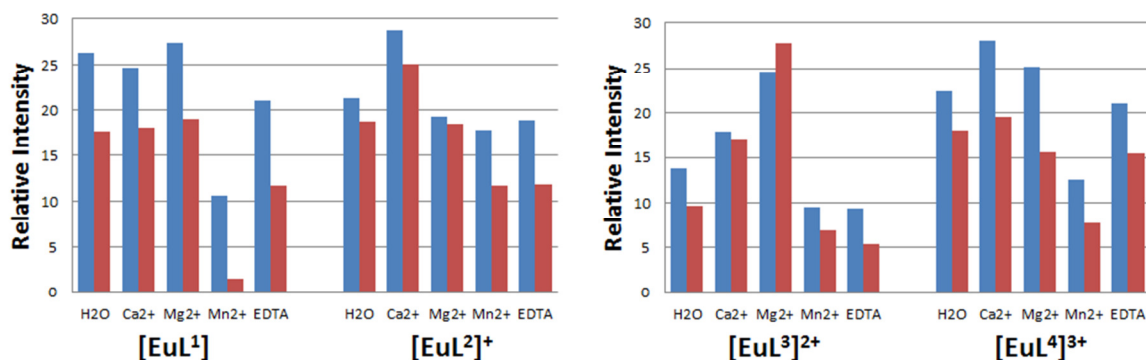
a) Changes in Eu 3+ emission intensity after 15 min (blue) or 18h (red) in the presence of the stated additives (10nM complex, 20mM additive, λ ex = 335 nm, λ em = 620 nm).
