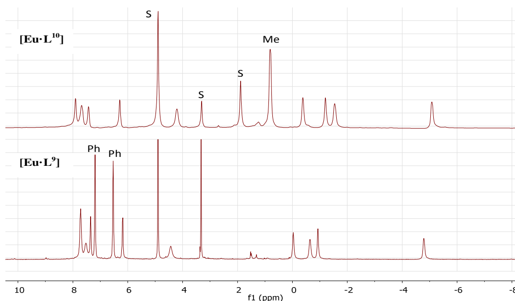
Figure 4.20 ^1\text{H} -NMR spectra of [\text{Eu}\cdot\text{L}^{10}] (upper) and [\text{Eu}\cdot\text{L}^9] (lower) ( \text{CD}_3\text{OD} , 400 MHz).
