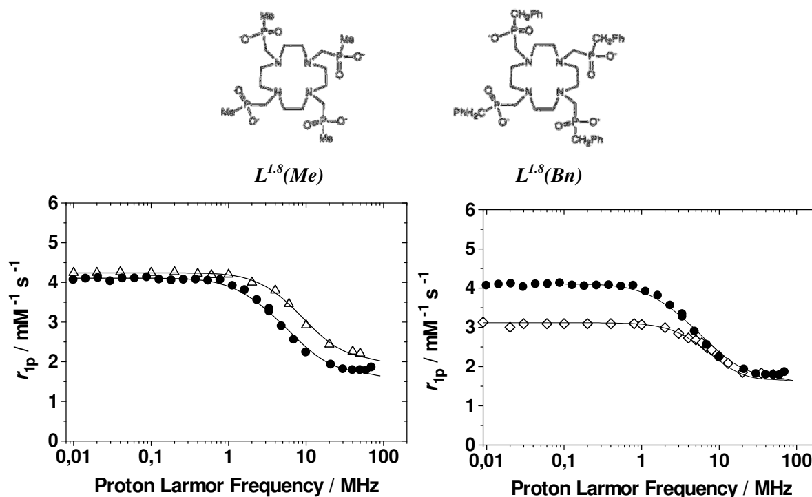
Figure 4.23 Comparison of the NMRD profile of [\text{Gd}\cdot\text{L}^{10}] (●) with that of [\text{Gd}\cdot\text{L}^{1.8}(\text{Me})]^- (Δ, left) and [\text{Gd}\cdot\text{L}^{1.8}(\text{Bn})]^- (◇, right).
