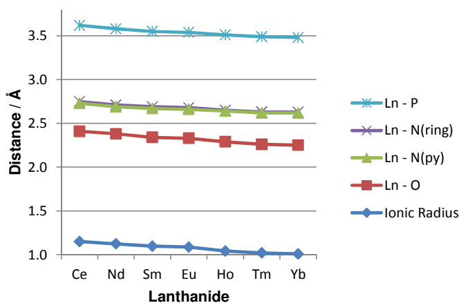
Figure 4.5 Bond distances and ionic radii of the seven isostructural [\text{Ln}\cdot\text{L}^9] complexes.
