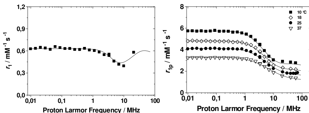
Figure 4.22 NMRD profiles for [\text{Gd}\cdot\text{L}^9] (90 : 10, \text{H}_2\text{O}/\text{CH}_3\text{OH} , left) and [\text{Gd}\cdot\text{L}^{10}] ( \text{H}_2\text{O} ) with varying temperature (right).
