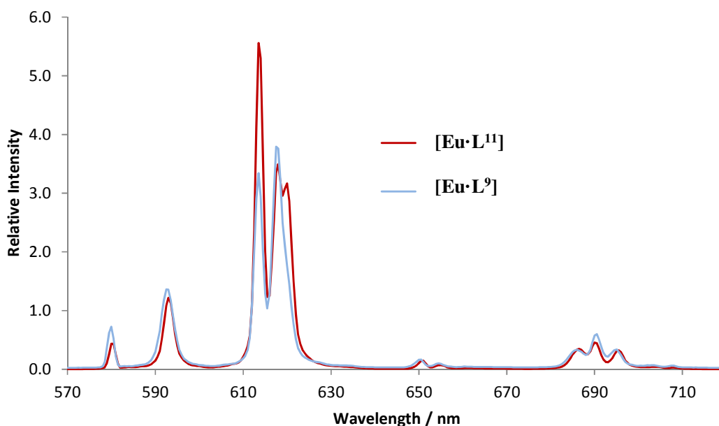
Figure 5.7 Comparison of the emission spectra of [Eu·L 11 ] (red, \lambda_{\text{ex}} = 332 nm, MeOH, 295 K) and [Eu·L 9 ] (blue, \lambda_{\text{ex}} = 274 nm, MeOH, 295 K). Spectra have been scaled so that the total integrated emission is the same in each case.
