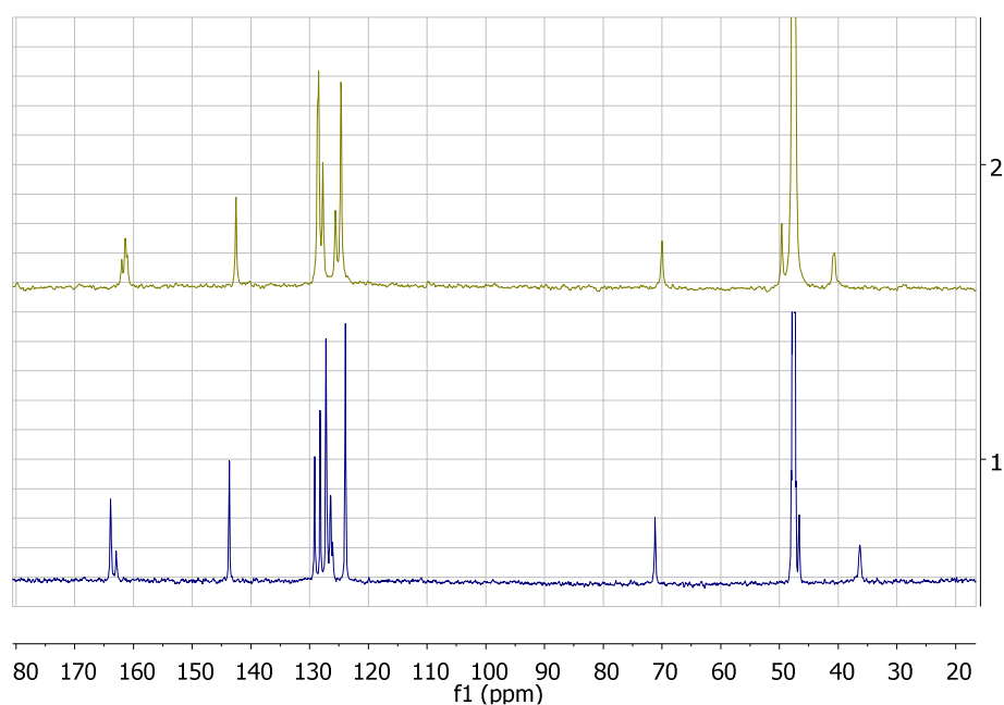
Figure 4.11 ^{13}\text{C} -NMR spectrum of [\text{Yb}\cdot\text{L}^9] at 22 °C (lower) and 50 °C (upper, \text{CD}_3\text{OD} , 400 MHz, pD 5.8)
