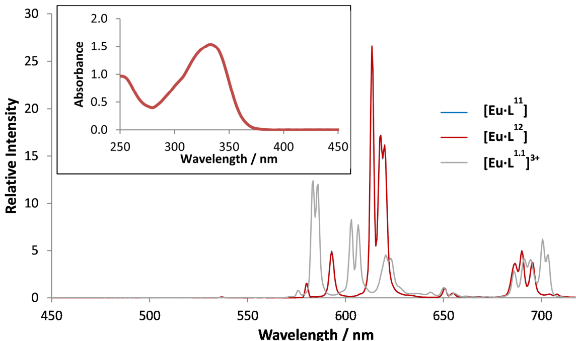
Figure 5.12 Comparison of the emission spectra of [\text{Eu}\cdot\text{L}^{11}] ( \text{CH}_3\text{OH} , \lambda_{\text{ex}} = 332 \text{ nm} , 295 K), [\text{Eu}\cdot\text{L}^{12}] ( \text{H}_2\text{O} : \text{CH}_3\text{OH} , 1 : 3, \lambda_{\text{ex}} = 332 \text{ nm} , 295 K) and [\text{Eu}\cdot\text{L}^{1.1}]^{3+} ( \text{H}_2\text{O} , 0.4 M KF, \lambda_{\text{ex}} = 303 \text{ nm} , 295 K) and insert ) absorption spectrum for [\text{Eu}\cdot\text{L}^{12}] ( \text{H}_2\text{O} : \text{CH}_3\text{OH} , 3 : 1, 295 K).
