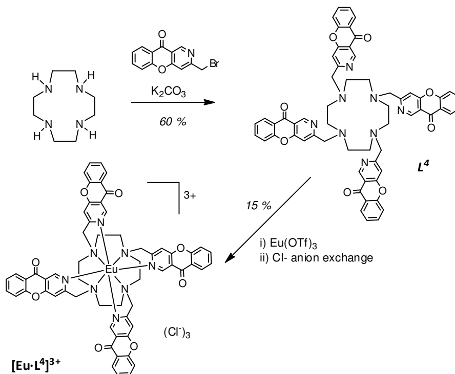
Scheme 2.7
