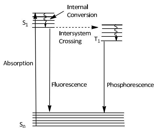
Figure 1.2 Jablonski diagram showing the important processes in photoluminescence.
