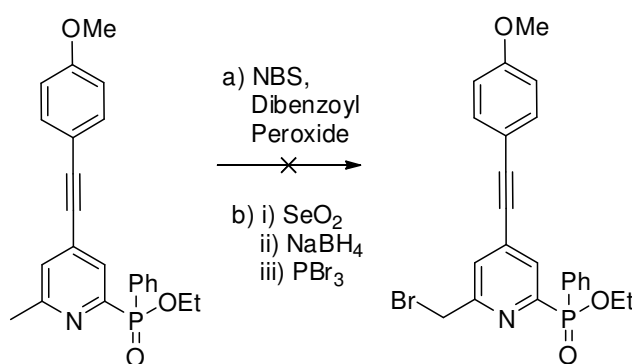
Scheme 5.6
