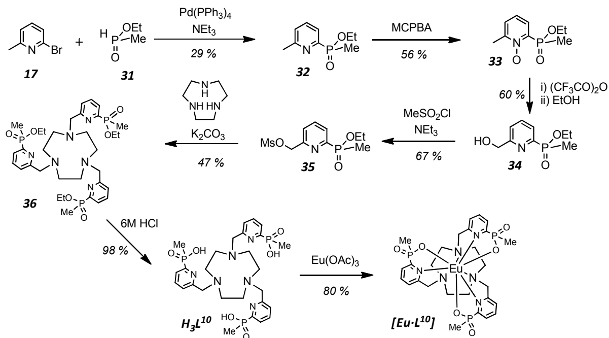
Scheme 4.3
