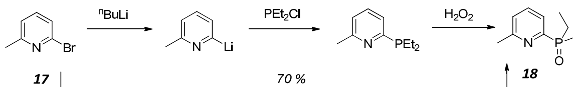
Scheme 3.1
