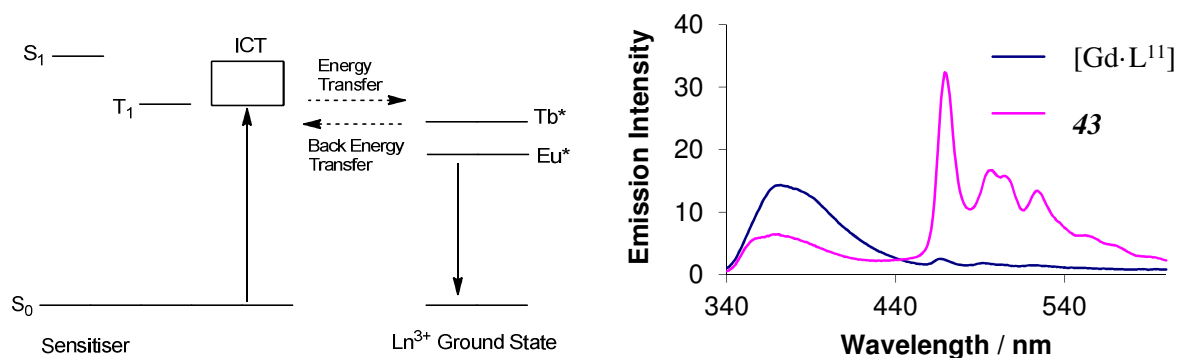
Figure 5.11 left) Jablonski diagram showing the proposed sensitised emission pathway and right) the 77 K emission spectra of [\text{Gd}\cdot\text{L}^{11}] (blue) and the arylalkynylpyridyl chromophore 43 in (EPA glass, \lambda_{\text{ex}} = 320 nm).
