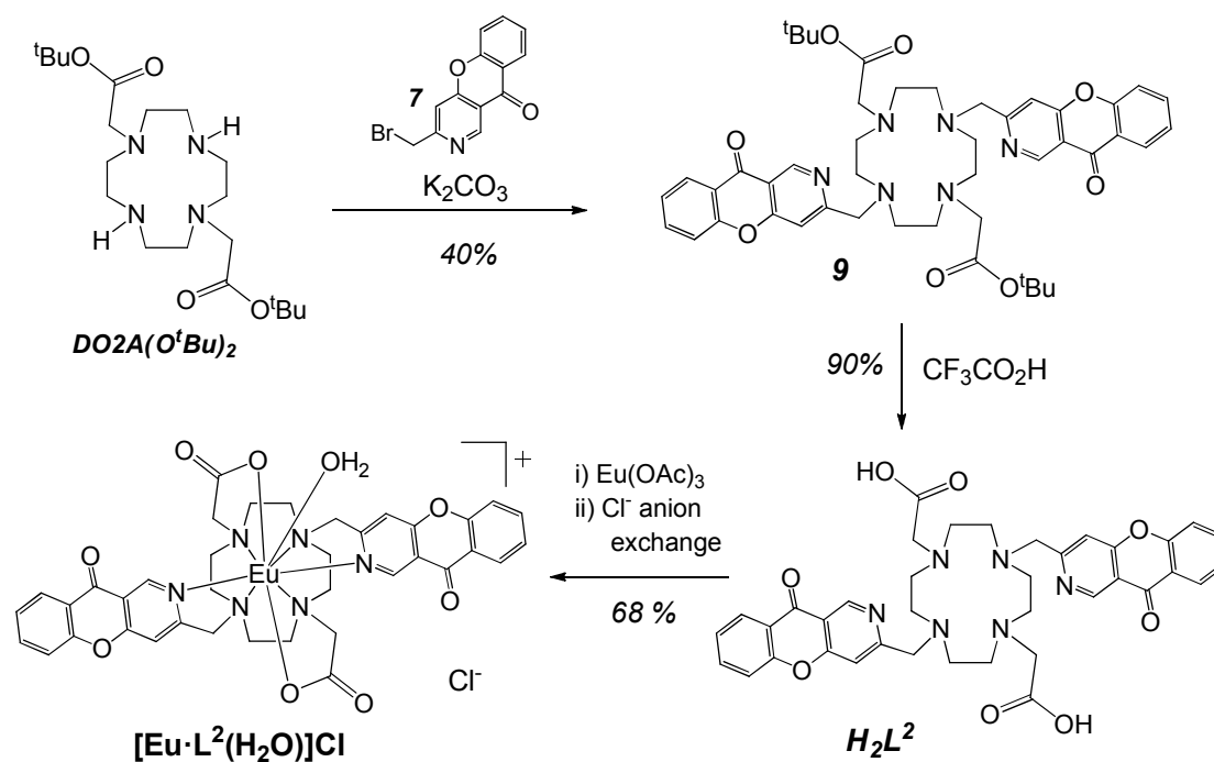
Scheme 2.5
