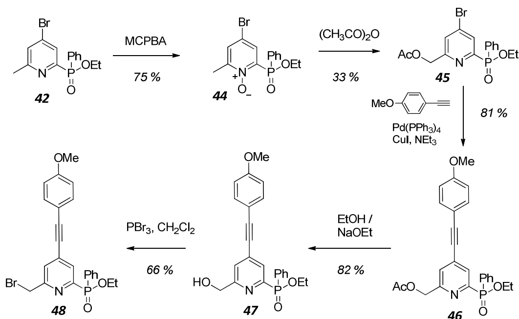
Scheme 5.7
