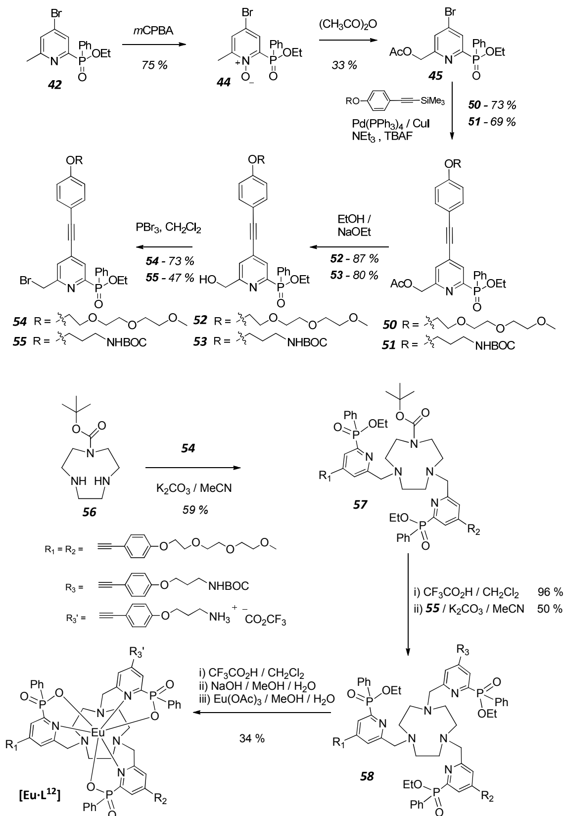
Scheme 5.9
