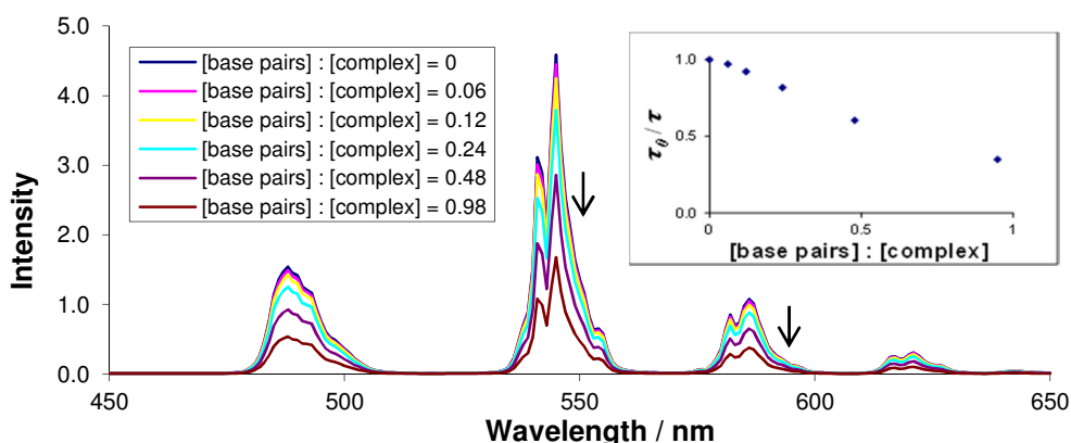
Figure 2.11 Luminescence titration of [\text{Tb}\cdot\text{L}^2(\text{H}_2\text{O})]^+ with DNA ( \text{H}_2\text{O} , pH 7.4, 295K) and insert ) Variation in the excited state lifetime as a function of added DNA.
