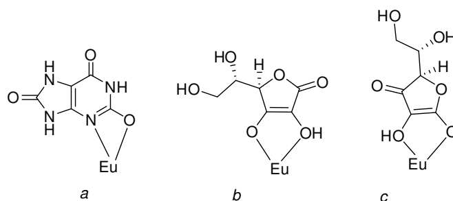
Figure 6.11 Potential binding modes of urate and ascorbate to the \text{Eu}^{3+} centre of [\text{Eu}\cdot\text{L}^{13}]^+ .
