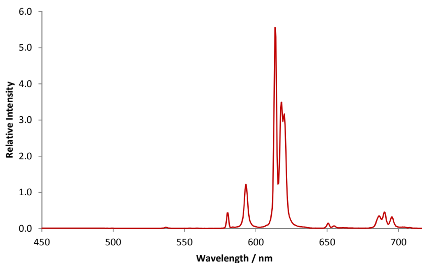
Figure 5.6 Emission spectrum for [\text{Eu}\cdot\text{L}^{11}] (MeOH, \lambda_{\text{ex}} = 332 \text{ nm} , 295 K).
