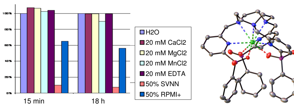
Figure 4.14 left) Stability data for [\text{Eu}\cdot\text{L}^9] in HEPES buffer at two time points, 15 min and 18 h (10nM complex, \lambda_{\text{ex}} = 335 nm, \lambda_{\text{em}} = 620 nm) and right) a side view of the crystal structure of [\text{Eu}\cdot\text{L}^9] , showing the three shielding Ph groups.
