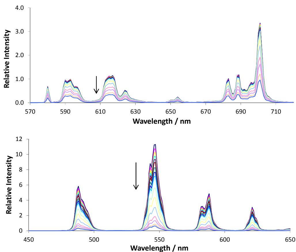
Figure 6.3 Luminescence titrations for [\text{Eu}\cdot\text{L}^1(\text{H}_2\text{O})] (upper) and [\text{Tb}\cdot\text{L}^1(\text{H}_2\text{O})] (lower) with increasing concentration of \text{MnCl}_2 ( \text{H}_2\text{O} , 20\ \mu\text{M} complex, 0 - 3\ \text{mM} \text{MnCl}_2 , 0.1\ \text{M} HEPES, 0.1\ \text{M} NaCl, pH 7.4, 295\ \text{K} ).
