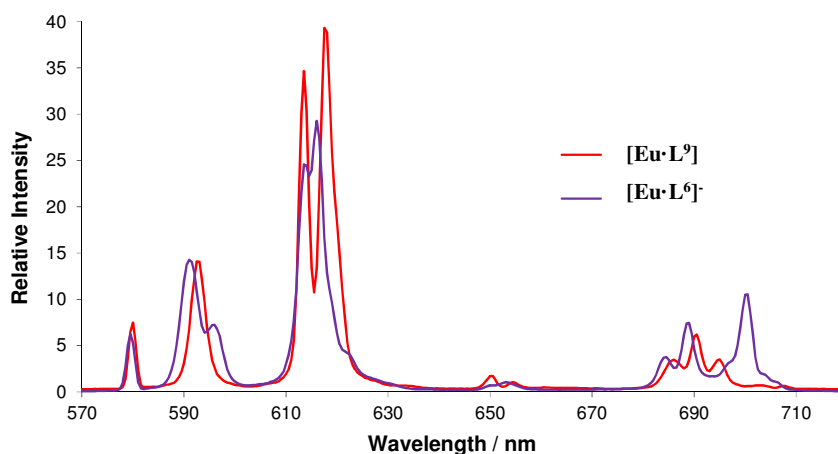
Figure 4.13 Comparison of the emission spectra of [\text{Eu}\cdot\text{L}^9] and [\text{Eu}\cdot\text{L}^6] ( \text{H}_2\text{O} , \lambda_{\text{ex}} = 274 nm, pH 5.8). Spectra have been scaled so that the total intensity integral is equal in each case.
