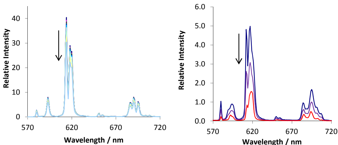
Figure 6.7 Luminescence titrations for [\text{Eu}\cdot\text{L}^{12}] (left) and [\text{Eu}\cdot\text{L}^{13}(\text{H}_2\text{O})]^+ (right) with increasing ascorbate concentrations ( \text{H}_2\text{O} : \text{CH}_3\text{OH} , 3 : 1, 8 \mu\text{M} complex, 0 – 10 mM ascorbate, 0.1 M HEPES, 0.1 M NaCl, pH 7.4, 295 K). For [\text{Eu}\cdot\text{L}^{13}(\text{H}_2\text{O})]^+ , only the emission spectra at 0 (blue), 60 (purple) and 940 \mu\text{M} (red) are shown.
