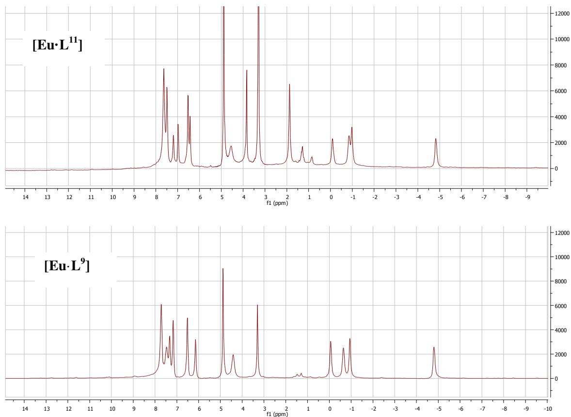
Figure 5.3 ^1\text{H-NMR} spectra of [\text{Eu}\cdot\text{L}^{11}] (upper) and [\text{Eu}\cdot\text{L}^9] (lower) (d-MeOD, 400 MHz, pD 6.2, 295 K).
