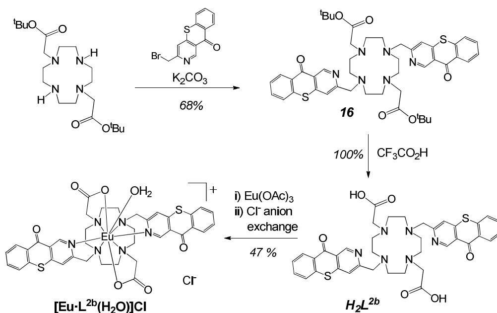
Scheme 2.9
