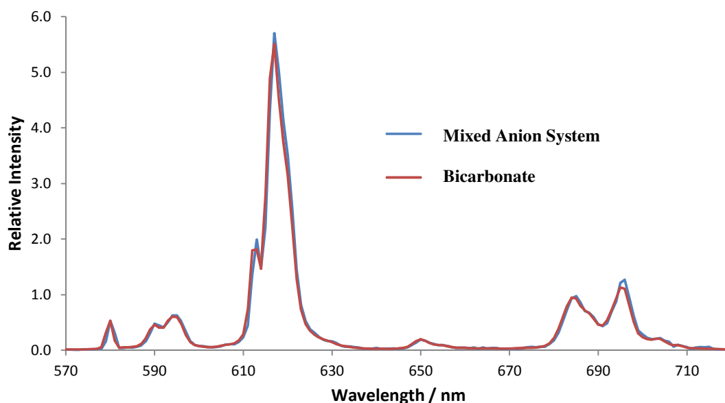
Figure 5.18 Comparison of the [\text{Eu} \cdot \text{L}^{13}(\text{H}_2\text{O})]^+ emission spectrum in the presence of bicarbonate ( red ) and a mixed anion system ( blue ), comprising sodium salts of bicarbonate (30 mM), citrate (0.13 mM), lactate (2.3mM) and hydrogen phosphate (1.3 mM) (0.1 M NaCl, pH 7.4, 295 K).
