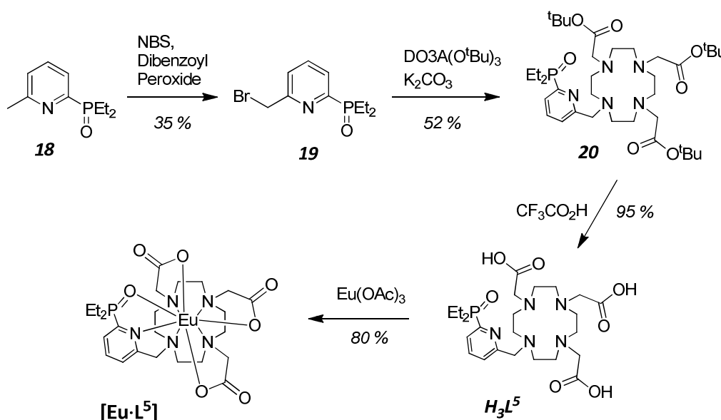
Scheme 3.2
