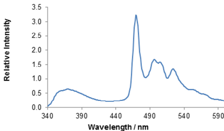
Figure 5.2 Emission spectrum of alkyne chromophore 43 at 77 K (EPA glass, \lambda_{\text{ex}} = 320 nm).
