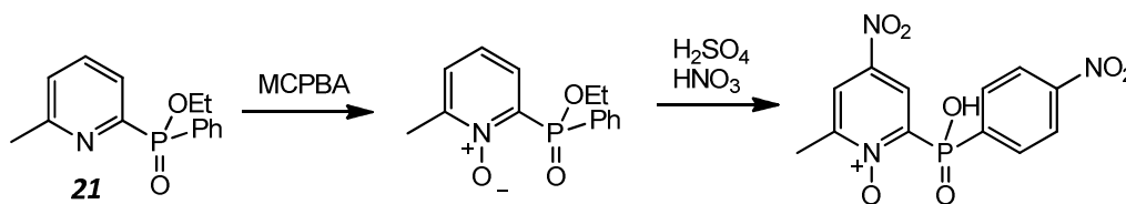
Scheme 5.1
