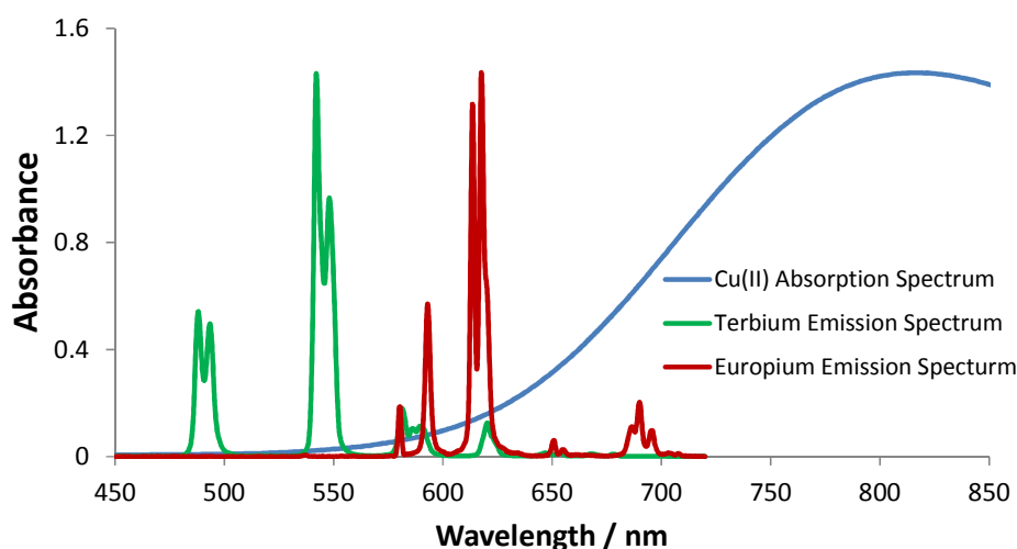
Figure 6.6 Absorption spectrum of \text{CuCl}_2 (blue) as a function of wavelength ( \text{H}_2\text{O} , pH 7.4, 295 K). The emission spectra for [\text{Tb}\cdot\text{L}^9] (green) and [\text{Eu}\cdot\text{L}^9] (red) are shown to allow analysis of the spectral overlap integral.
