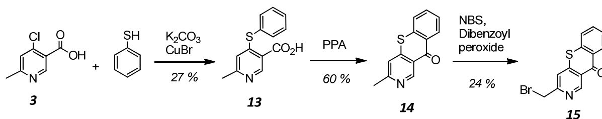
Scheme 2.8
