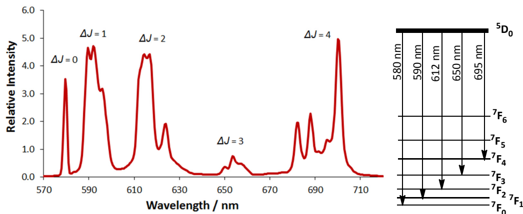
Figure 1.5 left ) A typical europium emission spectrum, with five transitions denoted by their \Delta J value. Further splitting within each transition is also observed and right ) the ^5D_0 and ^7F_J energy levels, giving rise to the europium emission.
