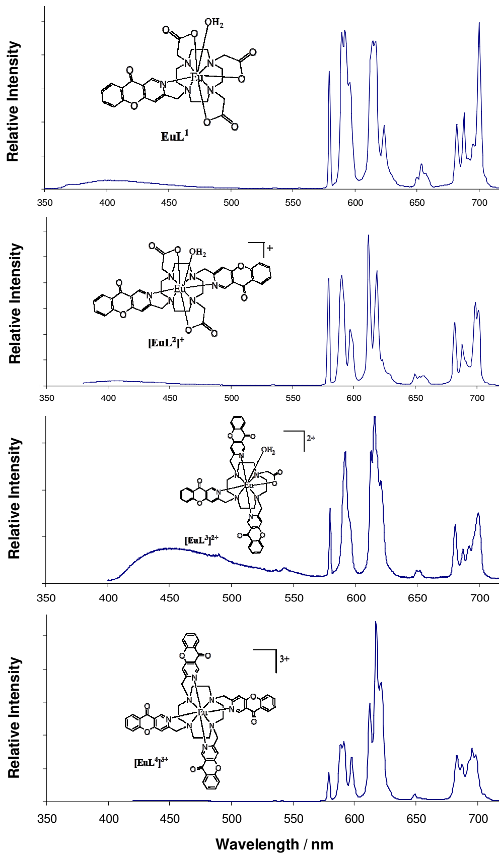
Figure 2.8 Emission spectra of the four europium complexes in water after excitation at 328 nm. Each spectrum was recorded with a complex concentration of 20 \mu M at pH 5.8 and 293 K.
