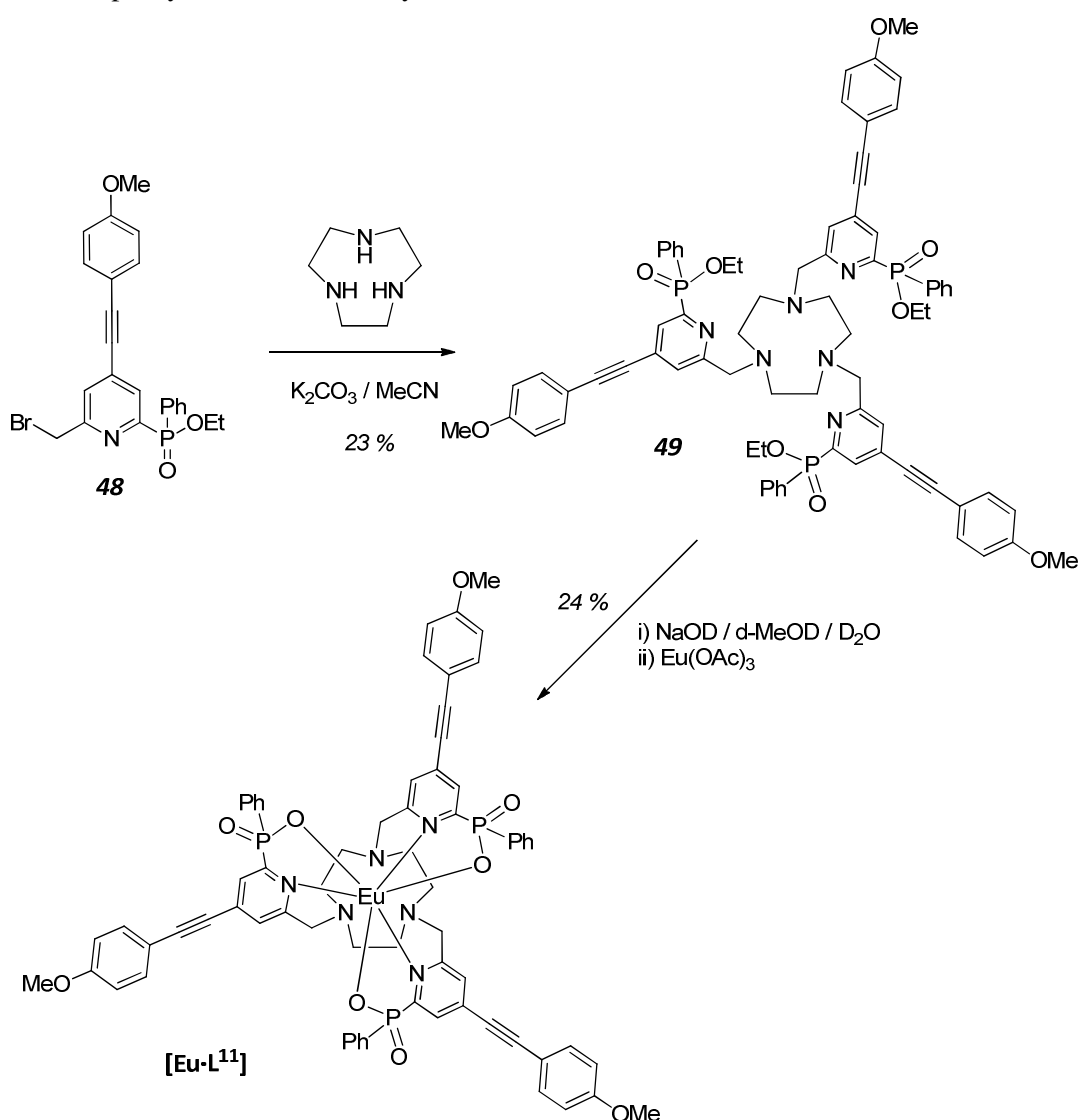
Scheme 5.8
