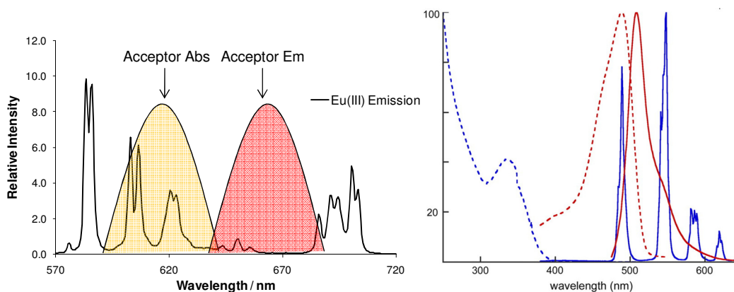
Figure 1.14 Schematics representing the spectral overlap between left ) the donor emission of [\text{Eu}\cdot\text{L}^{1.1}]^{3+} and an allophycocyanin dye and right ) the donor emission [\text{Tb}\cdot\text{L}^{1.13}]^+ (blue solid line) and the acceptor EGFP (absorption – red dashed line, emission – red solid line).
