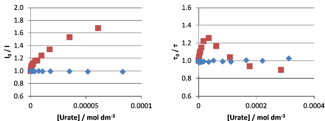
Figure 6.10 Variations in the total integrated emission, I_0/I (left) and excited state lifetime \tau_0/\tau (right) for [\text{Eu}\cdot\text{L}^{12}] (blue) and [\text{Eu}\cdot\text{L}^{13}(\text{H}_2\text{O})]^+ (red) as a function of added urate.
