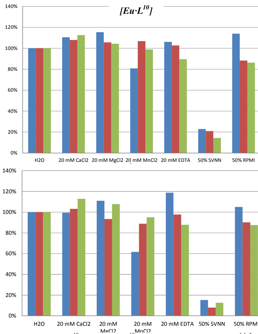
c) Stability assay for [Eu \cdot L^{10}] (blue), [Eu \cdot L^{10}] in 0.4 M KF (red) and [Eu \cdot L^{1.1}]^{3+} (green) after 10 min (upper) and 18 h (lower) (10nM complex, 20mM additive, \lambda_{ex} = 335 nm, \lambda_{ex} = 620 nm).
