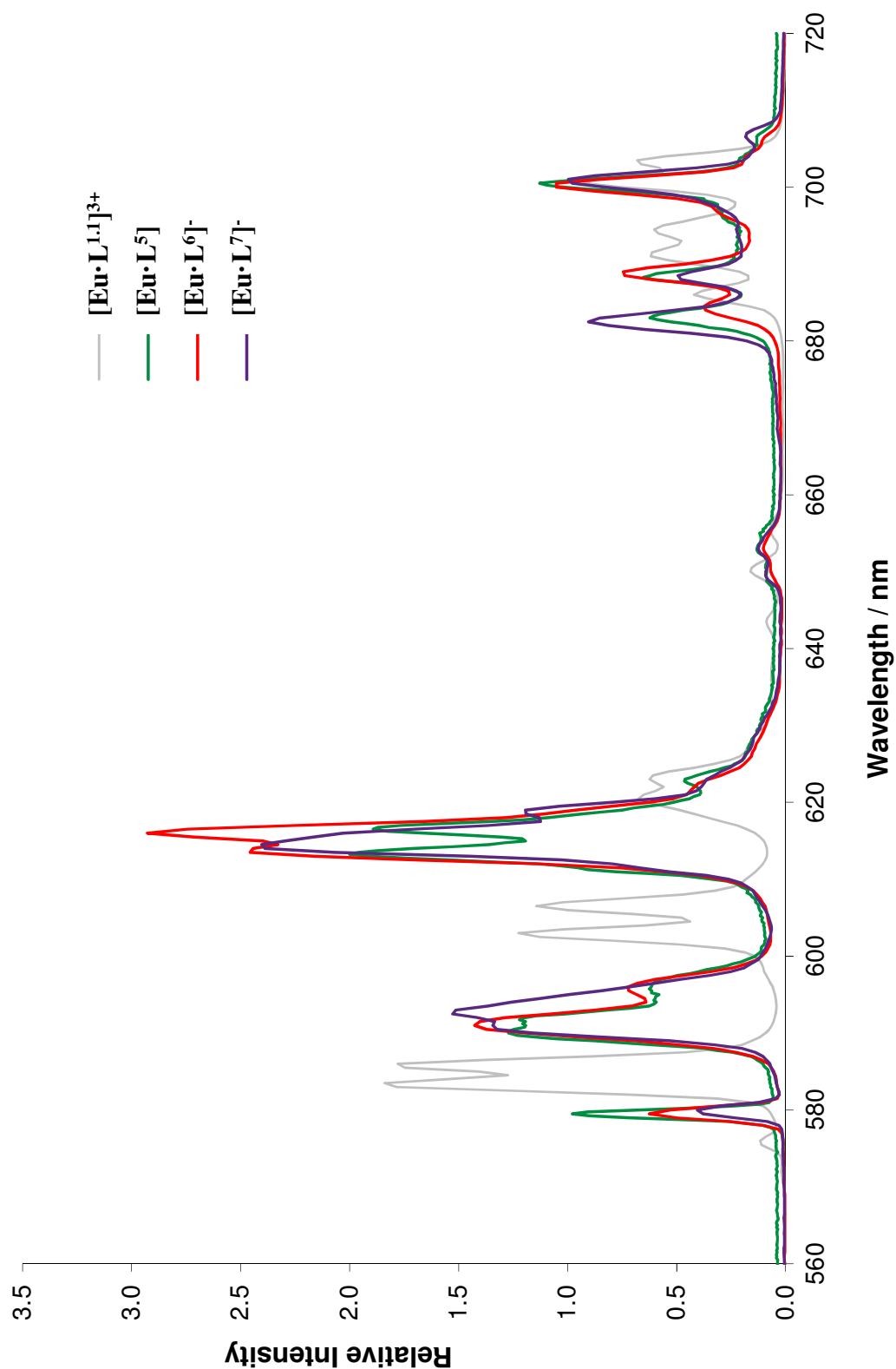
Figure 3.3 Comparison of the emission spectra of [\text{Eu}\cdot\text{L}^5] (purple), [\text{Eu}\cdot\text{L}^6]^- (red) and [\text{Eu}\cdot\text{L}^7]^- (green). The emission spectrum of the tris(bipyridine) complex [\text{Eu}\cdot\text{L}^{11}]^{3+} (grey) is also shown. All spectra recorded in \text{H}_2\text{O} ( 20\ \mu\text{M} complex, pH 5.8, 295 K) except [\text{Eu}\cdot\text{L}^{11}]^{3+} which also contains 0.4 M KF. Spectra have been scaled so that the total integrated intensity is equal for each spectrum.
