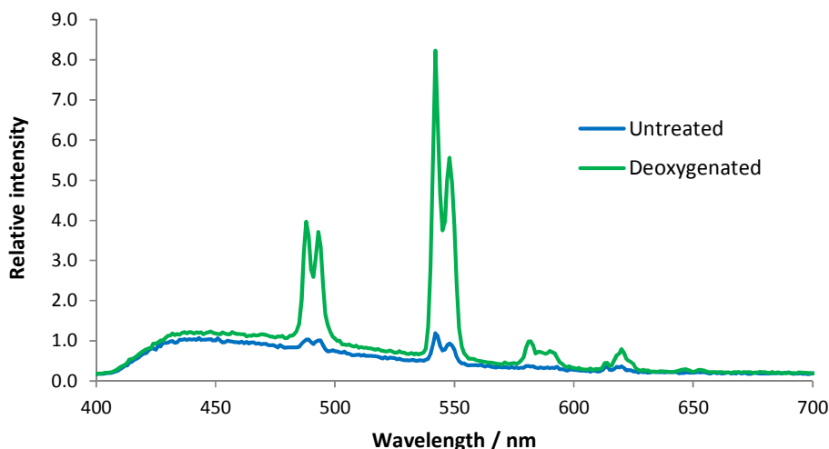
Figure 5.10 Emission spectrum for [\text{Tb}\cdot\text{L}^{11}] prior to (blue) and after (green) bubbling argon through the solution for 30 s (MeOH, \lambda_{\text{ex}} = 332 nm, 295 K).
