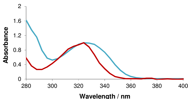
Figure 2.6 Absorption spectra of [\text{Eu}\cdot\text{L}^1(\text{H}_2\text{O})] in H 2 O (blue) and 2-methyl-3-azaxanthone in MeOH (red), showing a red shift of 4 nm in the maximum absorption wavelength.
