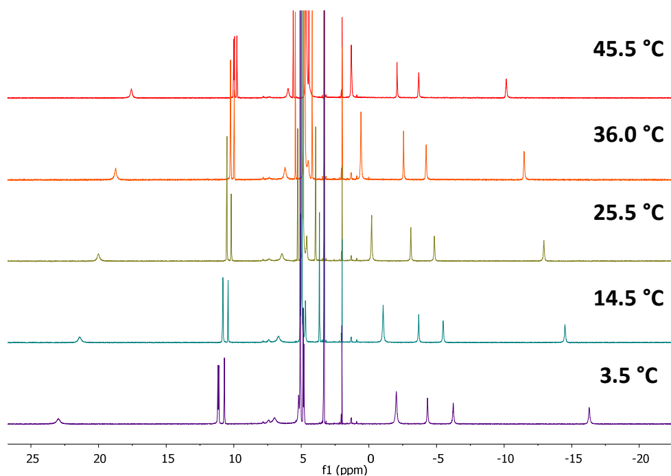
Figure 4.7 Variable temperature ^1\text{H} -NMR spectrum of [\text{Yb}\cdot\text{L}^9] ( \text{CD}_3\text{OD} , 500 MHz, pD 5.8).
