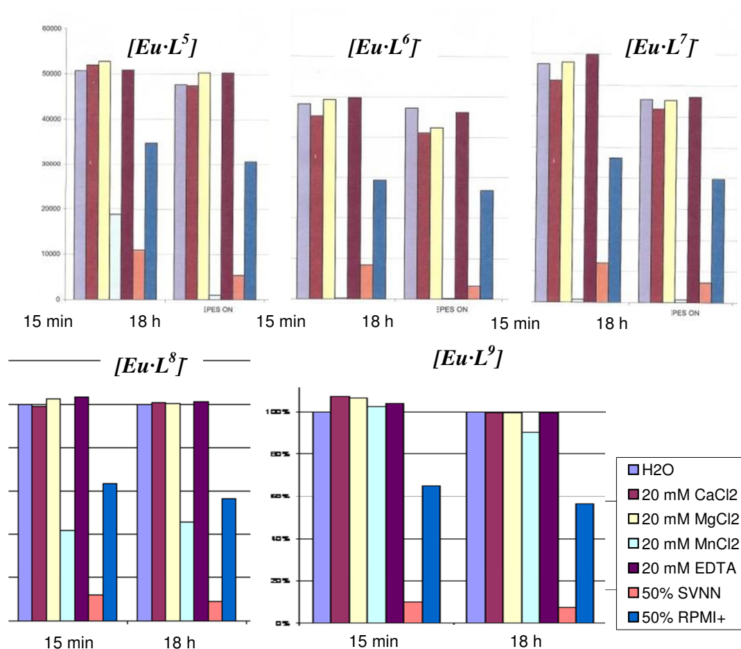
b) Changes in Eu 3+ emission intensity after 15 min or 18 h in the presence of the stated additives (10nM complex, 20mM additive, λ ex = 335 nm, λ em = 620 nm).
