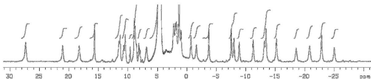
Figure 2.3 ^1\text{H-NMR} analysis of [\text{Eu}\cdot\text{L}^2(\text{H}_2\text{O})]\text{Cl} (400 MHz, \text{D}_2\text{O} , pD 5.8).
