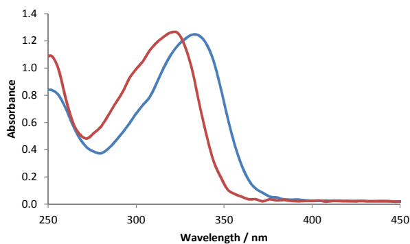
Figure 5.5 Absorption spectra for the alkynyl chromophore 43 (red) and [\text{Eu}\cdot\text{L}^{11}] (blue), which incorporates the same chromophore (MeOH, 295 K).
