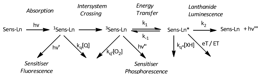
Scheme 6.1
