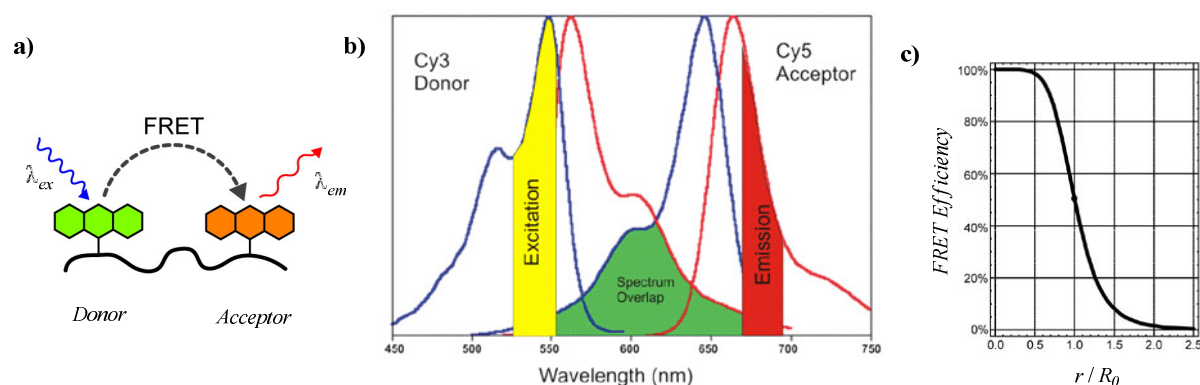
Figure 1.10 a) Schematic showing FRET between a donor and an acceptor, b) the excitation ( blue ) and emission ( red ) spectra of two cyanine dyes. The spectral overlap integral is highlighted in green. The yellow and red highlighted areas illustrate suitable wavelengths to excite the donor and measure acceptor emission, respectively and c) FRET efficiency as a function of r/R_0 .
