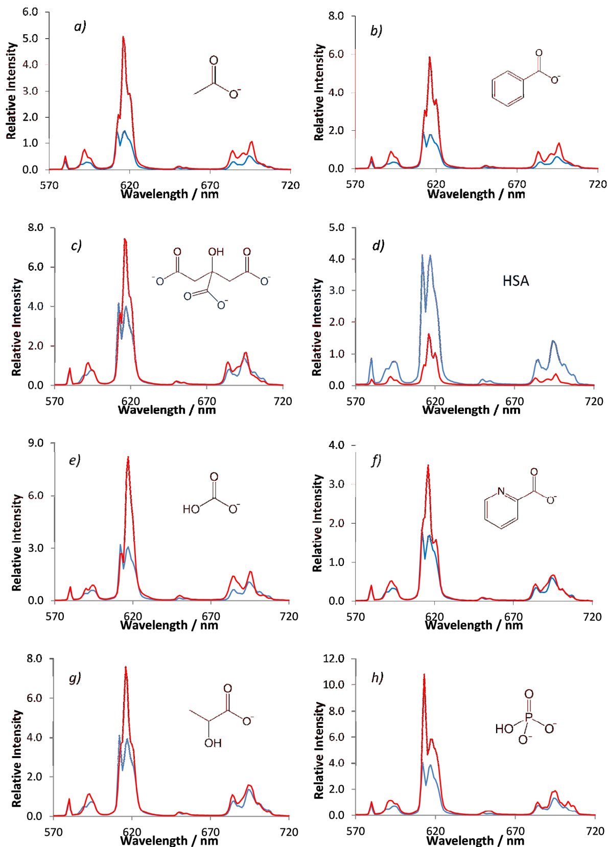
Figure 5.14 Limiting emission spectra for [\text{Eu}\cdot\text{L}^{13}(\text{H}_2\text{O})]^+ in the presence of an excess of anions or HSA (red). The emission spectrum in the absence of additive is also shown (blue). Each spectrum was recorded in \text{H}_2\text{O} : \text{CH}_3\text{OH} (3 : 1, \lambda_{\text{ex}} = 332 nm, pH 7.4, 295 K). The selected anions are a) acetate, b) benzoate, c) citrate, e) bicarbonate, f) picolinate, g) lactate and h) hydrogen phosphate as their \text{Na}^+ salts.
