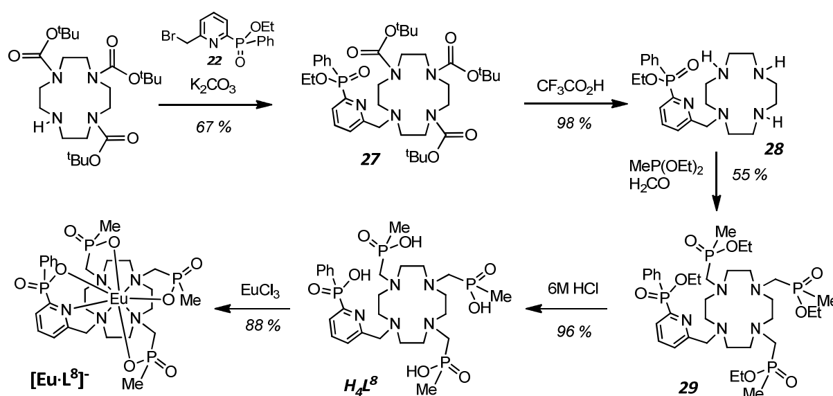
Scheme 3.5
