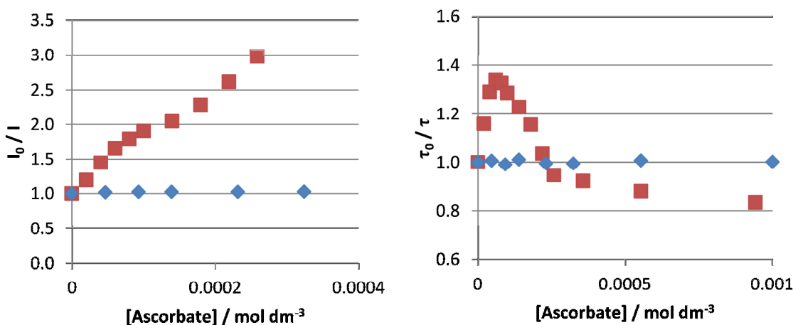
Figure 6.8 Variations in the total integrated emission, I_0 / I (left) and excited state lifetime \tau_0 / \tau (right) for [\text{Eu}\cdot\text{L}^{12}] (blue) and [\text{Eu}\cdot\text{L}^{13}(\text{H}_2\text{O})]^+ (red) as a function of added ascorbate.
