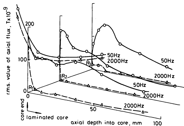
Fig. 14 Axial-flux distribution in laminated stator core Helical winding; radius = 0.87 R_f (143 mm); overhang = 0 (0 mm)
