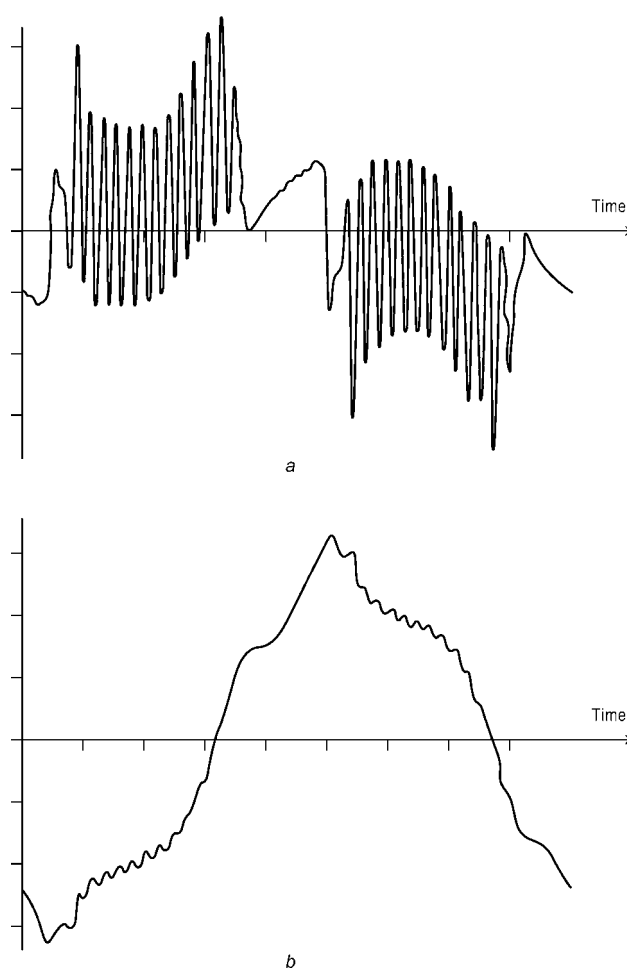
Figure 12 Typical voltage and flux waveforms obtained from a generator airgap search coil
