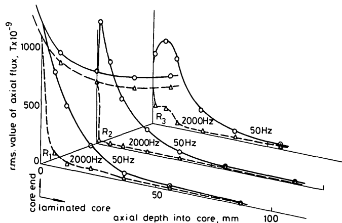
Fig. 10 Axial-flux distribution in laminated stator core Diamond winding; radius = 0.97 R_f (160 mm); overhang = 1.11 R_f (183 mm)
