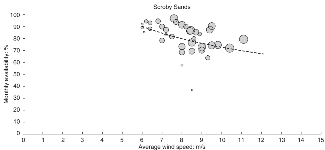
Figure 14. Monthly availability against wind speed for Scroby Sands offshore wind farm (each circle representing 1 month's operational data; circle radius is proportionate to capacity factor)
