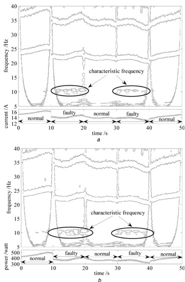
Figure 11 CWTs of the electrical signals
