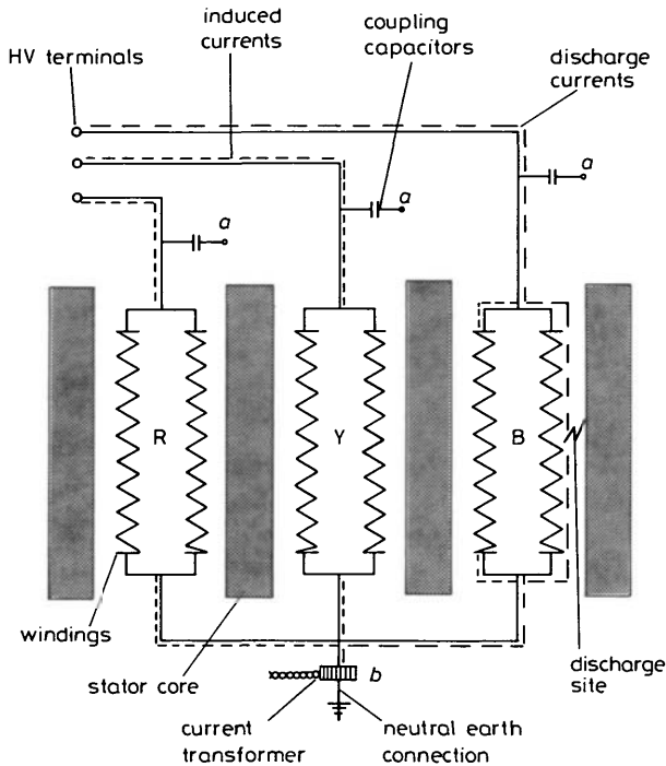
Fig. 1 Schematic diagram of generator stator winding
