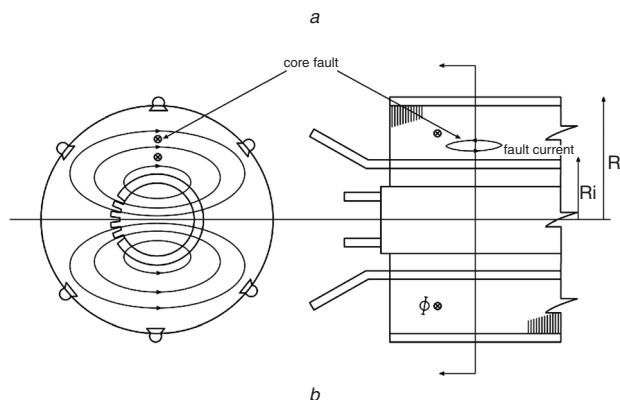
Fig. 1 Laminated core with core fault
