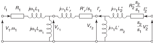
Fig. 10 Referred per-phase equivalent circuit
