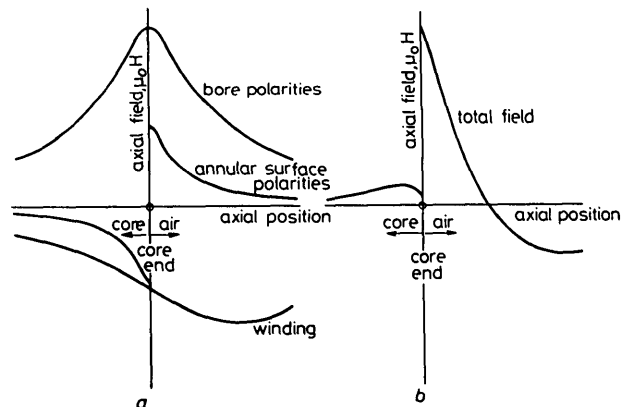
Fig. 7 Superposition of component fields due to the sources
