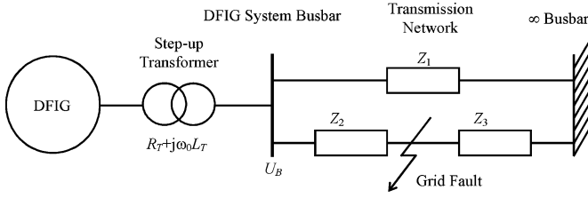
Fig. 14. Configuration of a simulated 2-MW DFIG system.
