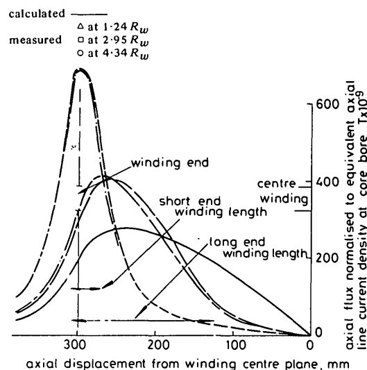
Fig. 4 Comparison between calculated values of axial flux density for three types of winding with various lengths of end winding
