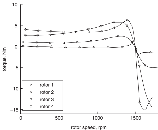
Fig. 4 Measured torque-speed characteristic Four-pole stator supplied with 90 V_{rms} Eight-pole stator open circuit (simple induction mode)
