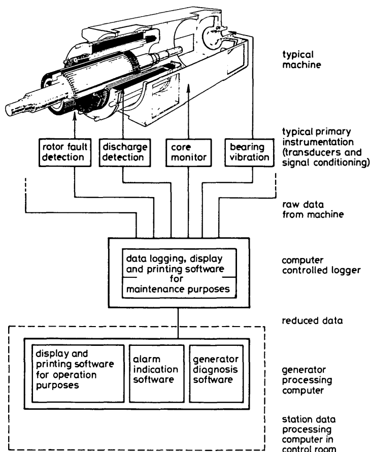
Fig. 8 Comprehensive monitoring scheme for a typical electrical machine Reproduced from Reference 37
