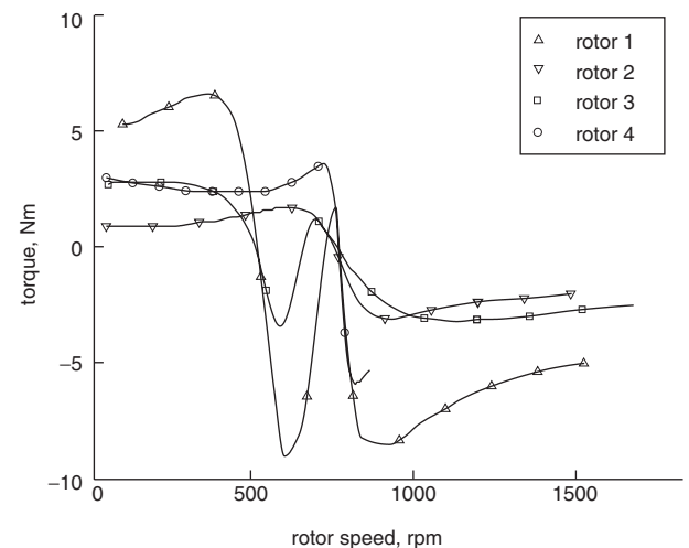
Fig. 7 Measured torque-speed characteristic Eight-pole stator supplied with 90 V_{rms} Four-pole stator short circuited (cascade induction mode)
