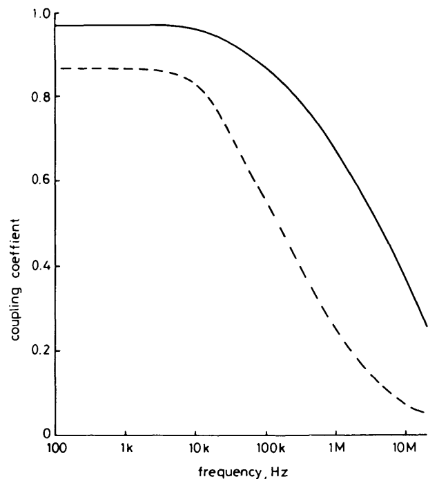
Fig. 12 Calculated variation of coupling coefficient across large turbo-generator stator core
