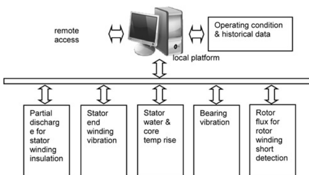
Figure 18 Configuration of a modular expert system for a large turbogenerator
