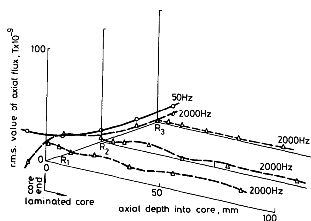
Fig. 19 Axial-flux distribution in laminated stator core
