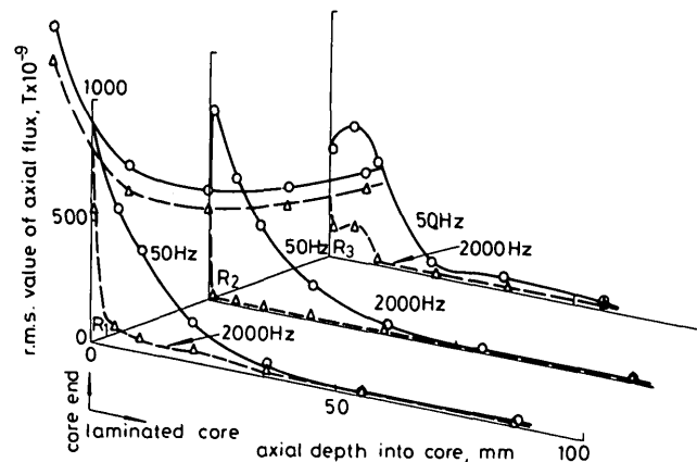
Fig. 11 Axial-flux distribution in laminated stator core Helical winding; radius = 0.87 R_f (143 mm); overhang = 1.11 R_f (183 mm)
