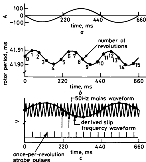
Fig. 2 Motor speed fluctuation waveforms
