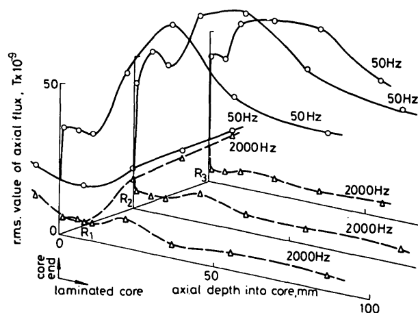
Fig. 15 Axial-flux distribution in laminated stator core Concentric winding; radius = 0.61 R_f (100 mm); overhang = 0 (0 mm)
