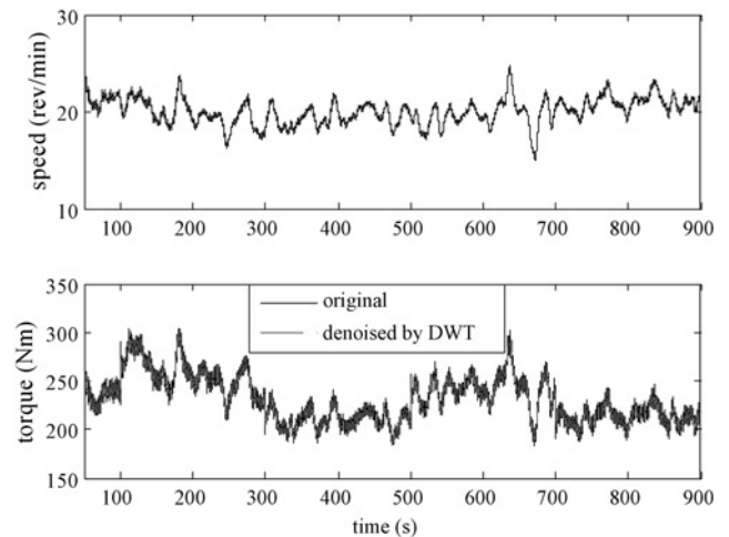
Figure 6 Shaft rotational speed and mechanical torque signals
