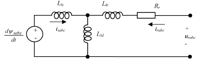
Fig. 2. Rotor-side equivalent circuit.
