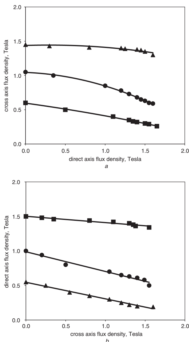
Fig. 14 Cross-magnetisation characteristics on a laminated core-plate steel sample
