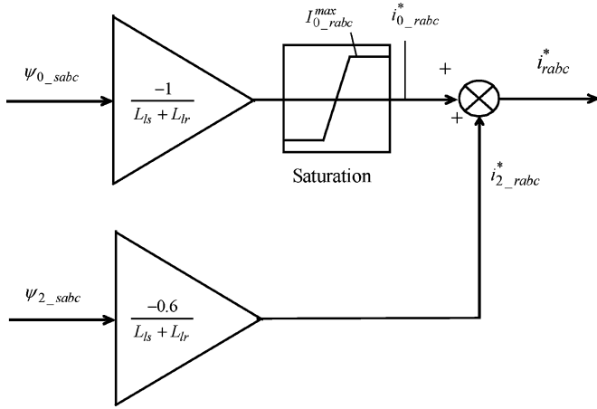
Fig. 8. Sharing of converter current capability.
