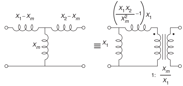
Fig. 15 Equivalent forms of 'T' and 'T' networks
