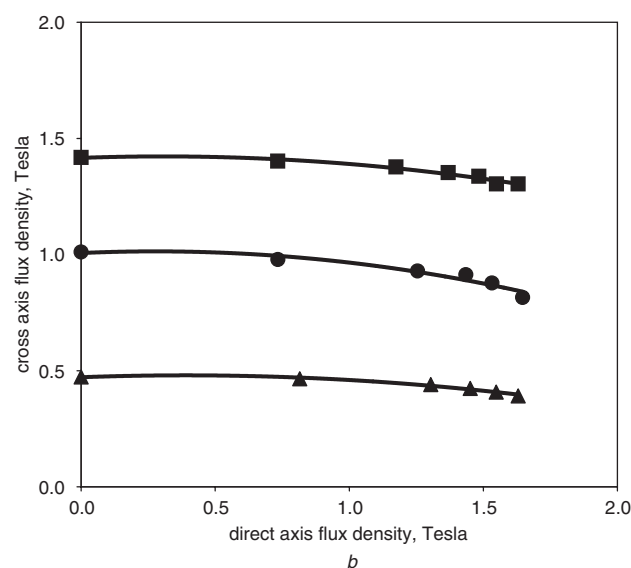
Fig. 13 Cross-magnetisation characteristics on an isotropic mild steel sample
