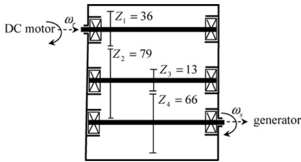
Figure 14 Diagram of the gearbox used in the drive train of the wind turbine
