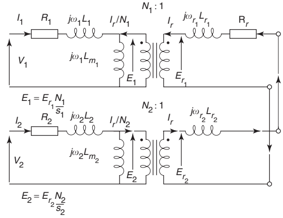
Fig. 9 BDFM per-phase equivalent circuit
