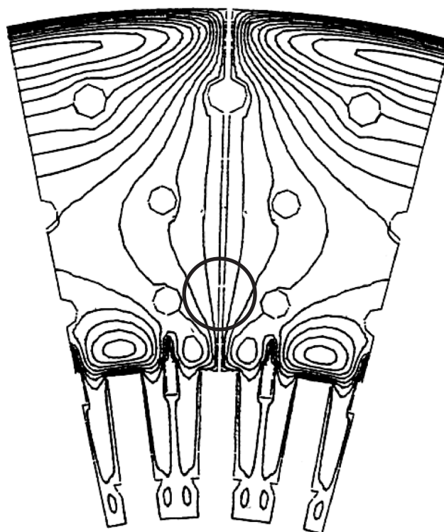
Fig. 8 Plot of eddy currents in the plane of lamination segments at the quadrature axis
