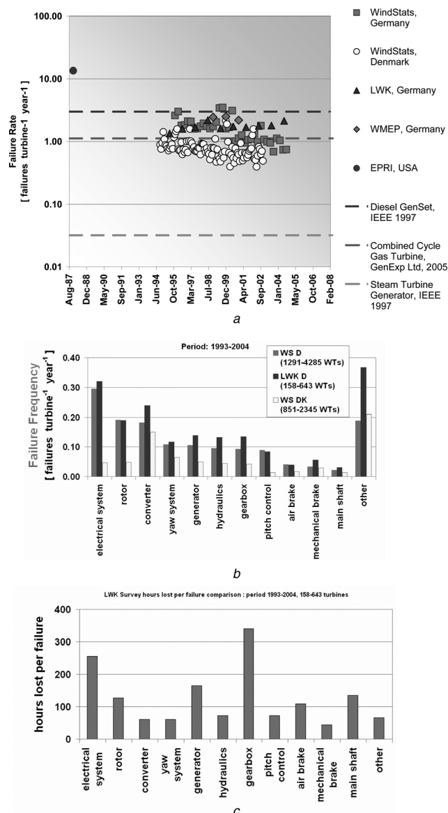
Figure 4 Results from surveys assuming a constant failure rate and the HPP model
