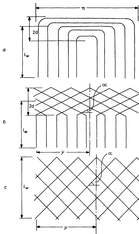
Fig. 1 Developed schematics of windings investigated
