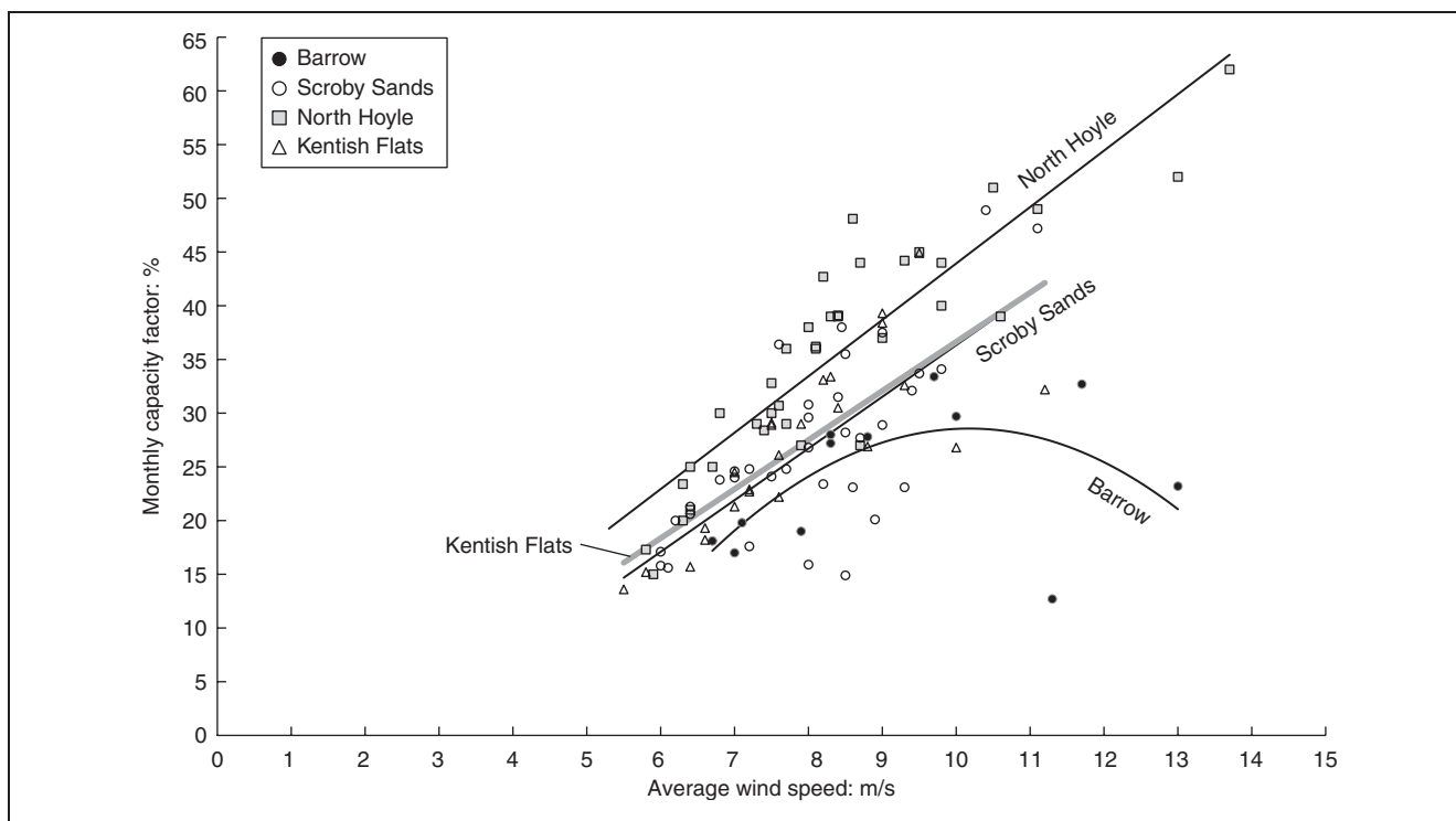
Figure 11. Monthly capacity factor against wind speed for the offshore wind farms
