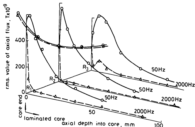
Fig. 12 Axial-flux distribution in laminated stator core Concentric winding; radius = 0.61 R_f (100 mm); overhang = 0.64 R_f (105 mm)
