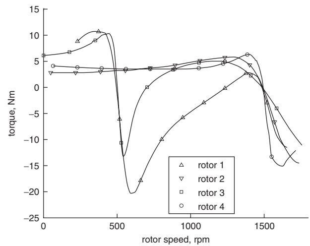
Fig. 6 Measured torque-speed characteristic Four-pole stator supplied with 90 V_{rms} Eight-pole stator open circuited (cascade induction mode)
