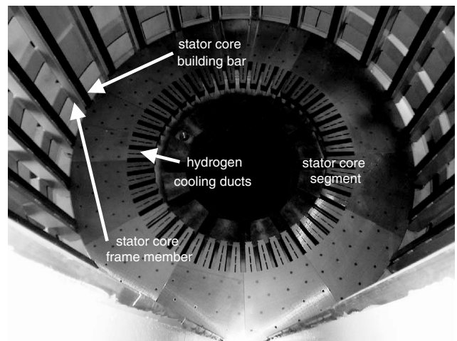
Fig. 2 Laminated stator core of a 500 MW, 2 pole hydrogen-cooled turbogenerator under construction
