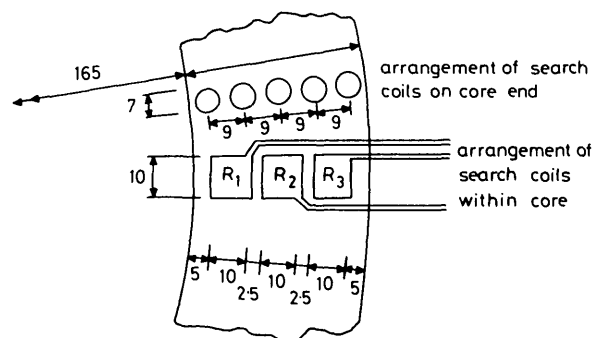
Fig. 7 Layout of axial search coils on core end and within the core
