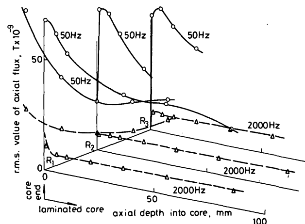
Fig. 16 Axial-flux distribution in laminated stator core
