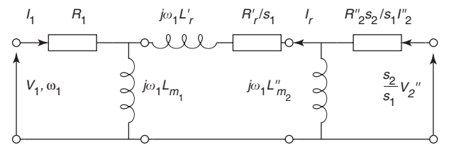
Fig. 11 Simplified per-phase equivalent circuit
