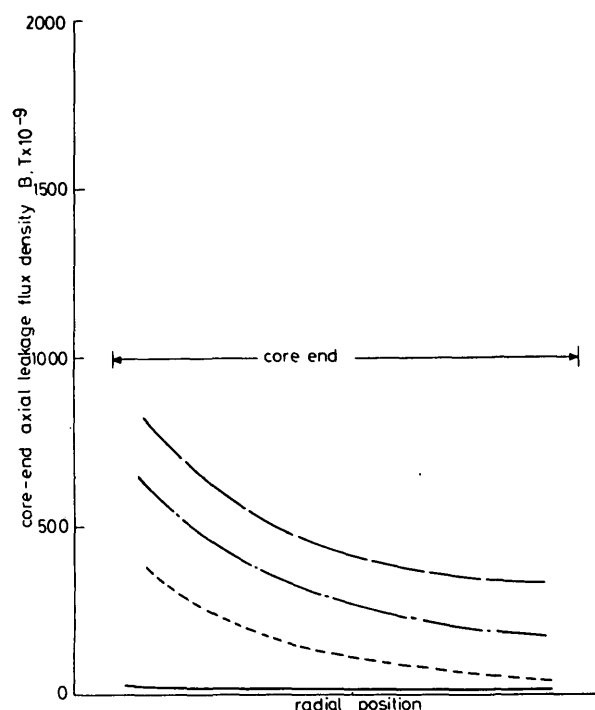
Fig. 9 Core end axial leakage flux density for the concentric winding, radius 0.61 R_t in four overhang positions
