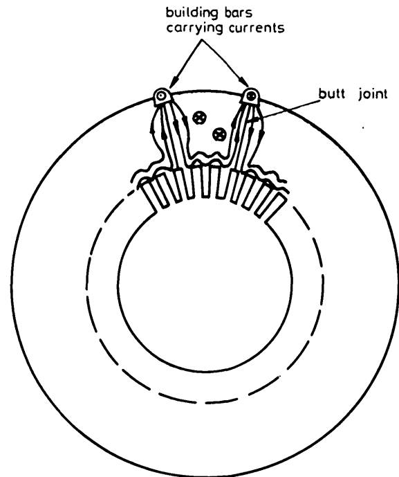
Fig. 5 Possible current route between building bars
