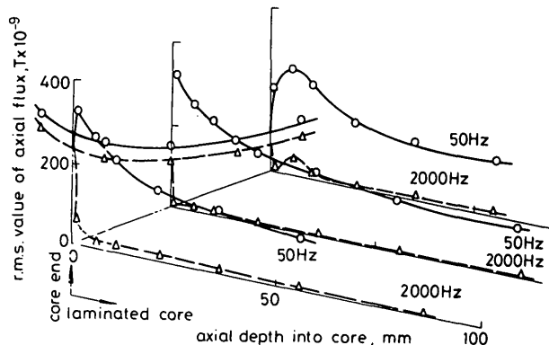
Fig. 13 Axial-flux distribution in laminated stator core Concentric winding; radius = 0.36 R_f (60 mm); overhang = 0.64 R_f (105 mm)
