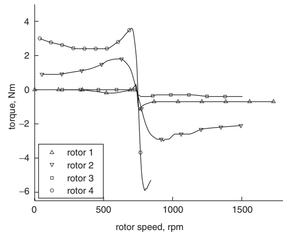
Fig. 5 Measured torque-speed characteristic Eight-pole stator supplied with 90 V_{rms} Four-pole stator open circuited (simple induction mode)
