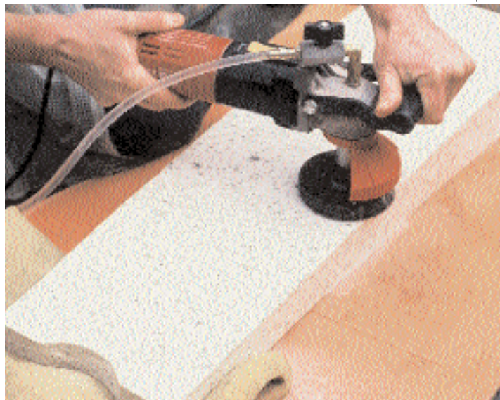
Grinding tall standing form, using Electra-Flex angle grinder.
