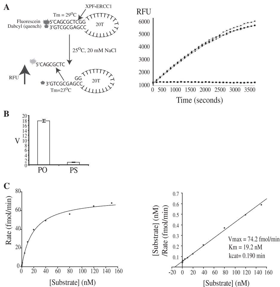
Figure 2. A microplate fluorescence-based assay to measure XPF-ERCC1 incision activity. (A) Left panel: principle of the fluorescence-based assay. RFU is relative fluorescence units. Incubation of intact stem-loop with XPF-ERCC1 in 0.75 mM \text{MnCl}_2 and 20 mM NaCl results in the cleaved oligonucleotide diffusing into solution at 25°C. Right panel: increase in fluorescence (RFU) with time. Reactions are shown in triplicate and contained: 3 nM XPF-ERCC1, 100 nM standard stem-loop substrate, 0.75 mM \text{MnCl}_2 , 0.5 mM DTT and 20 mM NaCl in 50 mM Tris buffer pH 8 at 25°C. Solid squares: buffer only (B) Graph showing rate of incisions (v) of 62.5 nM stem-loop by 3 nM XPF-ERCC1 where the scissile phosphate contains non-bridging oxygens (PO) or a non-bridging sulphur (PS). Average of three points \pm SD. (C) Left panel: Michaelis-Menten plot showing rate versus substrate concentration for full-length XPF-ERCC1. Mean of three points. Right panel: Hanes-Woolf plot.
