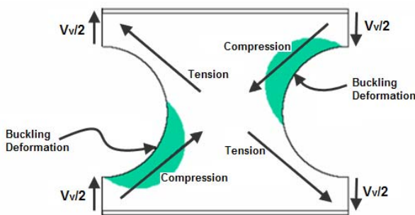
Fig. 7: Typical web-post behaviour
