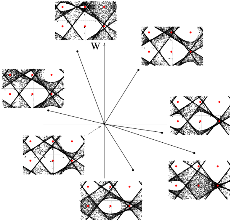
Figure 26: By plotting the algebra projection of the curve P(z, w) = W we see that near the critical points W_* the algebra fills in the region of the vanishing cycle (critical values of z, w , marked with red dots). Thus, the vanishing cycles sweep out the faces of the dimer model shown in Figure 25.
