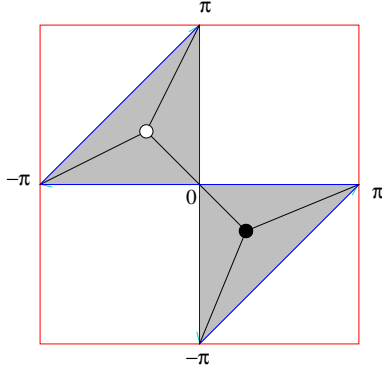
Figure 19: An embedding of the dimer model for \mathbb{C}^3 . The shaded region is the algebra projection of the curve P(z, w) = 1 - z - w = 0 , and in this case it is bounded by the straight-line winding cycles with (p, q) = (1, 1), (-1, 0), (0, -1) .
