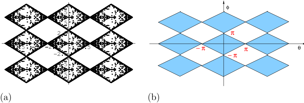
Figure 16: (a) The algebra of F_0 (cf. Figure 15) drawn using Monte-Carlo and redrawn in (b) to show the boundaries more clearly. We have indicated 3 \times 3 of the fundamental region to show the periodicity. Not all algebras are as regular as this.
