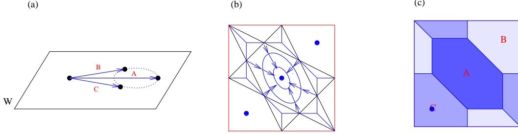
Figure 24: (a) For \mathbb{C}^3/\mathbb{Z}_3 , there are 3 critical points in the W -plane; (b) The algebra projection of the critical values of z, w at the critical points of W are in the interior of the three hexagonal faces of the dimer graph. Along the straight-line paths from W = 0 to a critical point, the corresponding face of the dimer model fills in. (c) The combination of these paths fills the entire T^2 in the angular parts of z, w . The S^1 fibre in the u, v plane vanishes over the boundary of each face and is non-vanishing in the interior, which exhibits these faces as the S^3 wrapped branes.
