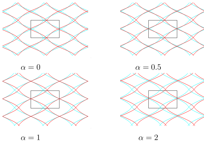
Figure 27: The 4 S^1 's winding the 4 cylinders of F_0 under the algebra projection. We vary the parameter \alpha which represents a complex modulus of \Sigma and see how the intersection varies for 4 different values of \alpha as indicated. The fundamental domain [-\pi, \pi] is indicated by the black box.
