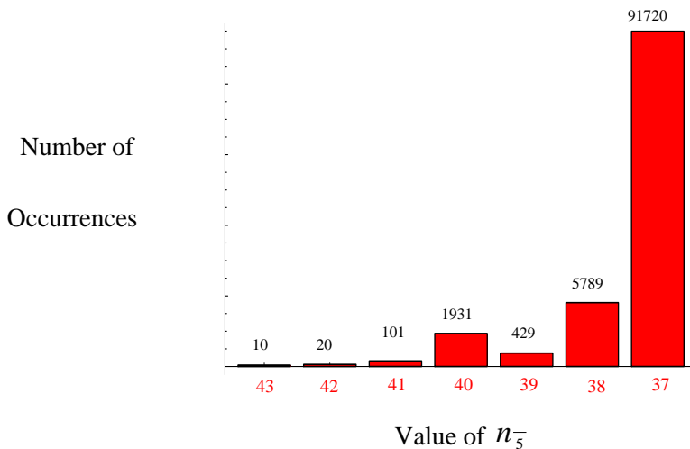
Figure 1: In 100,000 random integer initializations of the matrix M_2 , the numbers of occurrences of the various values of n_{\bar{5}} are plotted. We see that the generic value 37 dominates by far.
