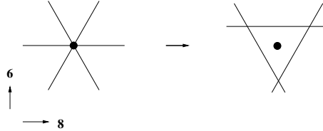
Figure 3: The 8d modulus for k = 3 .
