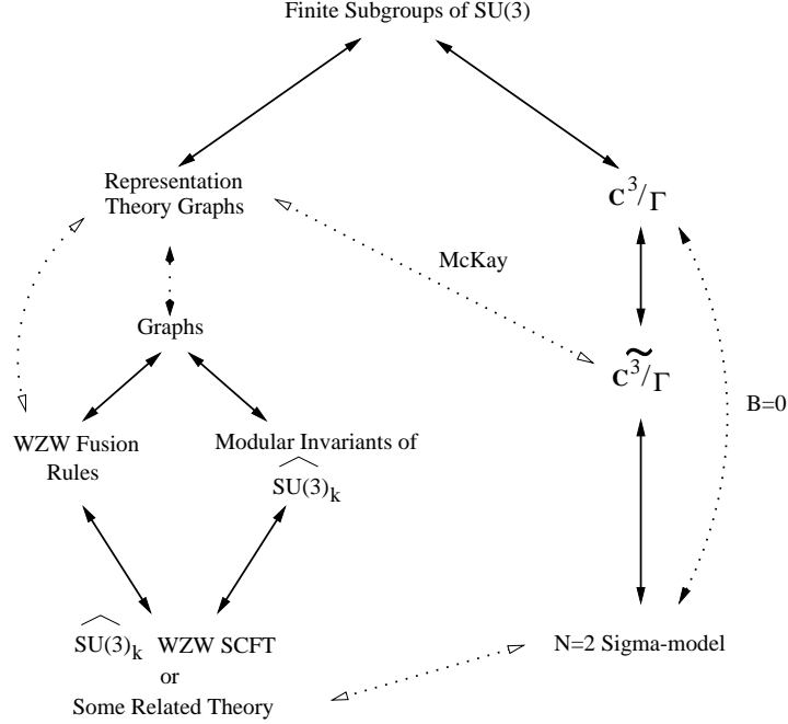
Figure 4: Web of Conjectures: Recently, the graphs from the representation theory side were constructed and were noted to resemble those on WZW \widehat{SU(3)}_k side [1]. The solid lines have been sufficiently well-established while the dotted lines are either conjectural or ill-defined.
