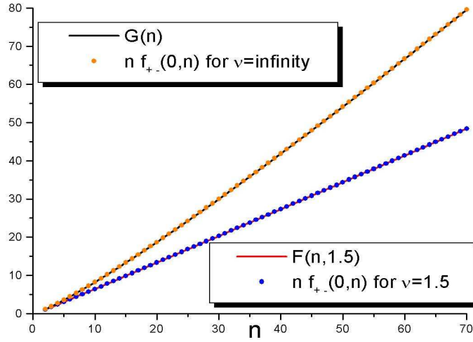
Figure 2: The functions F(n, 1.5) and G(n) and the corresponding values of nf_{+-}(0, n) for 2 \leq n \leq 70 .
