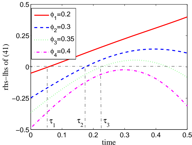
Figure 1: Right hand side(rhs) minus the left hand side(lhs) of equation (41) as a function of time t with fixed values of \varepsilon = 2.5, E = 2, \omega = 4.87 - i3.31 for \phi_1 = 0.2, \lambda_1 = 3.5 ; \phi_2 = 0.3, \lambda_2 = 3.73 + i0.2 ; \phi_3 = 0.35, \lambda_3 = 3.87 + i0.34 ; \phi_4 = 0.4, \lambda_4 = 4.02 + i0.52 . The corresponding passage times \tau are simply taken to be the smallest values of t for which the rhs-lhs=0.
